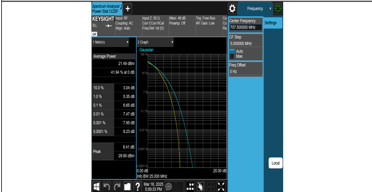
Band12-10MHz-16QAM-23130-1RB#0-PASS
