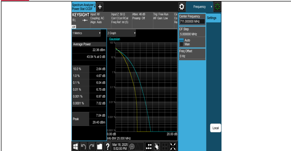
Band12-10MHz-QPSK-23130-50RB#0-PASS
