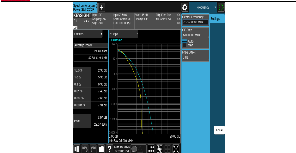
Band12-10MHz-16QAM-23095-27RB#0-PASS
