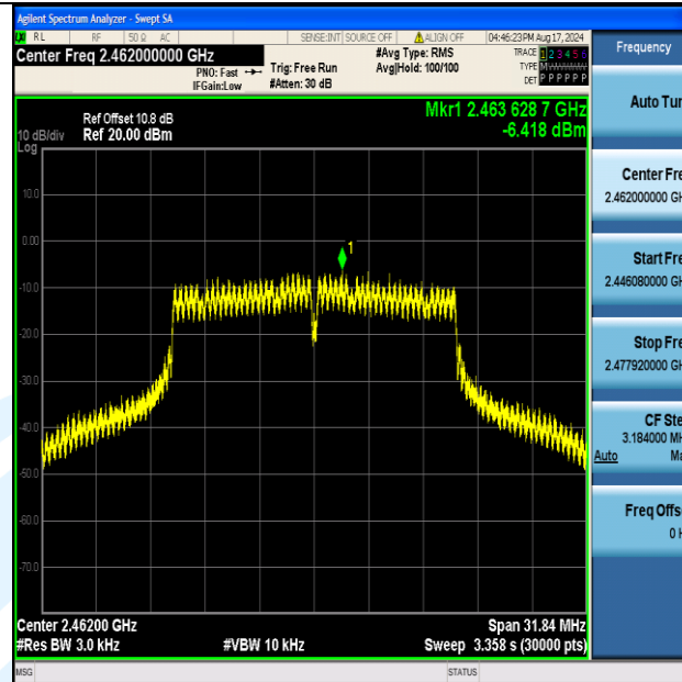
11G-Ant2-2462-PASS
