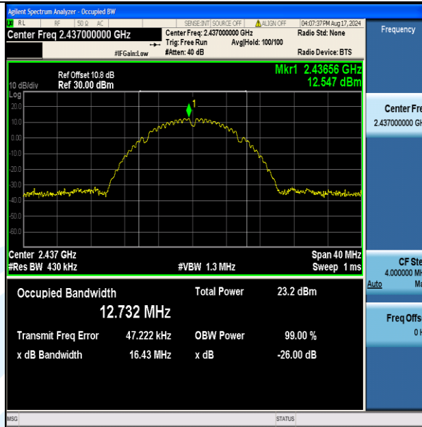
11B-Ant2-2437
