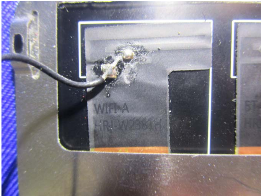
EUT – 5.8G WIFI Antenna View
