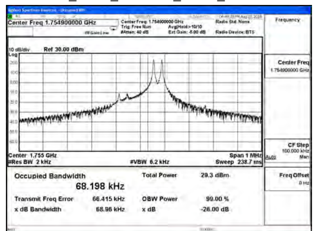
B4_3.75K_CH20399_QPSK_1RB47
