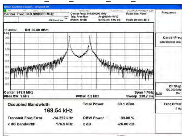
B26_3.75K_CH27039_BPSK_1RB0
