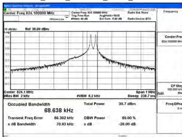
B5_3.75K_CH20401_BPSK_1RB47
