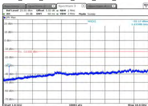
B26_3.75K_CH26915_BPSK_1RB0_above 1G
