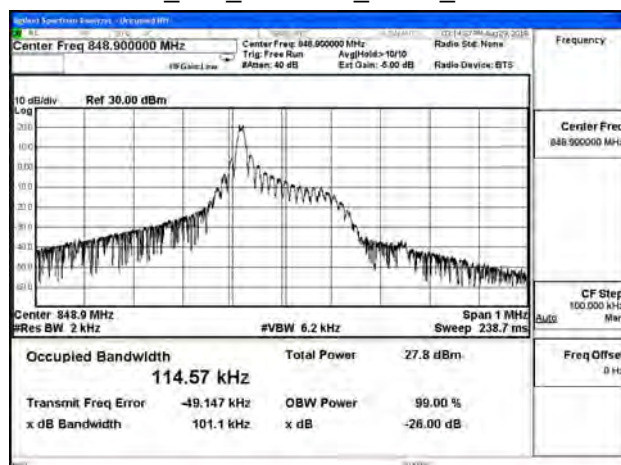
B26_15K_CH27039_BPSK_1RB0
