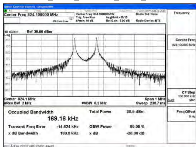
B26_3.75K_CH26791_BPSK_1RB0
