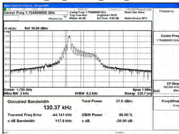
B4_15K_CH20399_QPSK_1RB0
