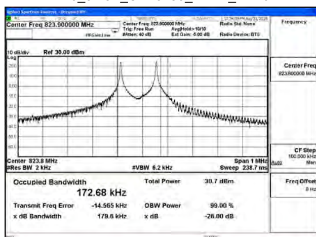
B26_3.75K_CH26788_BPSK_1RB0
