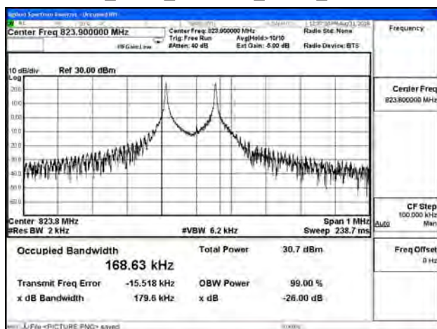
B26_3.75K_CH26788_QPSK_1RB0
