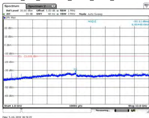
B26_15K_CH26790_QPSK_3RB3_above 1G
