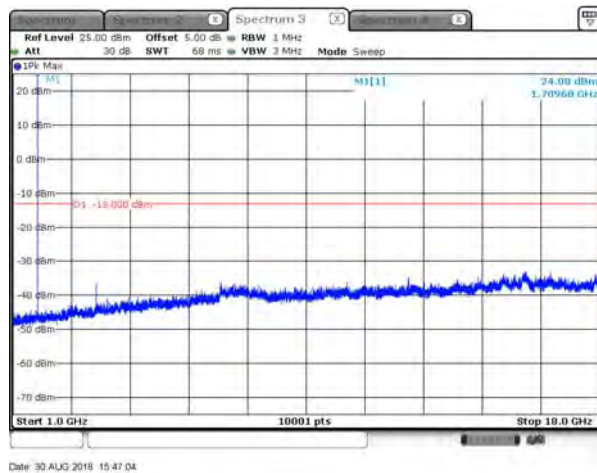
B4_15K_CH20175_QPSK_3RB3_above 1G
