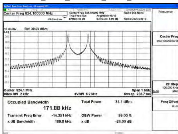
B5_3.75K_CH20401_QPSK_1RB0
