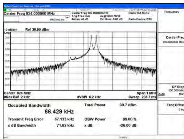
B26_3.75K_CH26790_QPSK_1RB47
