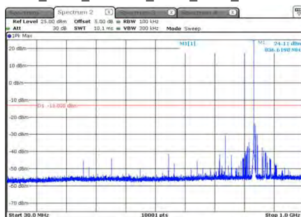
B26_3.75K_CH26915_BPSK_1RB0_under 1G
