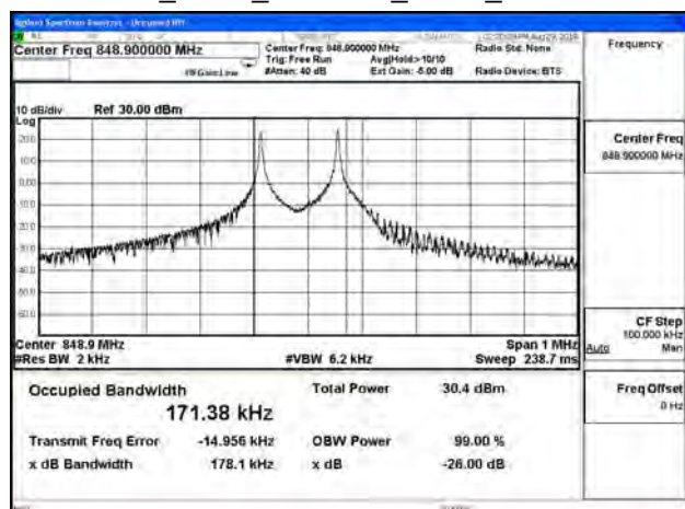
B5_3.75K_CH20649_BPSK_1RB0
