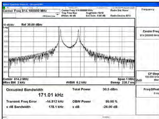
B26_3.75K_CH26692_QPSK_1RB0
