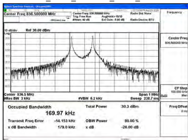
B26_3.75K_CH26915_BPSK_1RB0
