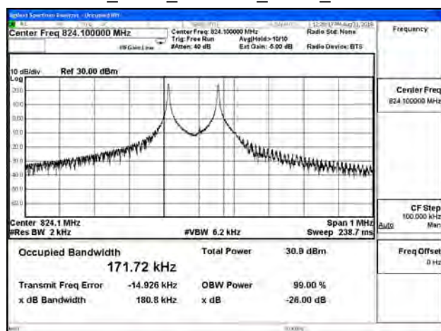
B26_3.75K_CH26791_QPSK_1RB0
