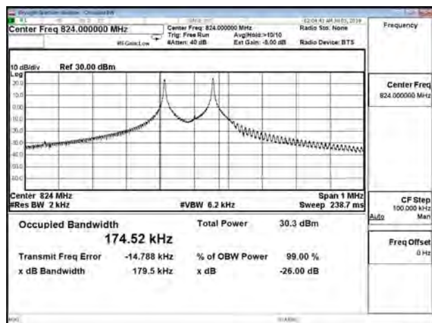
B26_3.75K_CH26790_BPSK_1RB0
