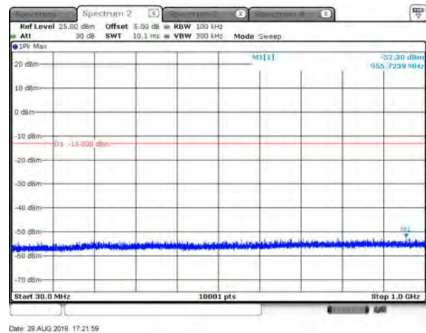
B2_15K_CH18900_QPSK_3RB3_under 1G
