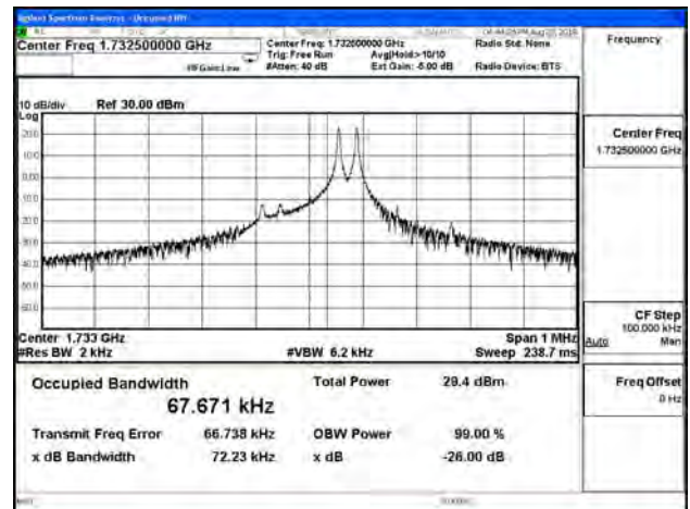
B4_3.75K_CH20175_QPSK_1RB47
