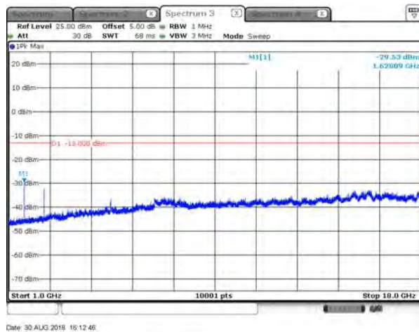
B26_15K_CH26740_QPSK_3RB3_above 1G
