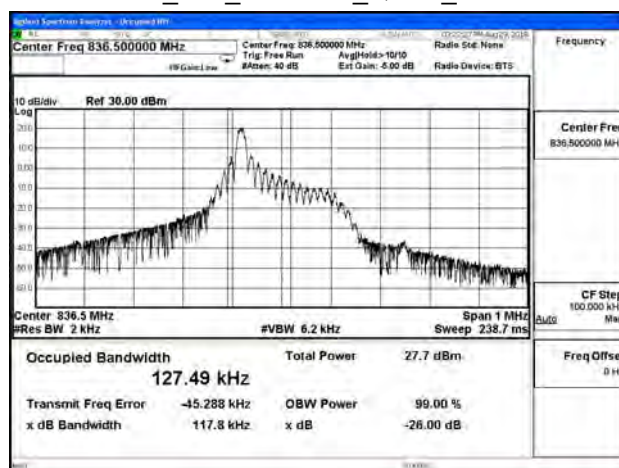
B26_15K_CH26915_QPSK_1RB0
