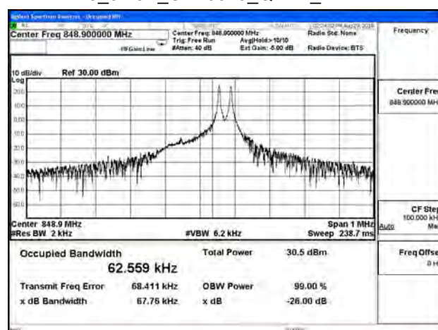
B5_3.75K_CH20649_QPSK_1RB47
