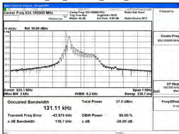
B5_15K_CH20401_BPSK_1RB0
