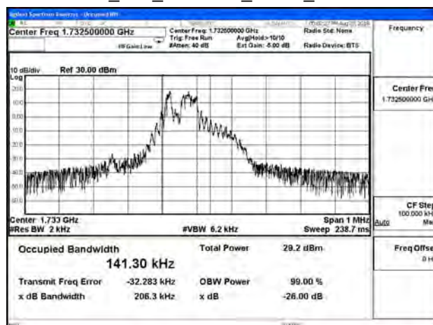
B4_15K_CH20175_QPSK_3RB3
