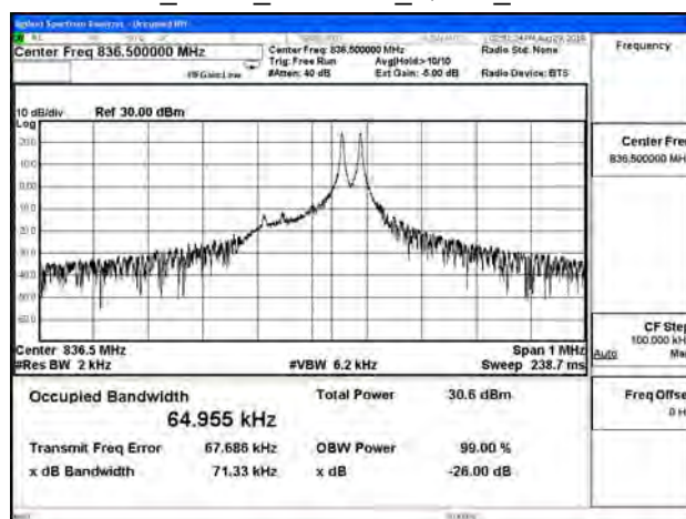
B26_3.75K_CH26915_QPSK_1RB47
