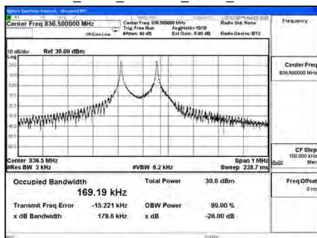
B5_3.75K_CH20525_QPSK_1RB0
