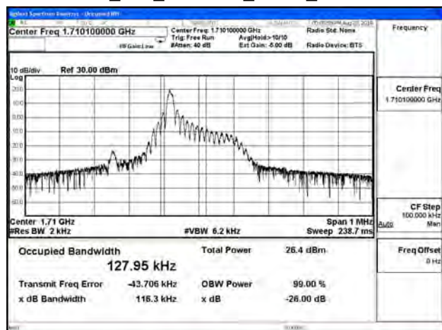
B4_15K_CH19951_QPSK_1RB0
