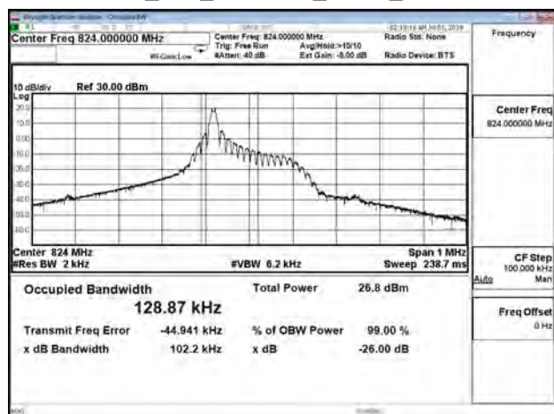
B26_15K_CH26790_BPSK_1RB0
