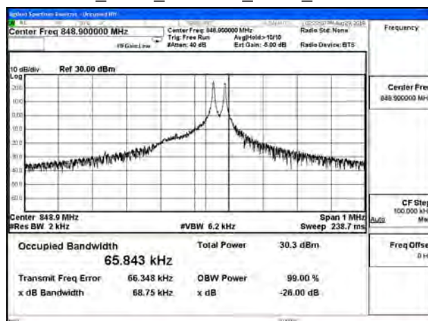
B5_3.75K_CH20649_BPSK_1RB47
