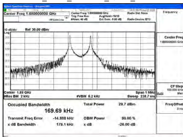
B2_3.75K_CH18900_QPSK_1RB0
