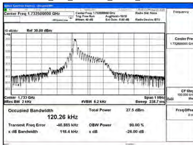
B4_15K_CH20175_QPSK_1RB0
