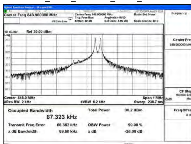
B26_3.75K_CH27039_BPSK_1RB47
