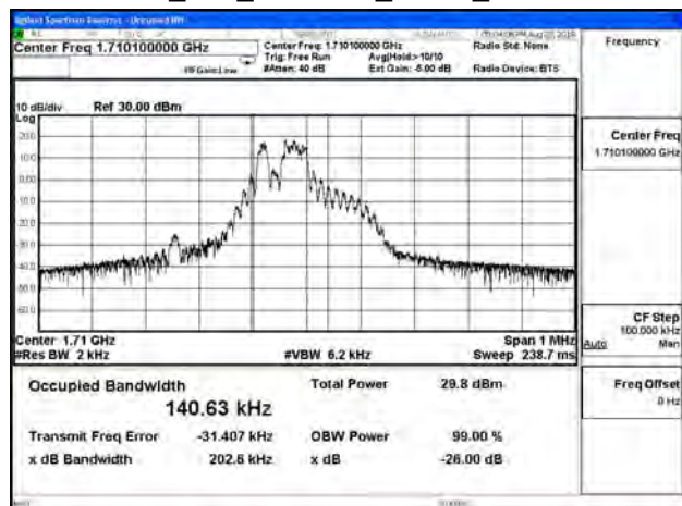
B4_15K_CH19951_QPSK_3RB3
