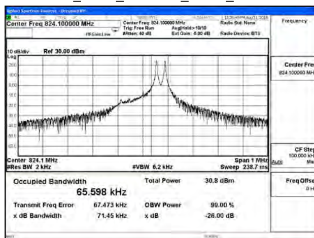
B26_3.75K_CH26791_QPSK_1RB47
