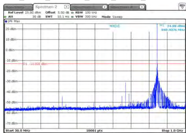
B5_3.75K_CH20649_BPSK_1RB47_under 1G
