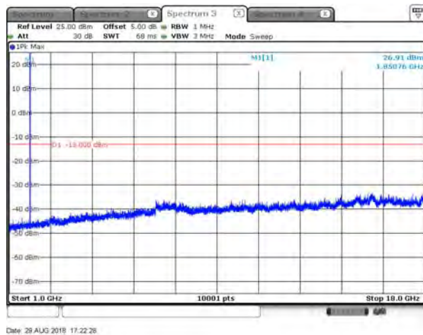
B2_15K_CH18900_QPSK_3RB3_above 1G
