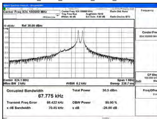
B26_3.75K_CH26791_BPSK_1RB47
