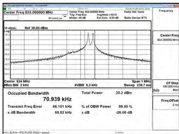
B26_3.75K_CH26790_BPSK_1RB47
