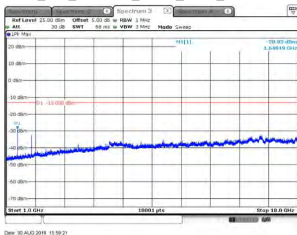
B5_15K_CH20525_QPSK_3RB3_above 1G
