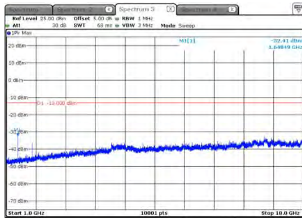
B5_3.75K_CH20401_BPSK_1RB0_above 1G
