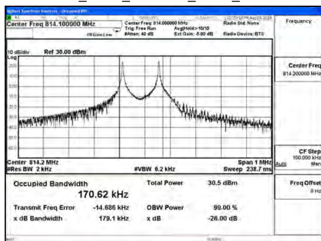
B26_3.75K_CH26692_BPSK_1RB0
