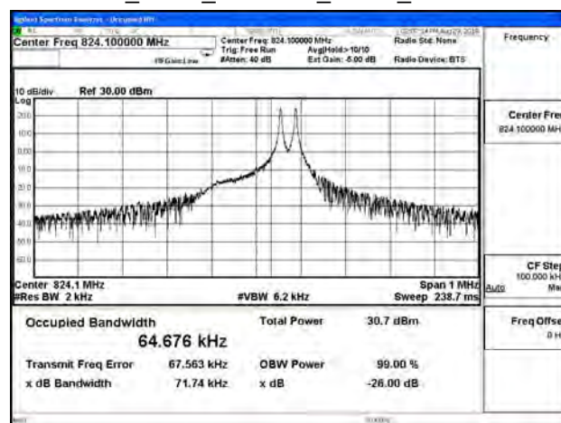
B5_3.75K_CH20401_QPSK_1RB47
