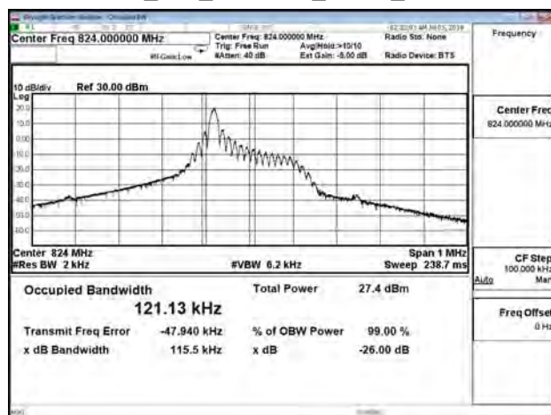
B26_15K_CH26790_QPSK_1RB0
