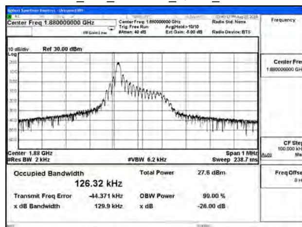
B2_15K_CH18900_QPSK_1RB0
