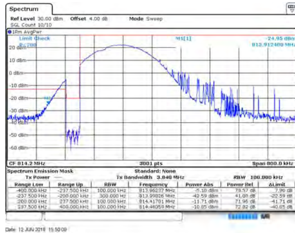
B26_15K_CH26692_QPSK_1RB0
