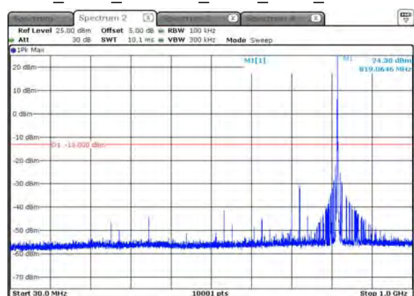
B26_3.75K_CH26740_BPSK_1RB0_under 1G
