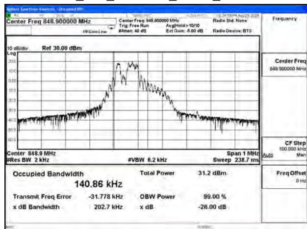
B5_15K_CH20649_QPSK_3RB3
