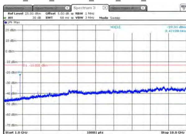
B26_3.75K_CH26788_BPSK_1RB0_above 1G
