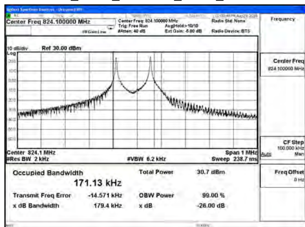
B5_3.75K_CH20401_BPSK_1RB0
