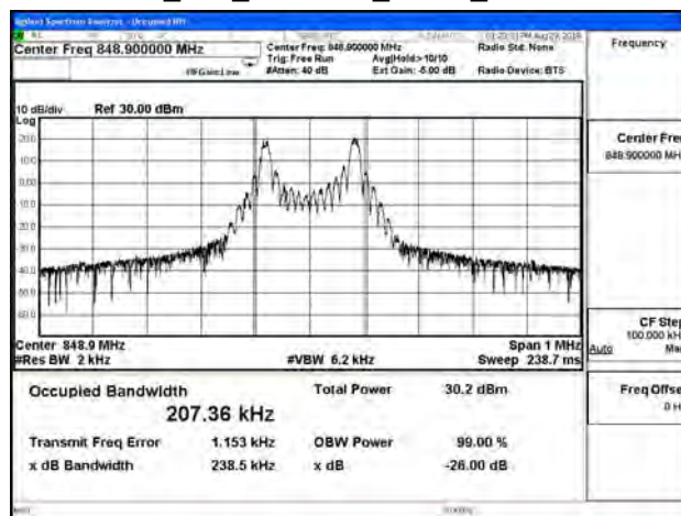
B5_15K_CH20649_QPSK_1RB11
