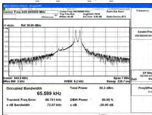
B26_3.75K_CH27039_QPSK_1RB47
