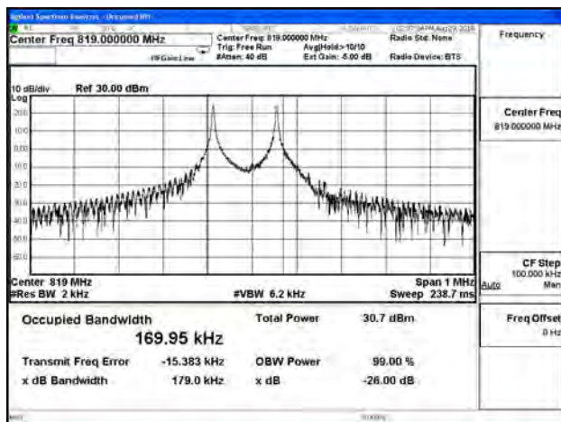
B26_3.75K_CH26740_QPSK_1RB0
