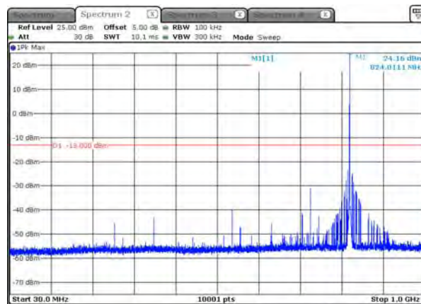
B26_3.75K_CH26790_BPSK_1RB0_under 1G
