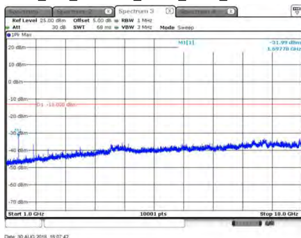
B5_15K_CH20649_QPSK_3RB3_above 1G
