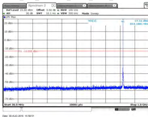
B5_15K_CH20525_QPSK_3RB3_under 1G
