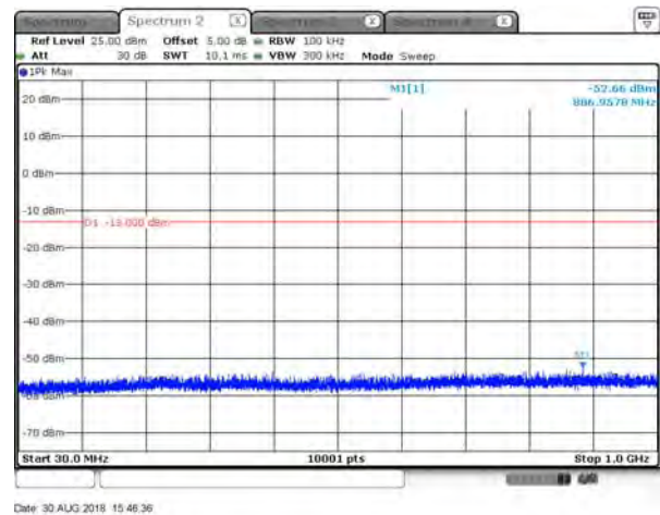
B4_15K_CH20175_QPSK_3RB3_under 1G
