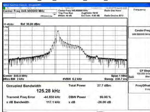
B5_15K_CH20649_BPSK_1RB0
