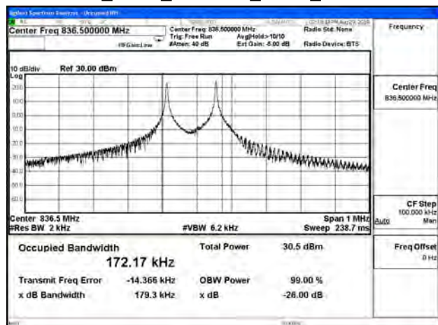
B5_3.75K_CH20525_BPSK_1RB0
