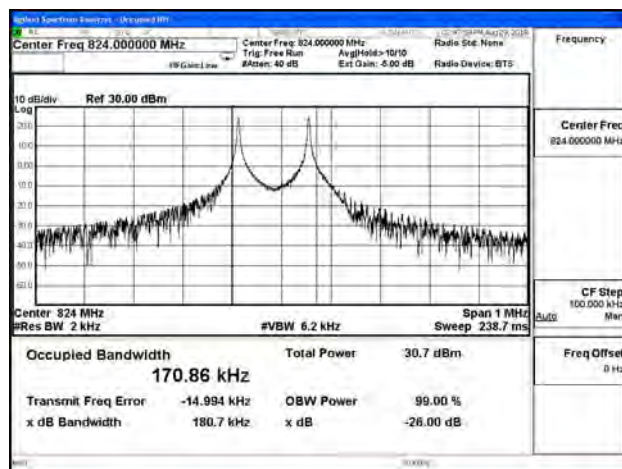
B26_3.75K_CH26790_QPSK_1RB0
