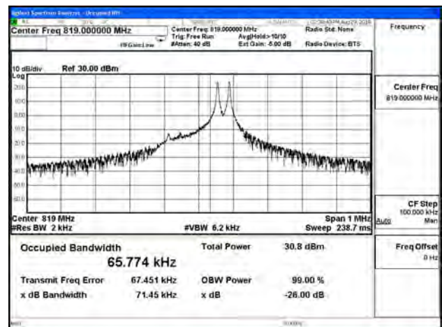
B26_3.75K_CH26740_QPSK_1RB47
