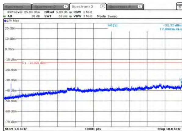
B5_3.75K_CH20525_BPSK_1RB0_above 1G
