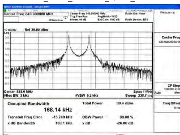
B26_3.75K_CH27039_QPSK_1RB0
