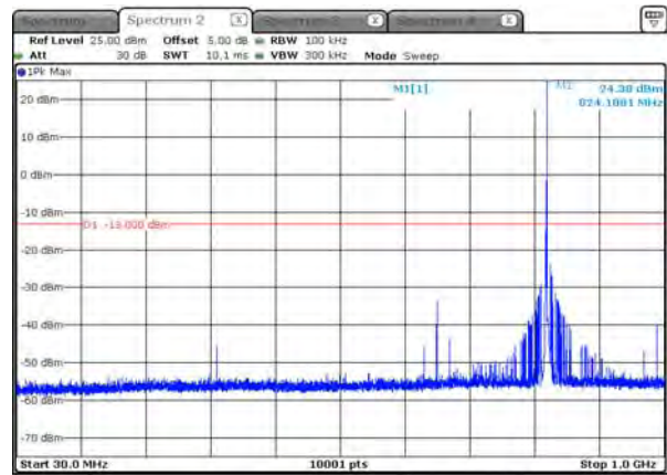
B5_3.75K_CH20401_BPSK_1RB0_under 1G
