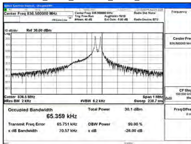
B5_3.75K_CH20525_BPSK_1RB47
