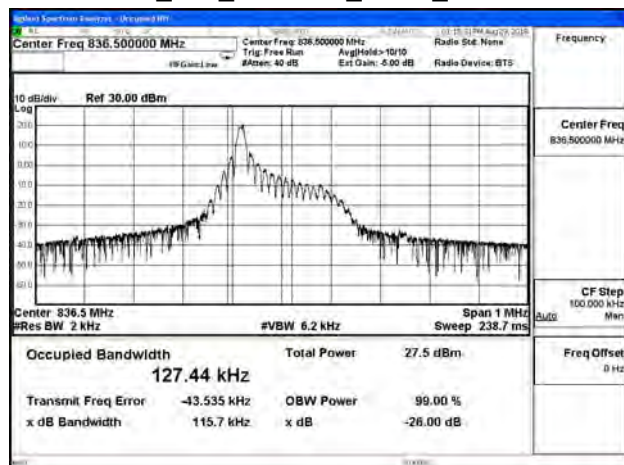
B5_15K_CH20525_BPSK_1RB0
