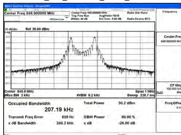
B5_15K_CH20649_BPSK_1RB11
