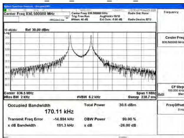
B26_3.75K_CH26915_QPSK_1RB0
