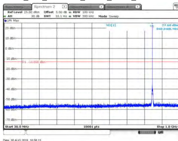
B5_15K_CH20649_QPSK_3RB3_under 1G
