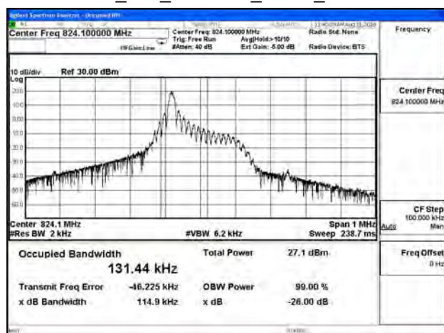
B26_15K_CH26791_QPSK_1RB0
