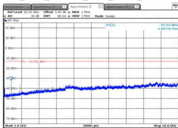
B26_3.75K_CH27039_BPSK_1RB47_above 1G
