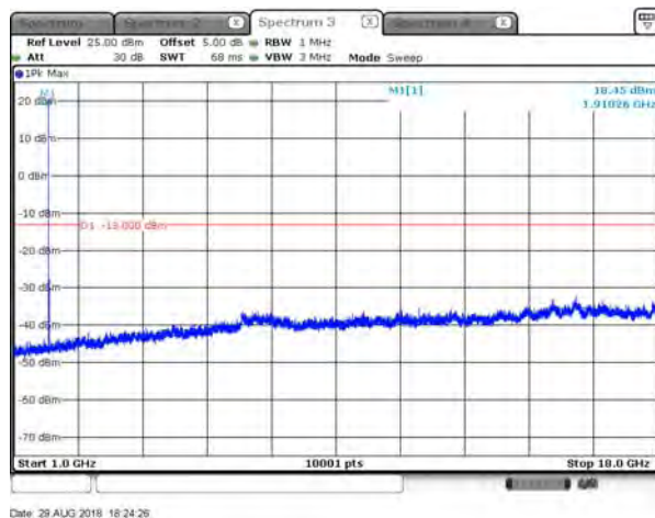
B2_15K_CH19199_QPSK_3RB3_above1G
