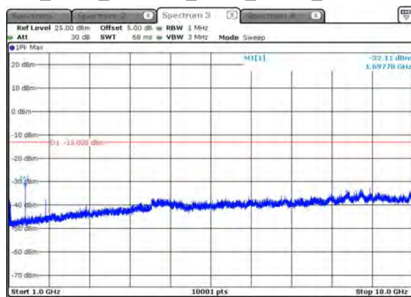
B5_3.75K_CH20649_BPSK_1RB47_above 1G
