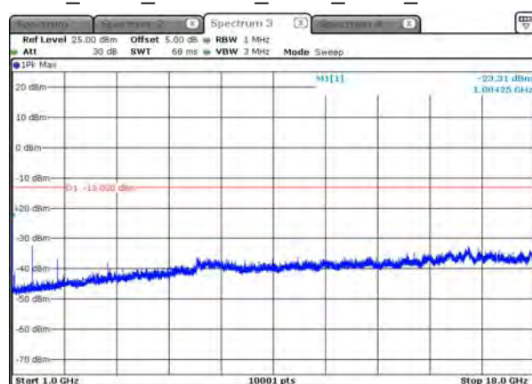
B26_3.75K_CH26740_BPSK_1RB0_above 1G
