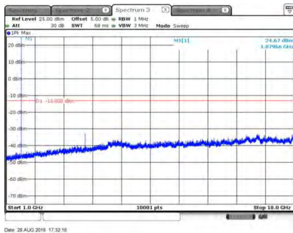
B2_15K_CH19199_QPSK_3RB3_above1G
