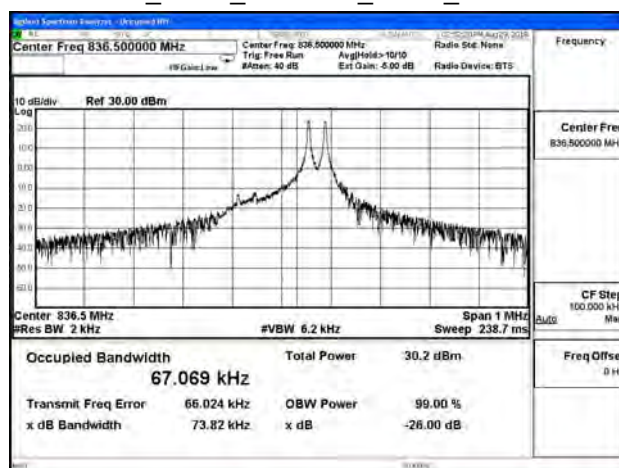
B26_3.75K_CH26915_BPSK_1RB47
