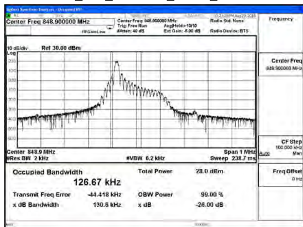
B5_15K_CH20649_QPSK_1RB0
