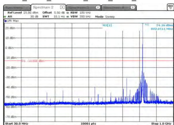
B26_3.75K_CH26788_BPSK_1RB0_under 1G
