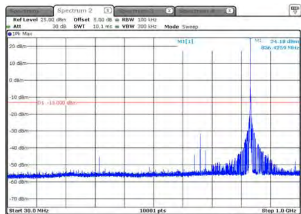
B5_3.75K_CH20525_BPSK_1RB0_under 1G
