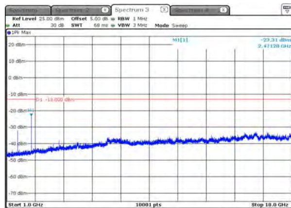
B26_3.75K_CH26790_BPSK_1RB0_above 1G
