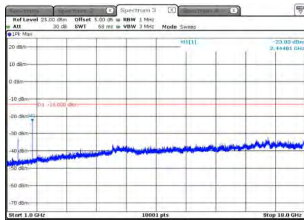
B26_3.75K_CH26692_BPSK_1RB0_above 1G
