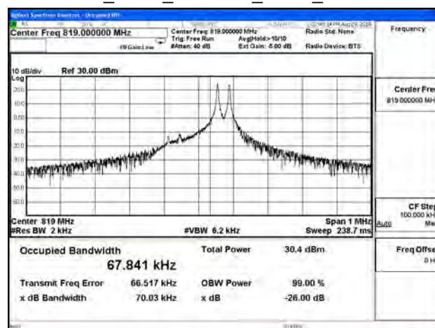
B26_3.75K_CH26740_BPSK_1RB47
