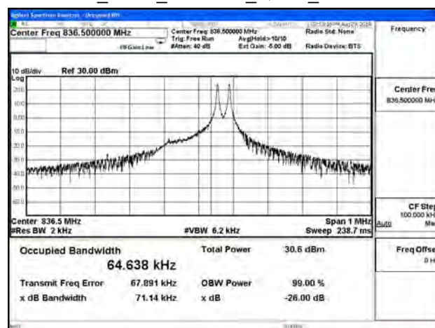
B5_3.75K_CH20525_QPSK_1RB47
