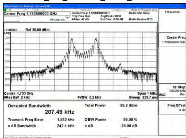
B4_15K_CH20175_QPSK_1RB11
