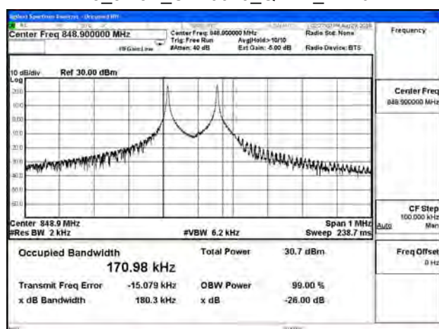
B5_3.75K_CH20649_QPSK_1RB0
