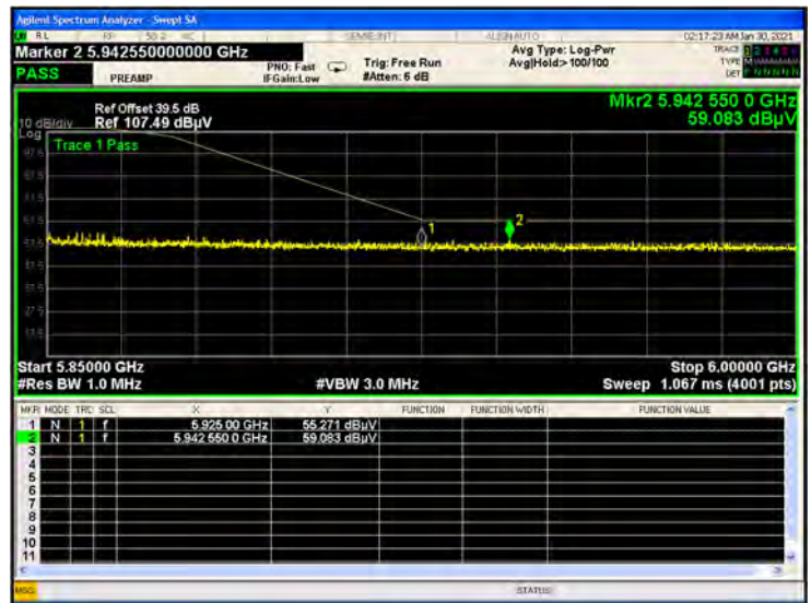
U-NII-3 11a CH165 Peak
