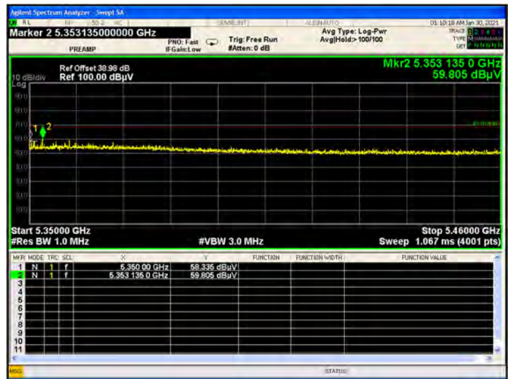
U-NII-2A 11ac20 CH64 Peak
