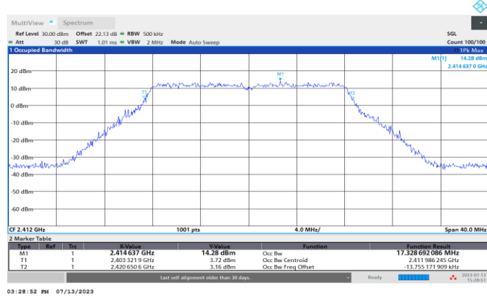
11G-CDD_Ant3_2412
