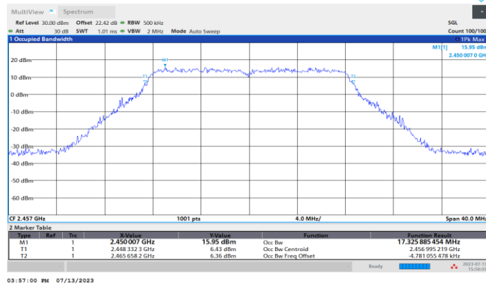
11G-CDD_Ant3_2457
