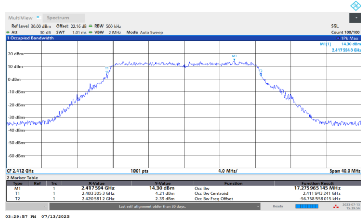
11G-CDD_Ant4_2412
