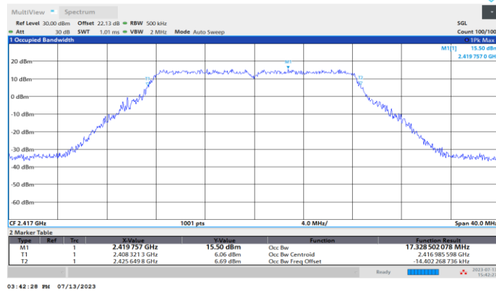
11G-CDD_Ant3_2417
