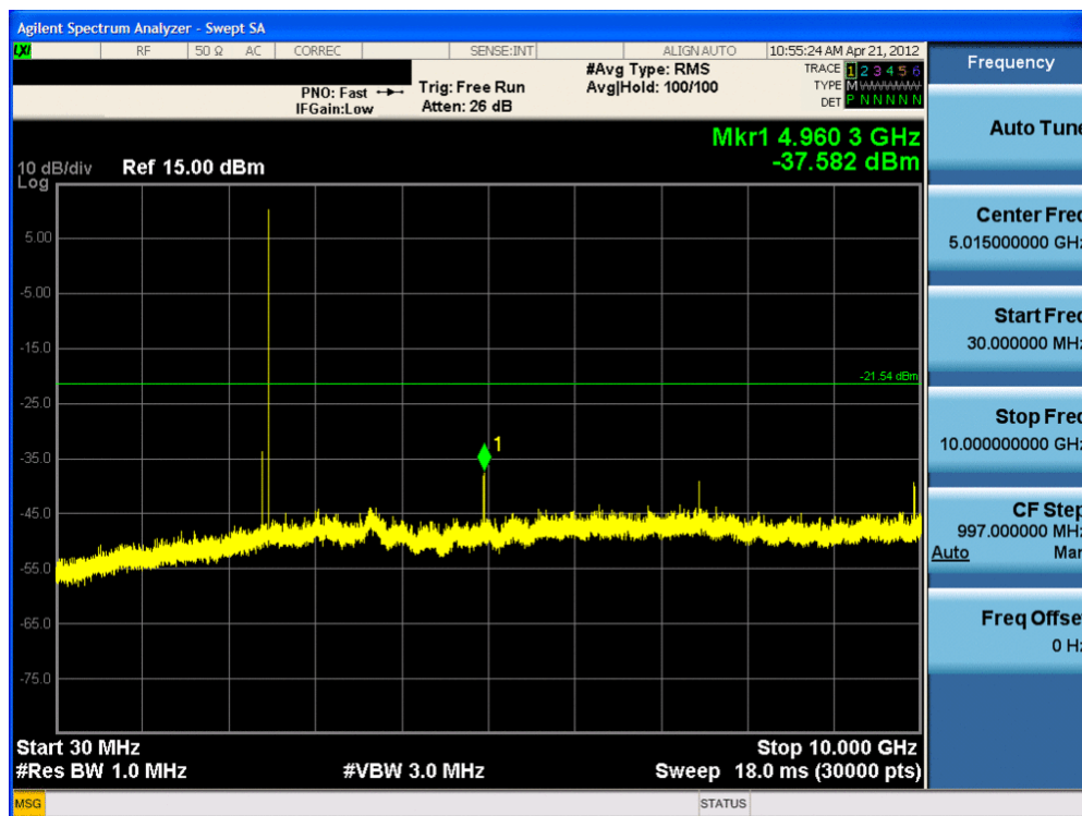
Plot 6-22. Conducted Spurious Plot (Bluetooth, 2Mbps – Ch. 78)
