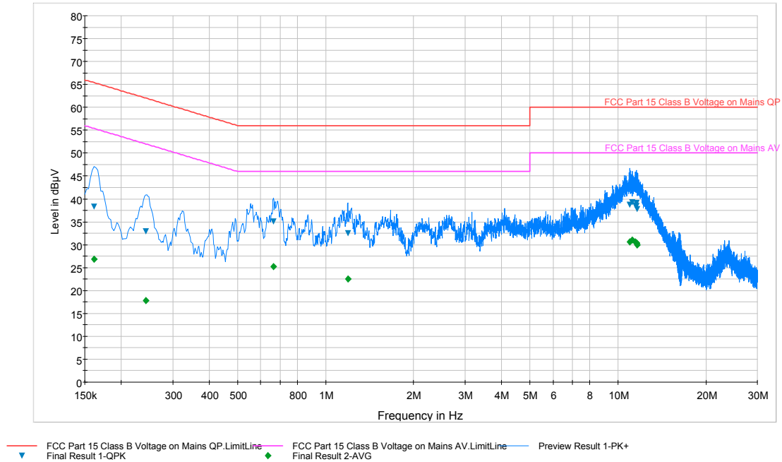
Plot 6-12. Line-Conducted Test Plot (N)
