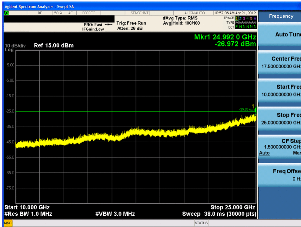
Plot 6-21. Conducted Spurious Plot (Bluetooth, 2Mbps – Ch. 39)
