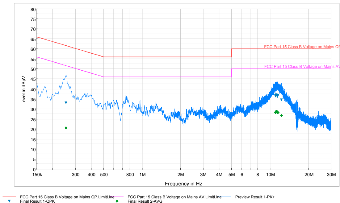
Plot 6-10. Line-Conducted Test Plot (L1)
