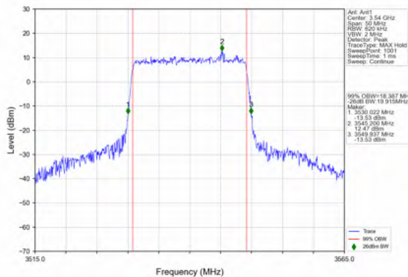
n78e_30kHz_SISO_NTNV_20MHz_CP-OFDM QPSK_3540MHz_Outer_Full
