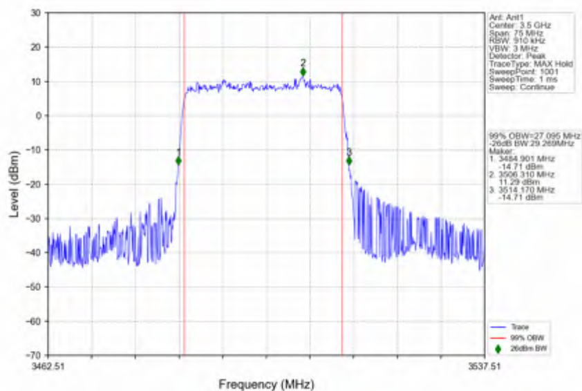
n78e_30kHz_SISO_NTNV_30MHz_DFT-s-OFDM_PI/2_BPSK_3500.01MHz_Outer_Full
