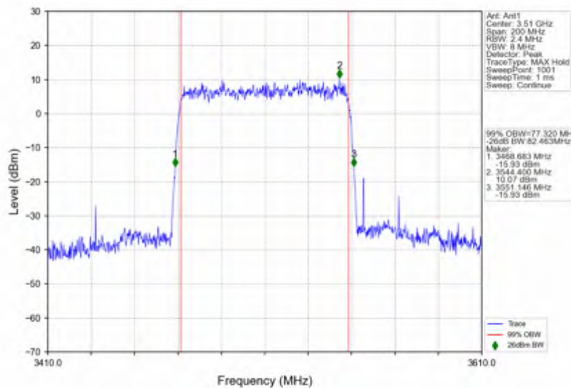
n78e 30kHz SISO NTNv 80MHz DFT-s-OFDM QPSK 3510MHz Outer Full
