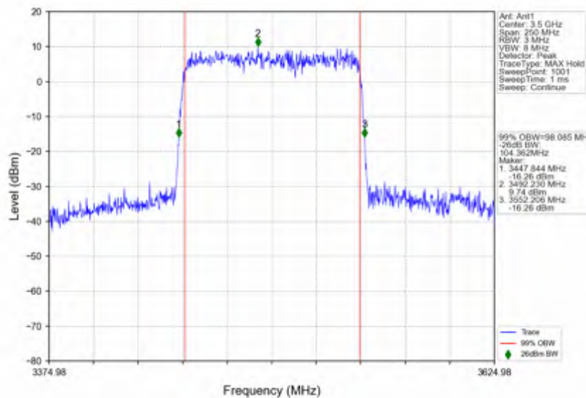
n78e_30kHz_SISO_NTNV_100MHz_CP-OFDM 64 QAM_3500.01MHz_Outer_Full
