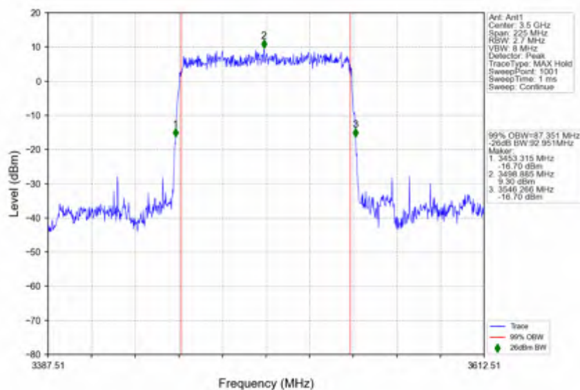
n78e_30kHz_SISO_NTNV_90MHz_DFT-s-OFDM_PI/2_BPSK_3500.01MHz_Outer_Full
