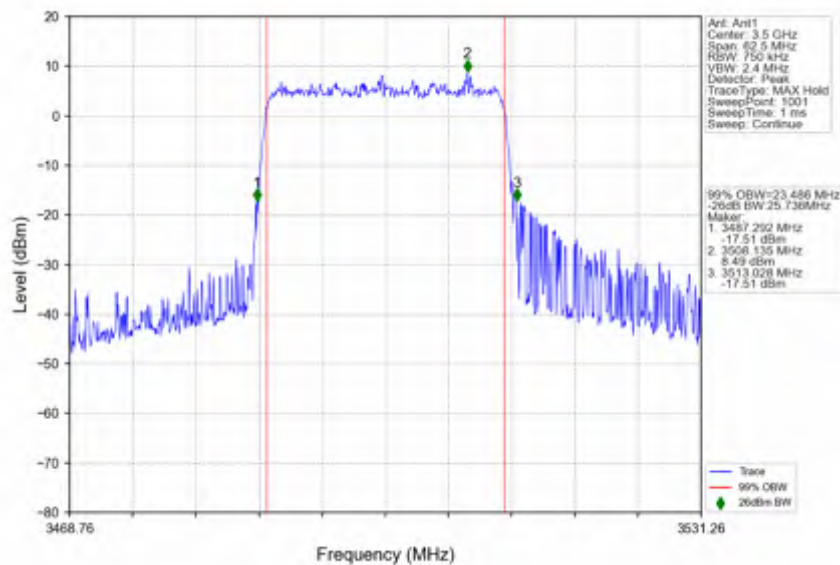
n78e_30kHz_SISO_NTNV_25MHz_CP-OFDM_256_QAM_3500.01MHz_Outer_Full
