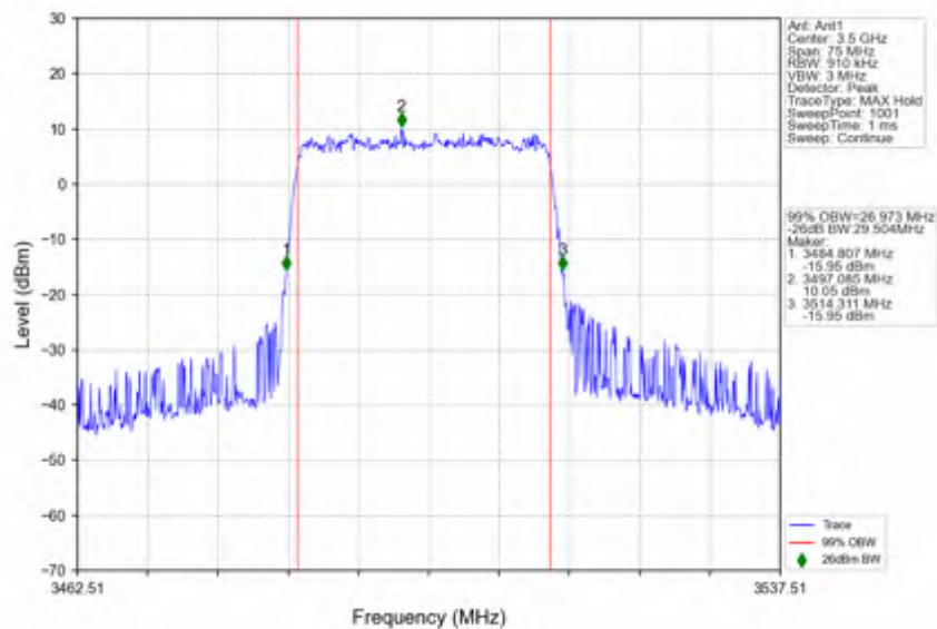
n78e_30kHz_SISO_NTNV_30MHz_DFT-s-OFDM_256_QAM_3500.01MHz_Outer_Full
