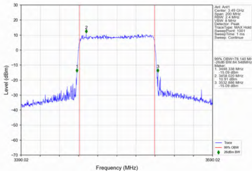
n78e_30kHz_SISO_NTNV_80MHz_CP-OFDM 64 QAM_3490.02MHz_Outer_Full
