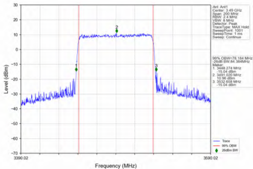
n78e_30kHz_SISO_NTNV_80MHz_CP-OFDM_QPSK_3490.02MHz_Outer_Full
