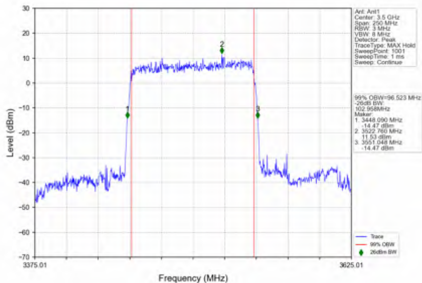
n78e 30kHz SISO NTNV 100MHz DFT-s-OFDM PI/2 BPSK 3500.01MHz Outer Full
