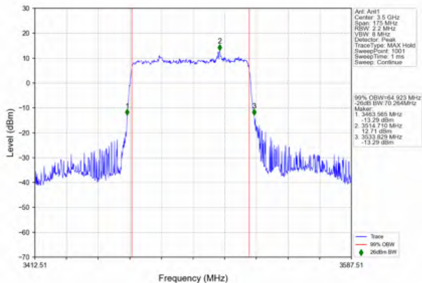
n78e_30kHz_SISO_NTNV_70MHz_DFT-s-OFDM PI/2 BPSK_3500.01MHz_Outer_Full
