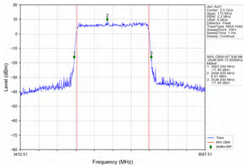
n78e_30kHz_SISO_NTNV_70MHz_CP-OFDM_256_QAM_3500.01MHz_Outer_Full
