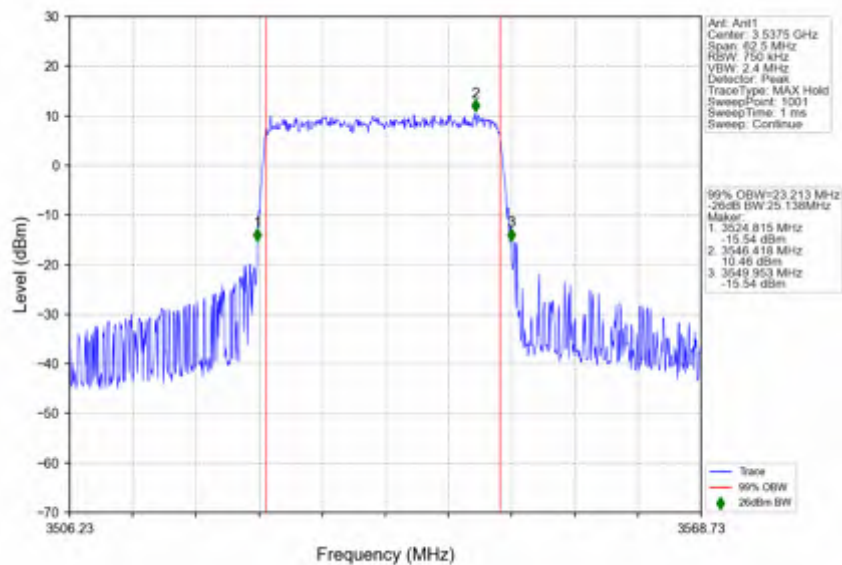
n78e_30kHz_SISO_NTNV_25MHz_DFT-s-OFDM_QPSK_3537.48MHz_Outer_Full
