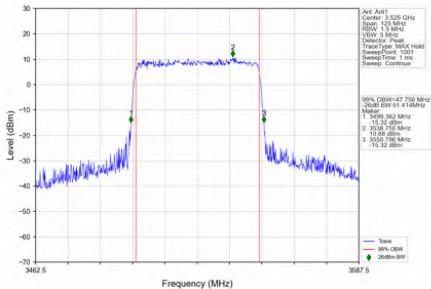
n78e_30kHz_SISO_NTNV_50MHz_CP-OFDM 64 QAM_3525MHz_Outer_Full
