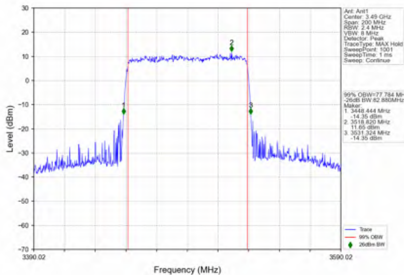
n78e_30kHz_SISO_NTNV_80MHz_DFT-s-OFDM 64 QAM_3490.02MHz_Outer_Full
