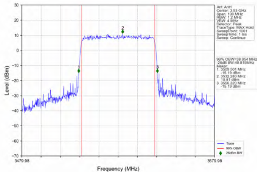
n78e_30kHz_SISO_NTNV_40MHz_CP-OFDM_QPSK_3529.98MHz_Outer_Full
