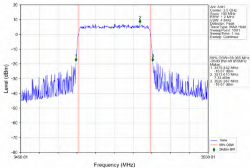
n78e_30kHz_SISO_NTNV_40MHz_CP-OFDM_256_QAM_3500.01MHz_Outer_Full
