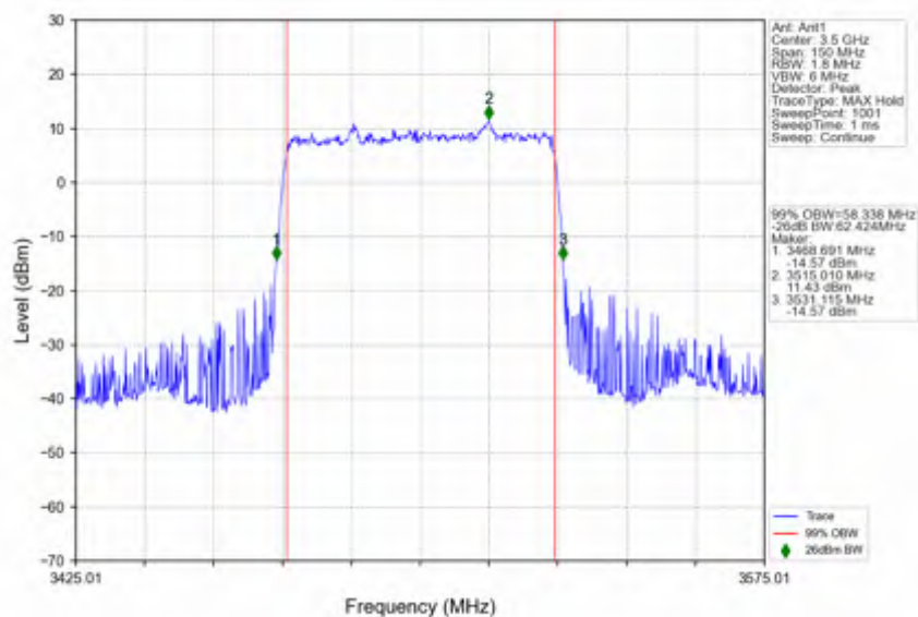
n78e_30kHz_SISO_NTNV_60MHz_DFT-s-OFDM_PI/2_BPSK_3500.01MHz_Outer_Full
