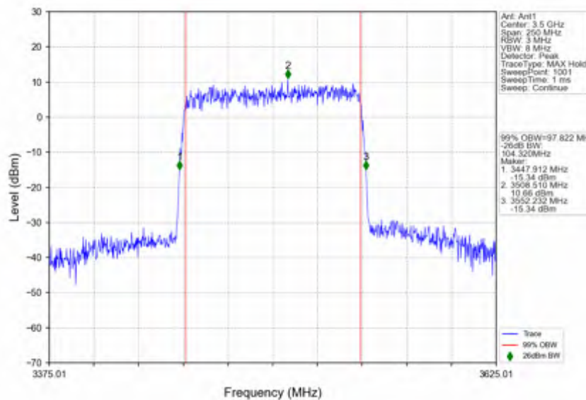
n78e_30kHz_SISO_NTNV_100MHz_CP-OFDM_16_QAM_3500.01MHz_Outer_Full
