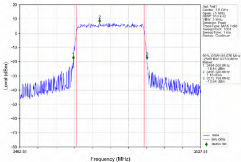
n78e_30kHz_SISO_NTNV_30MHz_CP-OFDM_256_QAM_3500.01MHz_Outer_Full
