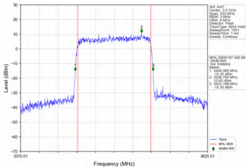
n78e_30kHz_SISO_NTNV_100MHz_CP-OFDM 64 QAM_3499.98MHz_Outer_Full
