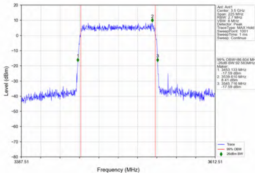
n78e_30kHz_SISO_NTNV_90MHz_DFT-s-OFDM_256_QAM_3500.01MHz_Outer_Full
