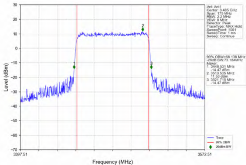
n78e_30kHz_SISO_NTNV_70MHz_CP-OFDM_QPSK_3485.01MHz_Outer_Full
