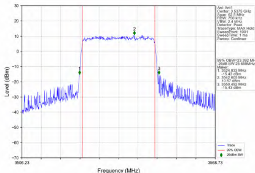
n78e_30kHz_SISO_NTNV_25MHz_CP-OFDM_QPSK_3537.48MHz_Outer_Full
