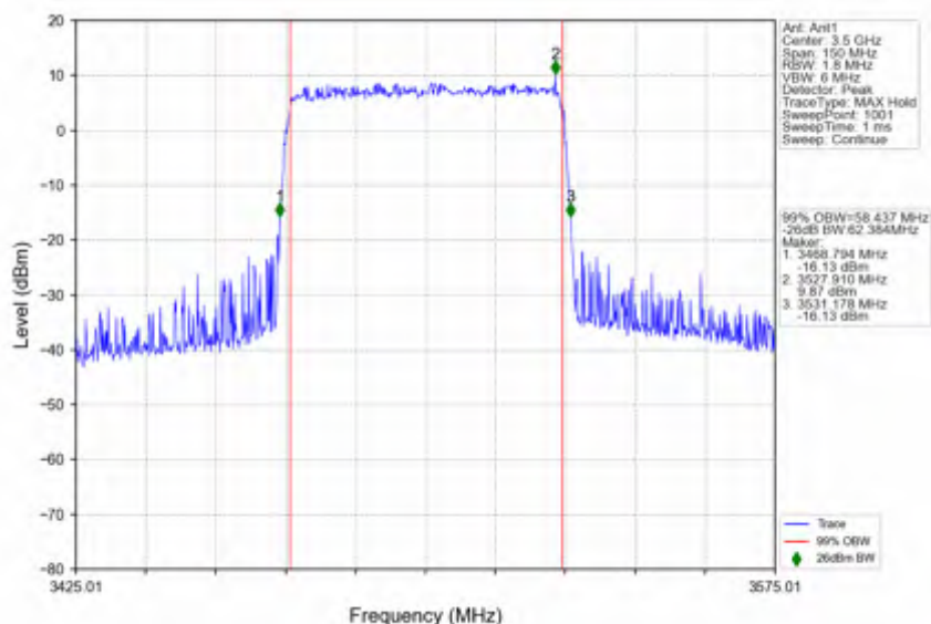
n78e 30kHz SISO NTNV 60MHz DFT-s-OFDM 256 QAM 3500.01MHz Outer Full
