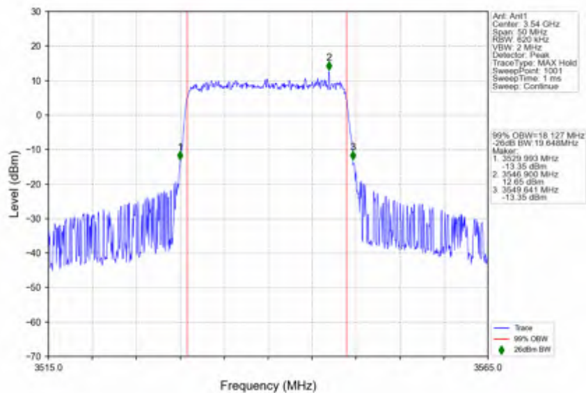
n78e_30kHz_SISO_NTNV_20MHz_DFT-s-OFDM_QPSK_3540MHz_Outer_Full
