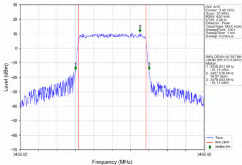
n78e_30kHz_SISO_NTNV_20MHz_CP-OFDM 64 QAM_3460.02MHz_Outer_Full
