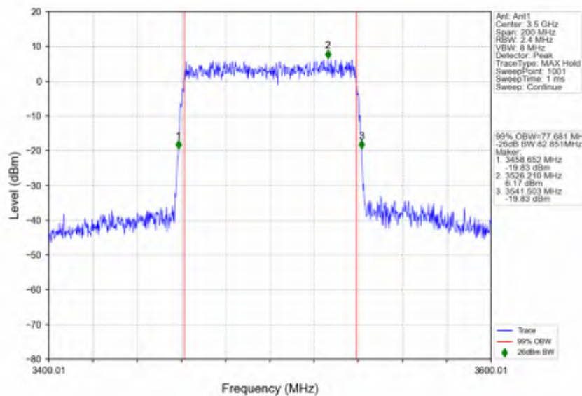
n78e_30kHz_SISO_NTNV_80MHz_CP-OFDM_256_QAM_3500.01MHz_Outer_Full
