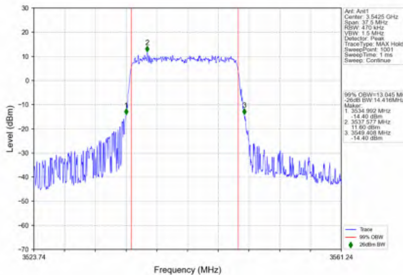
n78e_30kHz_SISO_NTNV_15MHz_DFT-s-OFDM_QPSK_3542.49MHz_Outer_Full
