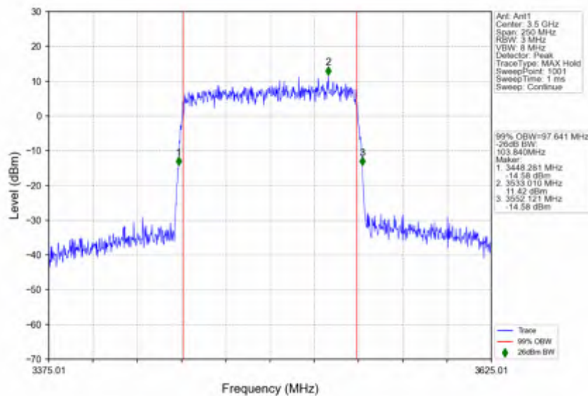
n78e_30kHz_SISO_NTNV_100MHz_CP-OFDM QPSK_3500.01MHz_Outer_Full
