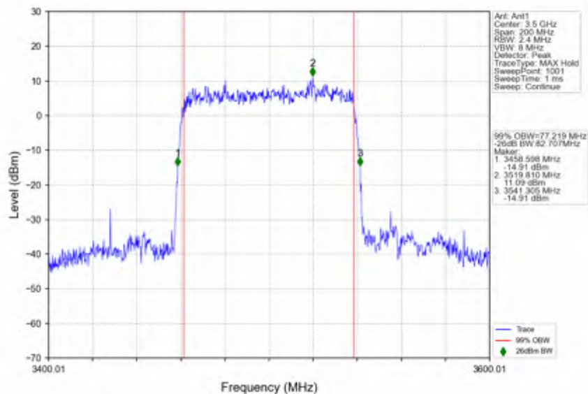
n78e_30kHz_SISO_NTNV_80MHz_DFT-s-OFDM PI/2 BPSK_3500.01MHz_Outer_Full
