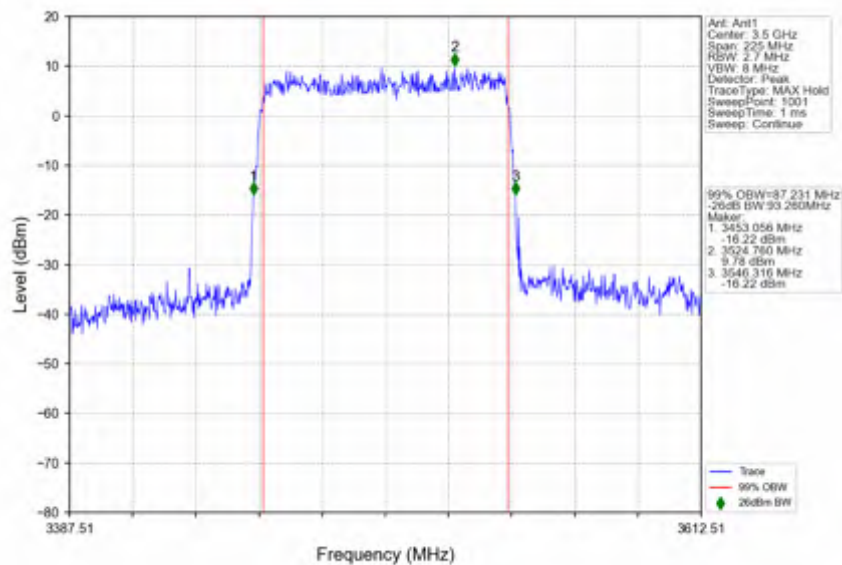
n78e_30kHz_SISO_NTNV_90MHz_DFT-s-OFDM_16_QAM_3500.01MHz_Outer_Full
