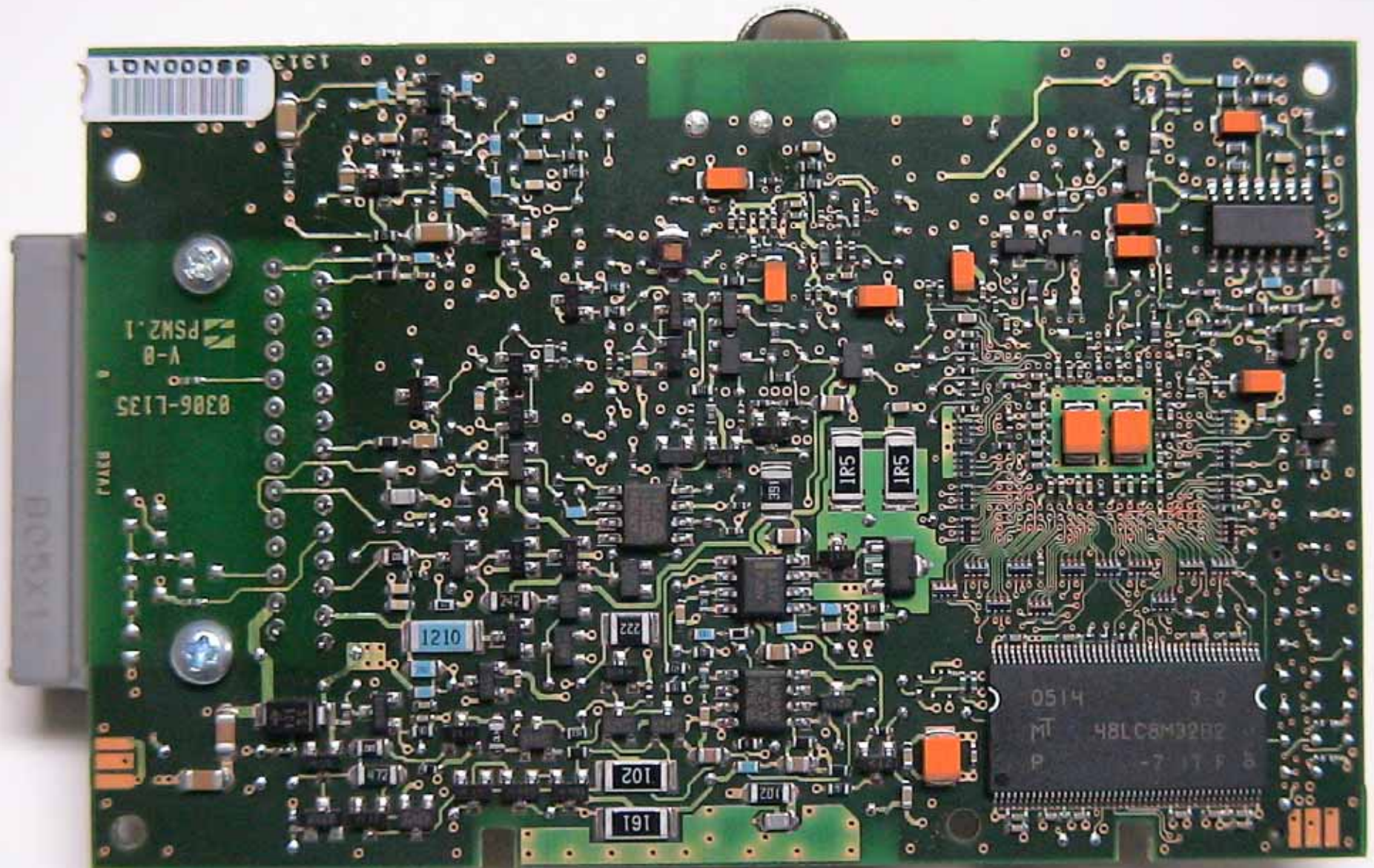
PCB (bottom)
