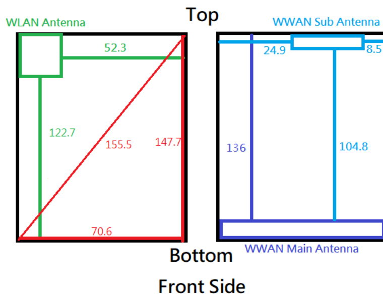
Fig.17 Antenna position of EUT
