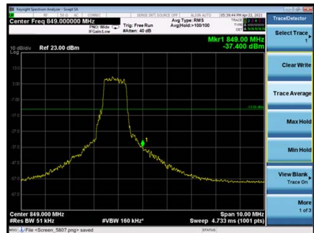
LTE-M Band 26 16QAM 10MHz CH-High 100%RB
