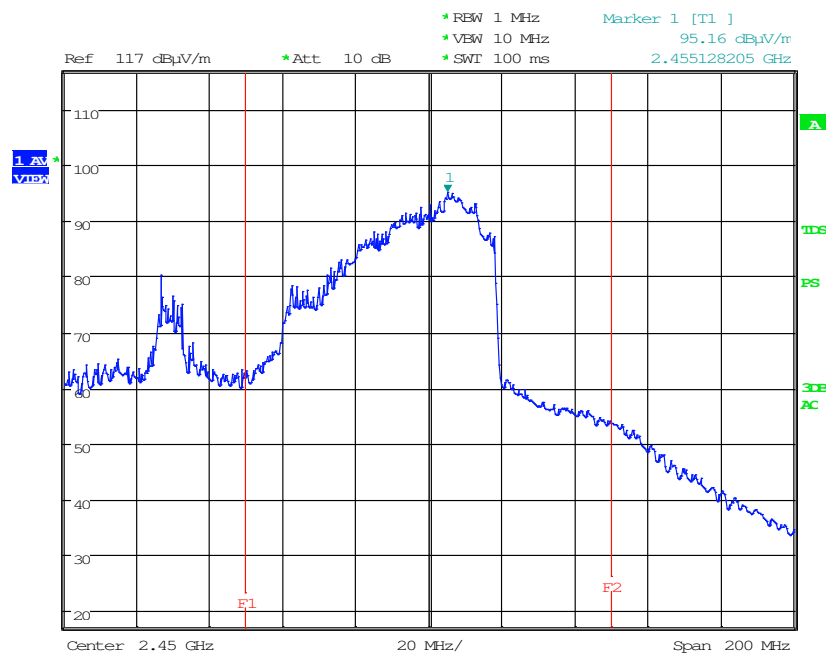
< Fig 8. Frequency Measurements (Minimum Frequency Observed: 2.455 GHz) >
