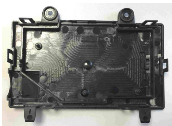
Bottom Housing, View from outside on the part.
