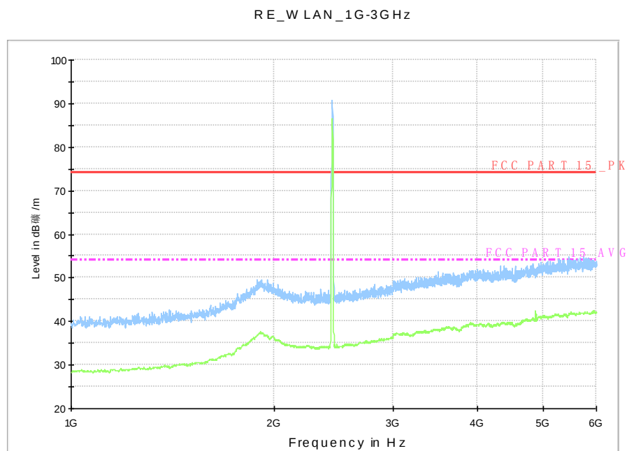
Fig.A.6.2.14 Radiated Spurious Emission (802.11g, Ch6, 1 GHz-3 GHz)
