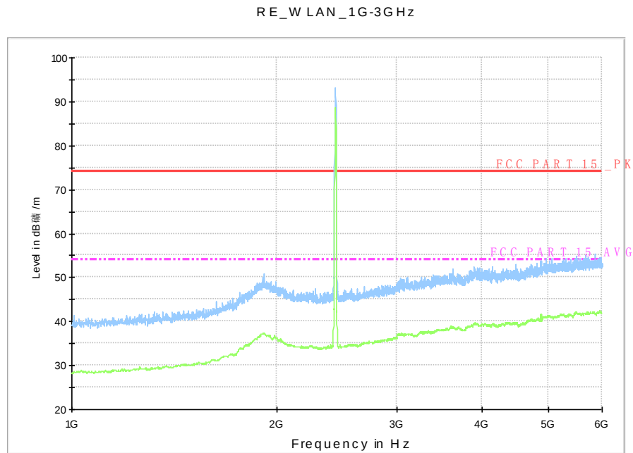
Fig.A.6.2.5 Radiated Spurious Emission (802.11b, Ch6, 1 GHz-3 GHz)
