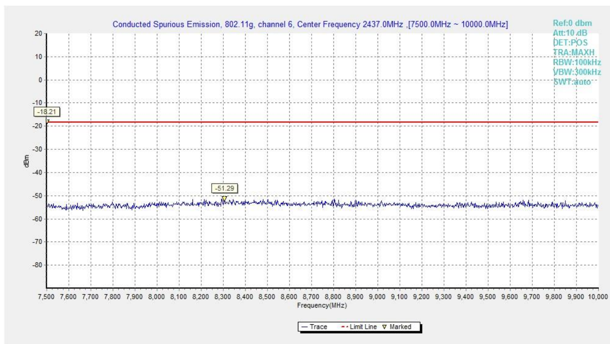
Fig.A.6.1.37 Conducted Spurious Emission (802.11g, Ch6, 7.5 GHz-10 GHz)
