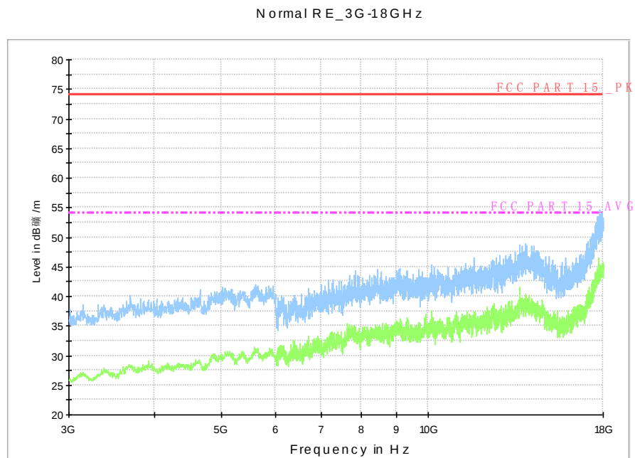
Fig.A.6.2.18 Radiated Spurious Emission (802.11g, Ch11, 3 GHz-18 GHz)
