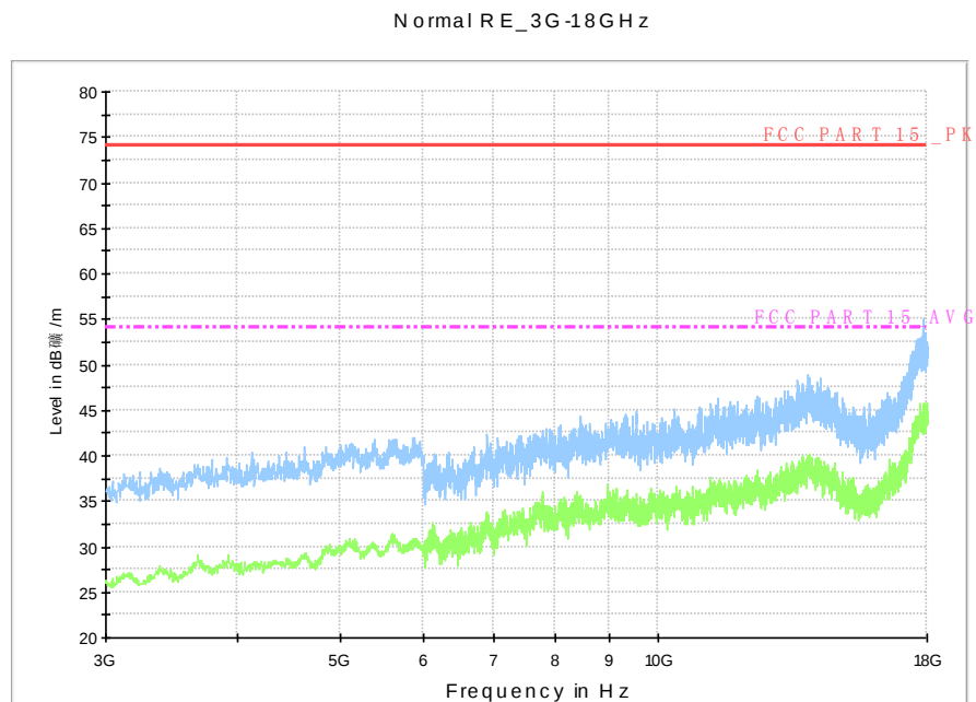
Fig.A.6.2.12 Radiated Spurious Emission (802.11g, Ch1, 3 GHz-18 GHz)
