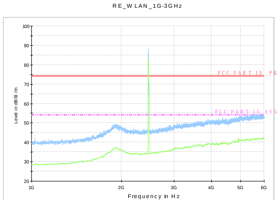
Fig.A.6.2.26 Radiated Spurious Emission (802.11n-HT20, Ch11, 1 GHz-3 GHz)
