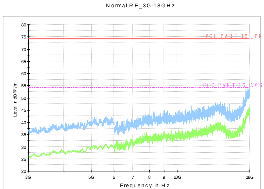
Fig.A.6.2.24 Radiated Spurious Emission (802.11n-HT20, Ch6, 3 GHz-18 GHz)
