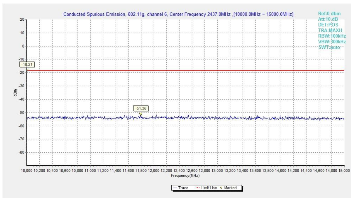
Fig.A.6.1.38 Conducted Spurious Emission (802.11g, Ch6, 10 GHz-15 GHz)
