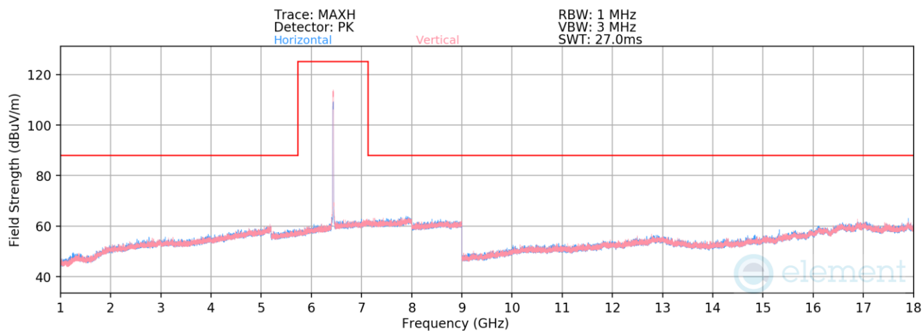
Plot 7-655. Radiated Spurious Emissions above 1GHz SDM Diversity (802.11ax – Ch. 97)
