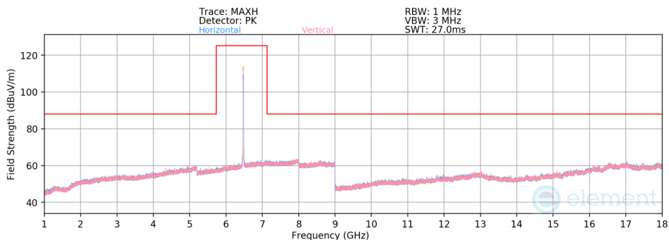
Plot 7-656. Radiated Spurious Emissions above 1GHz SDM Diversity (802.11ax – Ch. 105)
