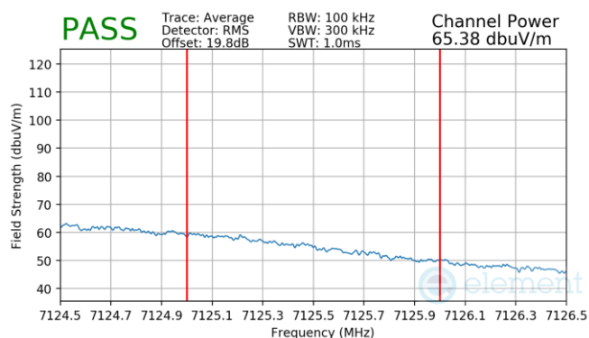
Plot 7-670. Antenna 5T Radiated Upper Band Edge (Average – UNII Band 8)
