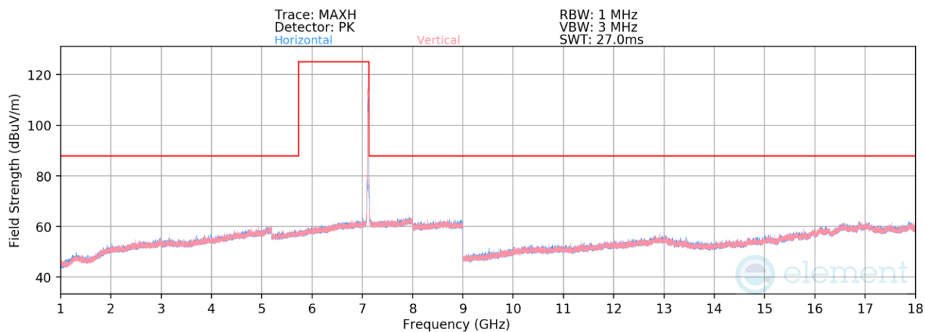
Plot 7-666. Radiated Spurious Emissions above 1GHz SDM Diversity (802.11ax – Ch. 233)
