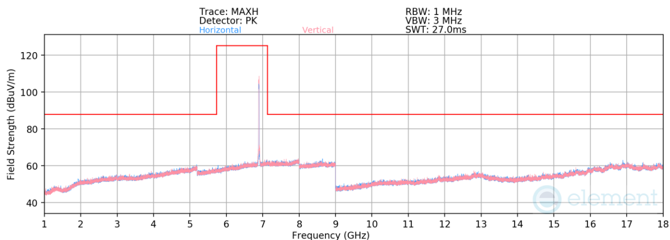
Plot 7-632. Radiated Spurious Emissions above 1GHz Antenna 1b (802.11ax – Ch. 189)
