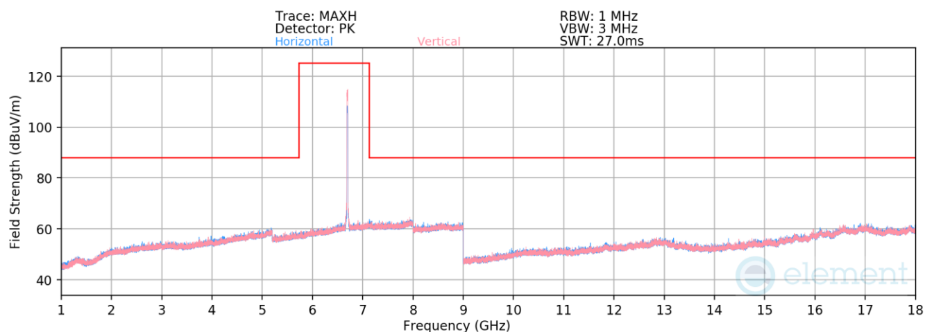
Plot 7-661. Radiated Spurious Emissions above 1GHz SDM Diversity (802.11ax – Ch. 149)
