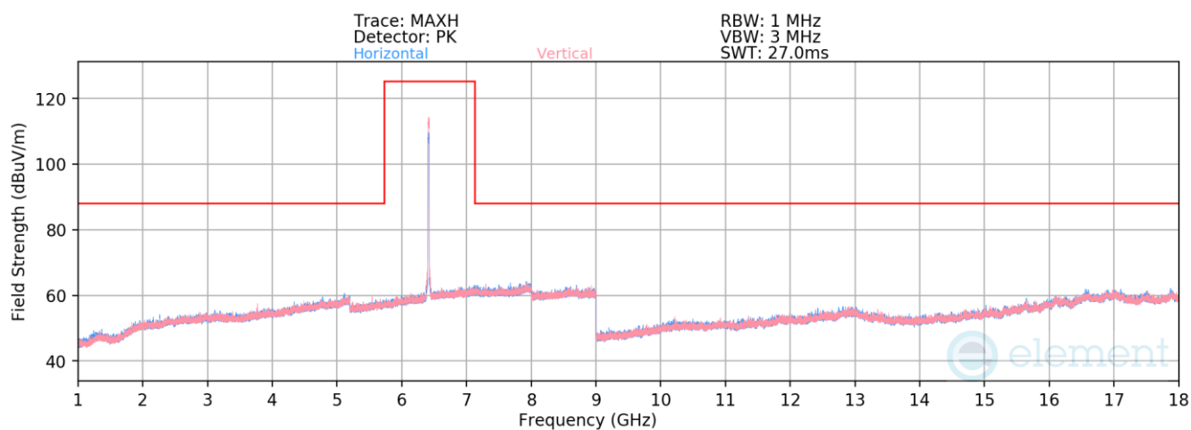
Plot 7-654. Radiated Spurious Emissions above 1GHz SDM Diversity (802.11ax – Ch. 93)
