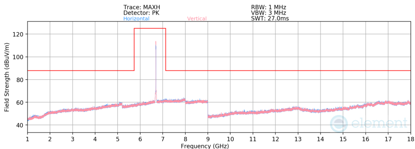
Plot 7-645. Radiated Spurious Emissions above 1GHz SDM Primary (802.11ax – Ch. 149)
