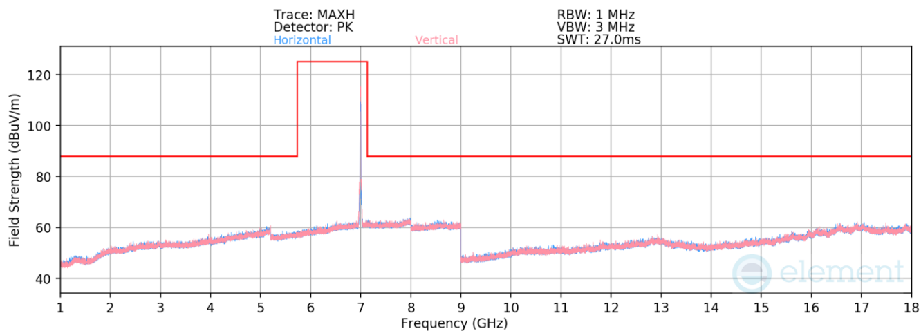
Plot 7-649. Radiated Spurious Emissions above 1GHz SDM Primary (802.11ax – Ch. 209)
