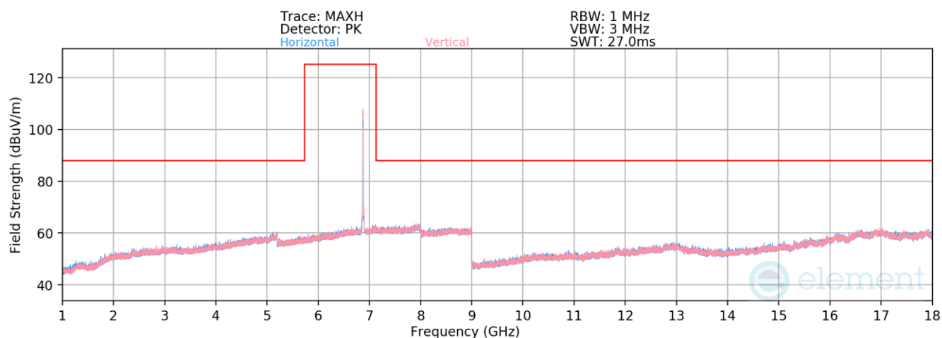
Plot 7-631. Radiated Spurious Emissions above 1GHz Antenna 1b (802.11ax – Ch. 185)
