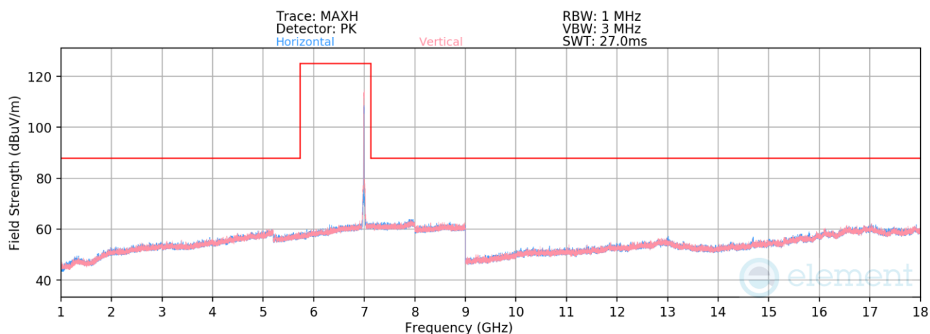
Plot 7-665. Radiated Spurious Emissions above 1GHz SDM Diversity (802.11ax – Ch. 209)
