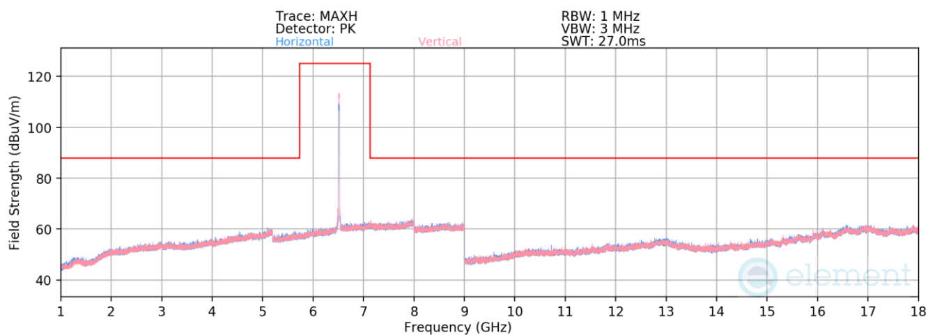
Plot 7-641. Radiated Spurious Emissions above 1GHz SDM Primary (802.11ax – Ch. 113)
