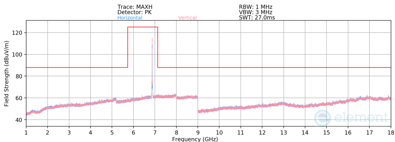
Plot 7-662. Radiated Spurious Emissions above 1GHz SDM Diversity (802.11ax – Ch. 185)
