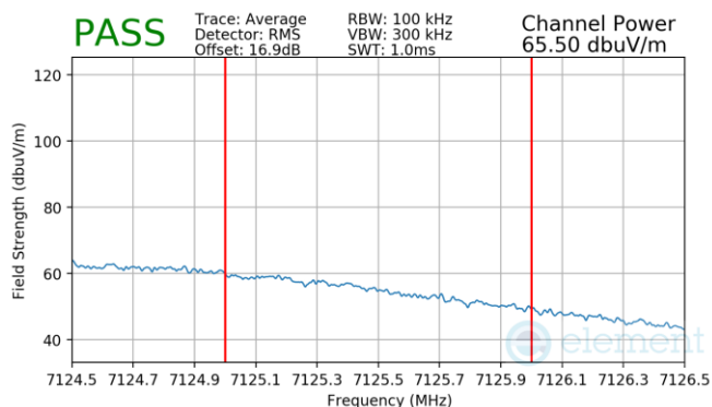
Plot 7-684. Antenna 3b Radiated Upper Band Edge (Average – UNII Band 8)
