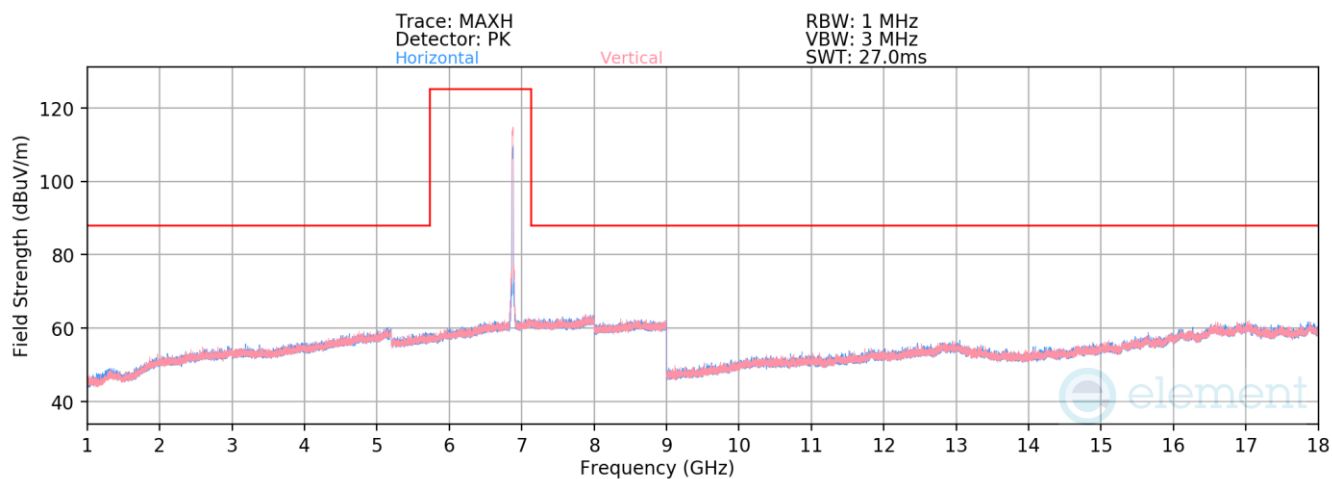
Plot 7-646. Radiated Spurious Emissions above 1GHz SDM Primary (802.11ax – Ch. 185)
