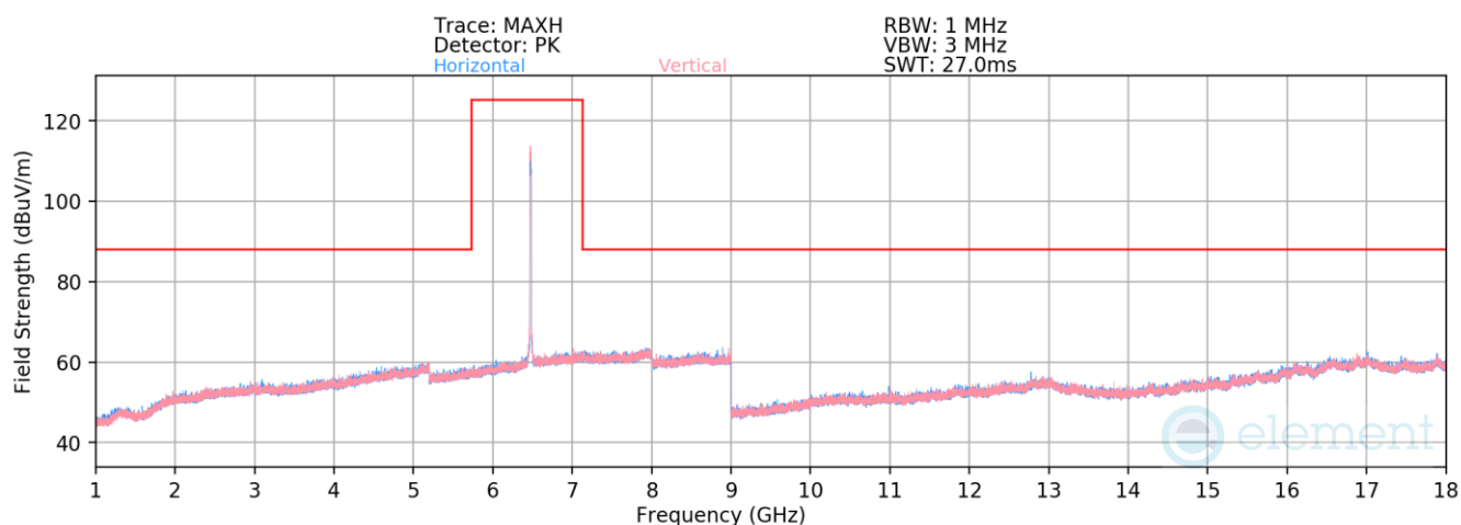
Plot 7-640. Radiated Spurious Emissions above 1GHz SDM Primary (802.11ax – Ch. 105)
