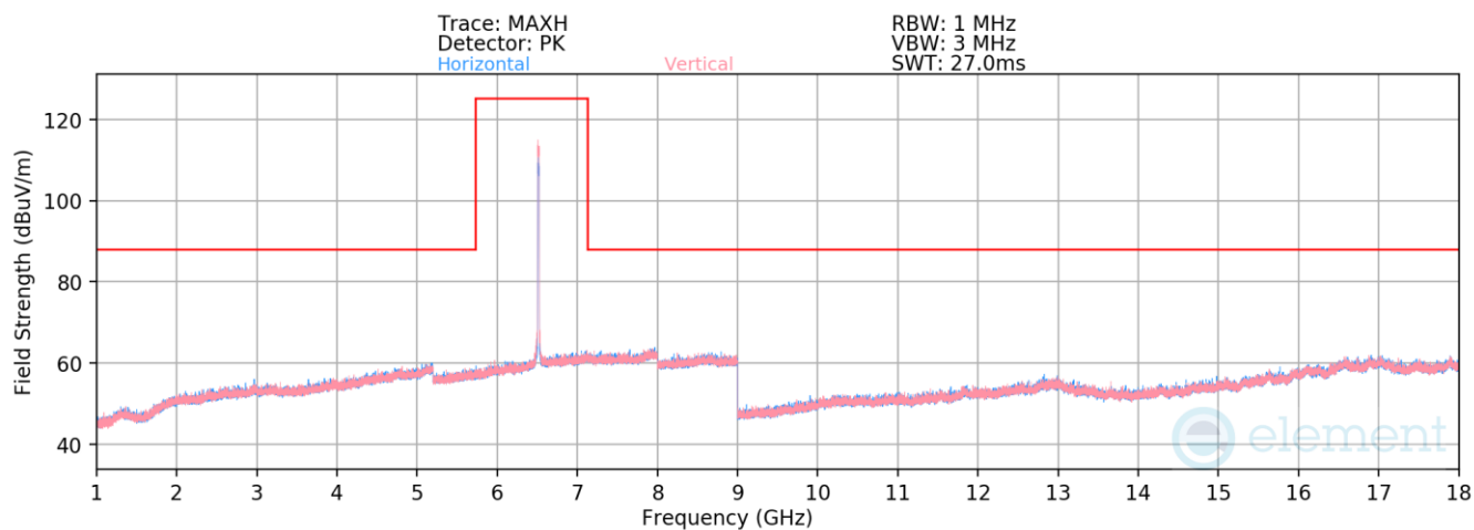
Plot 7-657. Radiated Spurious Emissions above 1GHz SDM Diversity (802.11ax – Ch. 113)
