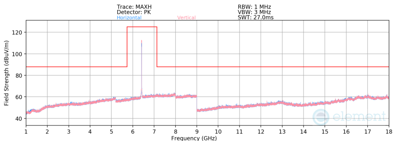
Plot 7-638. Radiated Spurious Emissions above 1GHz SDM Primary (802.11ax – Ch. 93)
