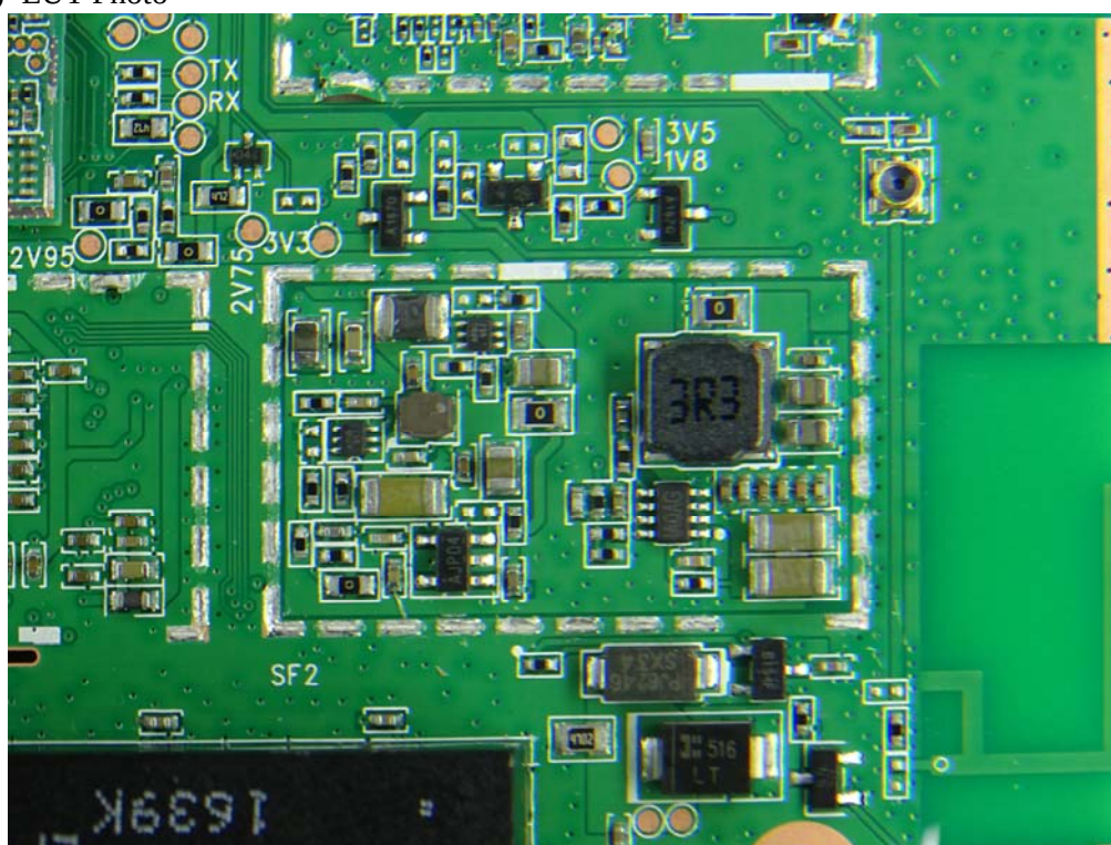
(23) EUT Photo
