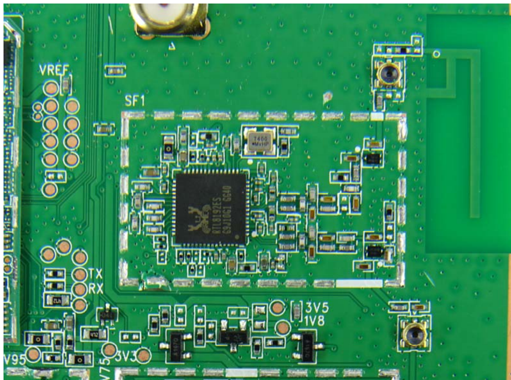
(11) EUT Photo
