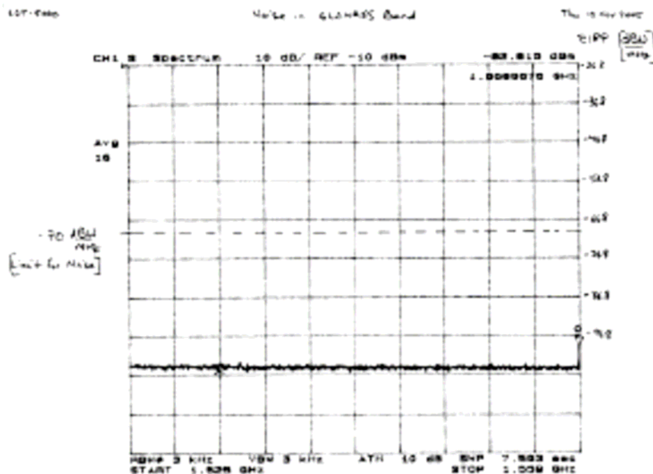
Figure 2. Noise and Spurious in Receive Band 1525 to 1559 MHz.
