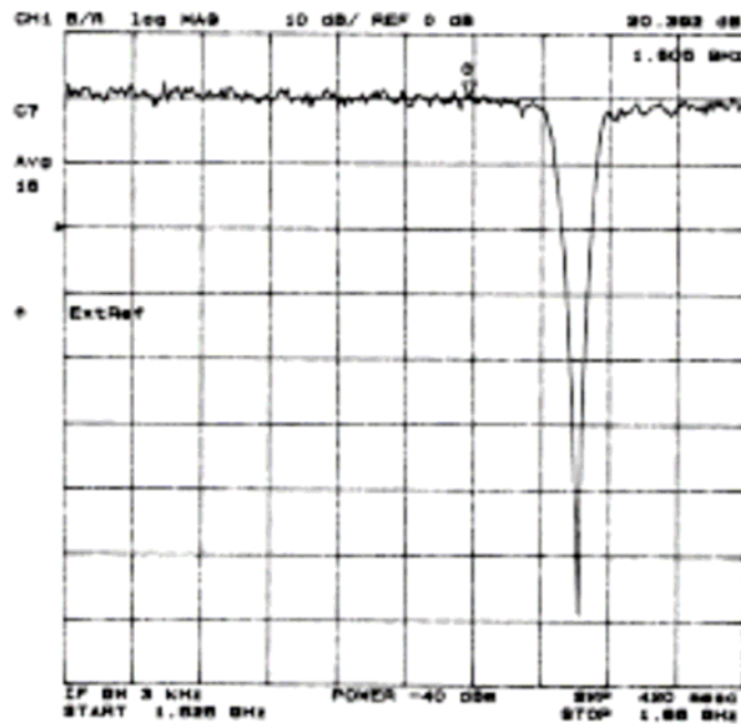
Figure 5. System Gain
