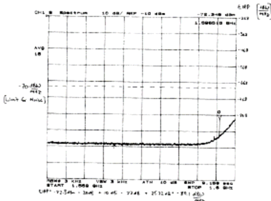
Figure 3. Noise and Spurious in Receive Band 1559 to 1600 MHz.
