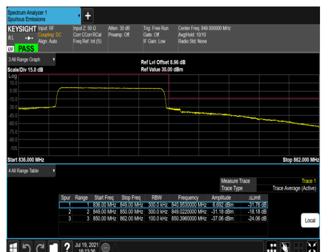
Band5-10MHz-16QAM-20600-50RB#0
