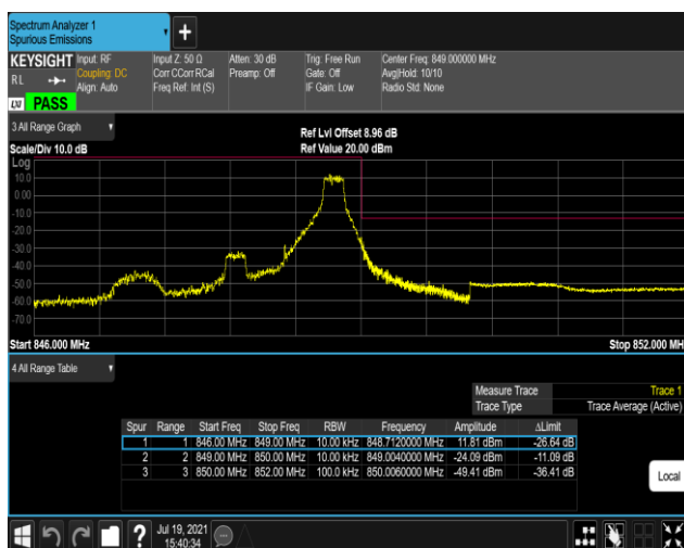
Band5-1.4MHz-16QAM-20643-1RB#5
