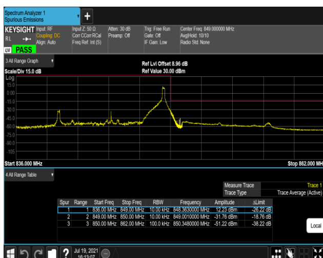
Band5-10MHz-16QAM-20600-1RB#49
