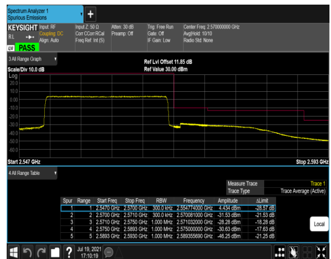
Band7-20MHz-QPSK-21350-100RB#0
