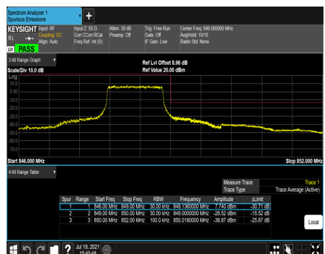
Band5-1.4MHz-QPSK-20643-6RB#0
