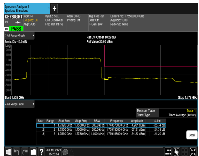
Band4-20MHz-QPSK-20300-100RB#0
