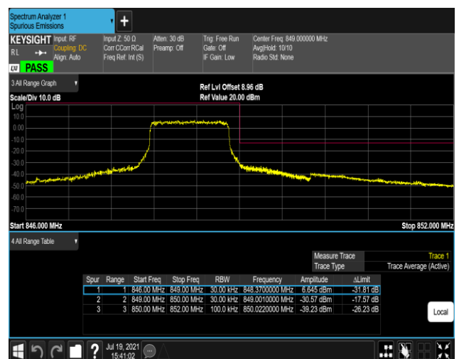
Band5-1.4MHz-16QAM-20643-6RB#0
