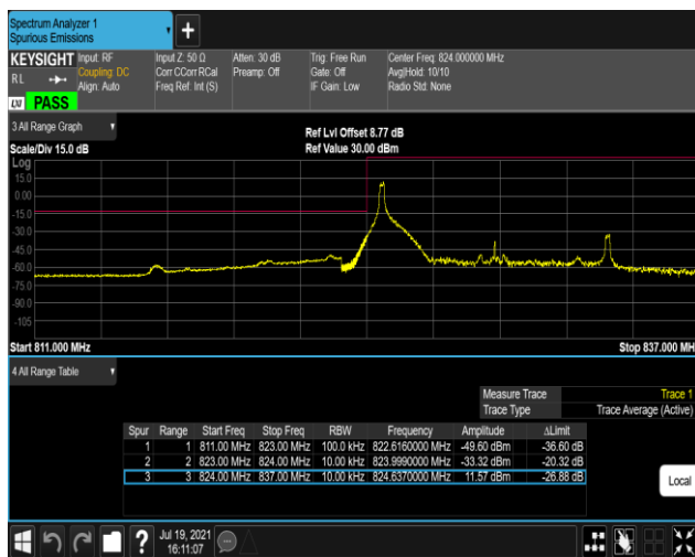
Band5-10MHz-16QAM-20450-50RB#0
