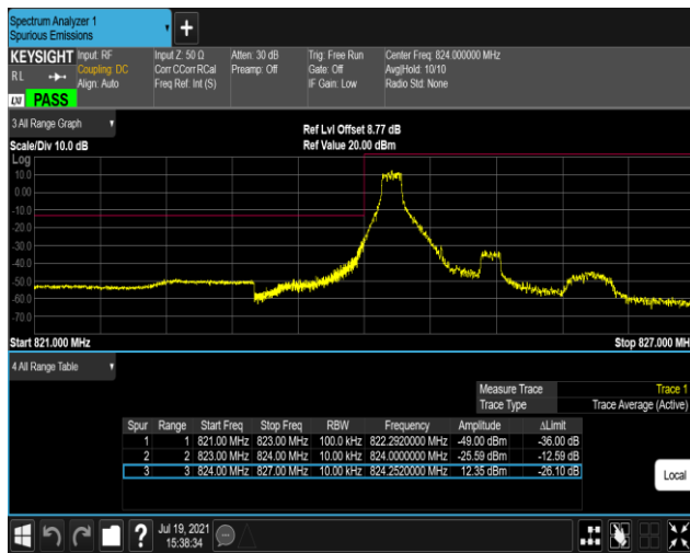
Band5-1.4MHz-16QAM-20407-6RB#0
