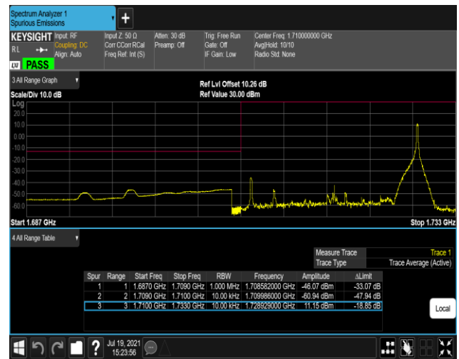
Band4-20MHz-QPSK-20300-1RB#0
