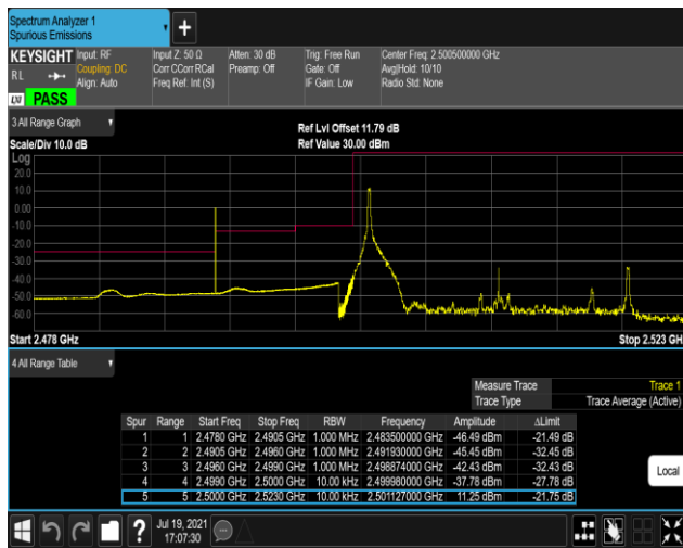
Band7-20MHz-QPSK-20850-100RB#0
