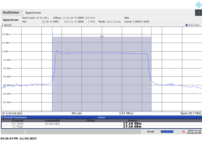
Antenna Port 2
