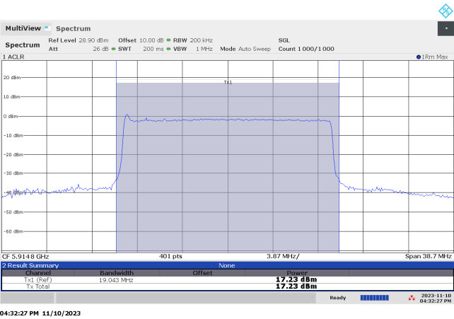
Antenna Port 1
