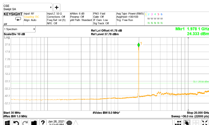
Figure 8.5-24: Conducted spurious emissions of 20 MHz two top channels, two-carrier operation
