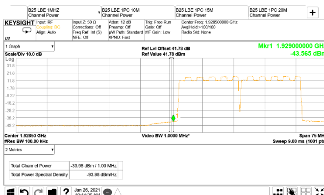
Figure 8.5-74: Conducted band edge emission at 1929 MHz, 15 MHz channel two-carrier operation (RBW = 1 MHz)
