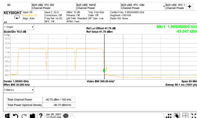
Figure 8.5-87: Conducted band edge emission at 1995 MHz, 10 MHz channel three-carrier operation (RBW = 1% of EBW)
