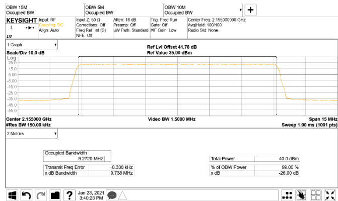
Figure 8.6-2: 99% Occupied bandwidth and 26 dB bandwidth sample plot for 10 MHz channel
