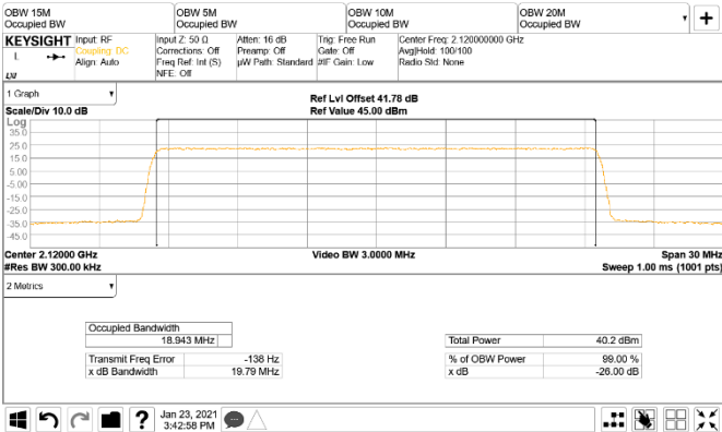
Figure 8.6-4: 99% Occupied bandwidth and 26 dB bandwidth sample plot for 20 MHz channel
