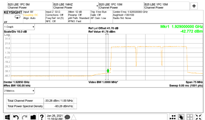
Figure 8.5-86: Conducted band edge emission at 1929 MHz, 10 MHz channel three-carrier operation (RBW = 1 MHz)
