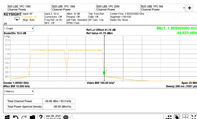
Figure 8.5-67: Conducted band edge emission at 1995 MHz, 5 MHz channel two-carrier operation (RBW = 1% of EBW)
