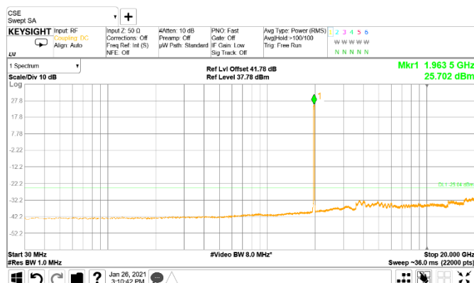
Figure 8.5-20: Conducted spurious emissions of 15 MHz two mid channels, two-carrier operation
