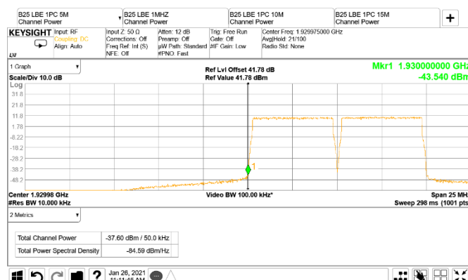
Figure 8.5-65: Conducted band edge emission at 1930 MHz, 5 MHz channel two-carrier operation (RBW = 1% of EBW)
