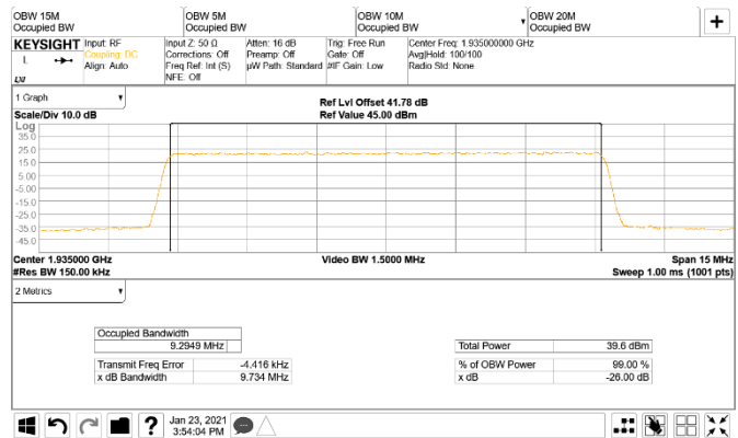
Figure 8.7-2: 99% Occupied bandwidth and 26 dB bandwidth sample plot for 10 MHz channel
