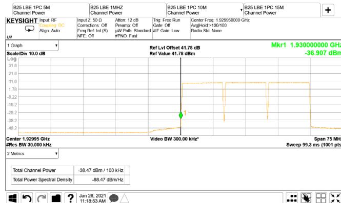
Figure 8.5-85: Conducted band edge emission at 1930 MHz, 10 MHz channel three-carrier operation (RBW = 1% of EBW)
