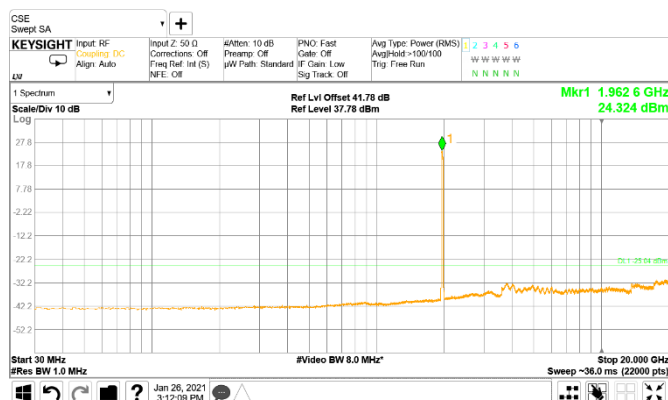
Figure 8.5-22: Conducted spurious emissions of 20 MHz two low channels, two-carrier operation
