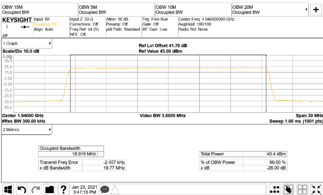
Figure 8.7-4: 99% Occupied bandwidth and 26 dB bandwidth sample plot for 20 MHz channel
