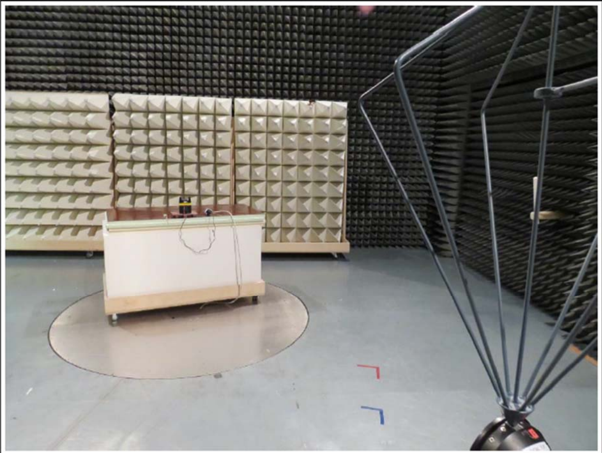
VIEW A1
