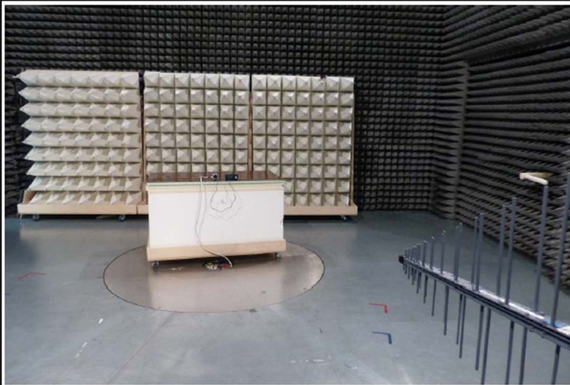
Test Setup 200-1000MHz EUT configuration 3
