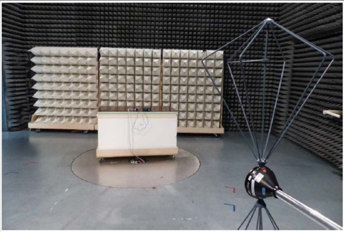
Test Setup 30-200MHz EUT configuration 3
