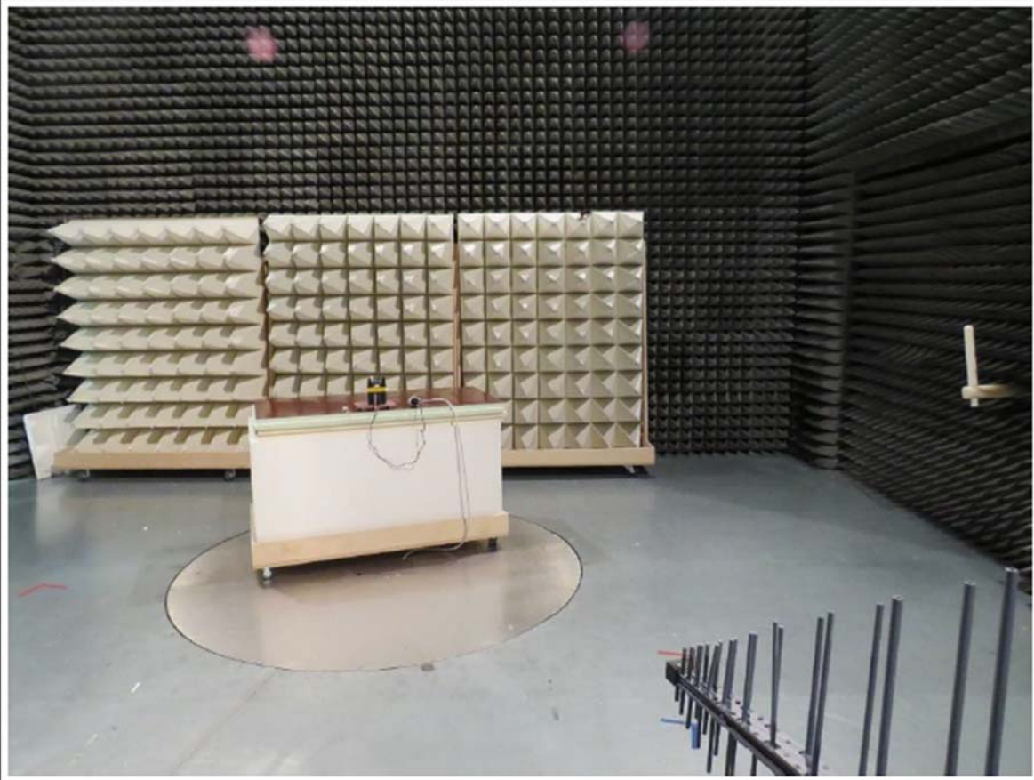
VIEW A2
