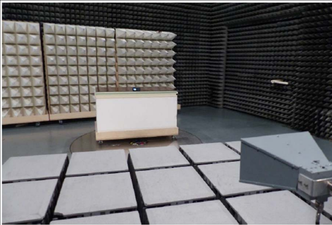
Test Setup 1-13GHz EUT configuration 1, 2
