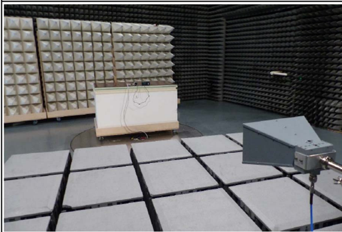
Test Setup 1-13GHz EUT configuration 3
