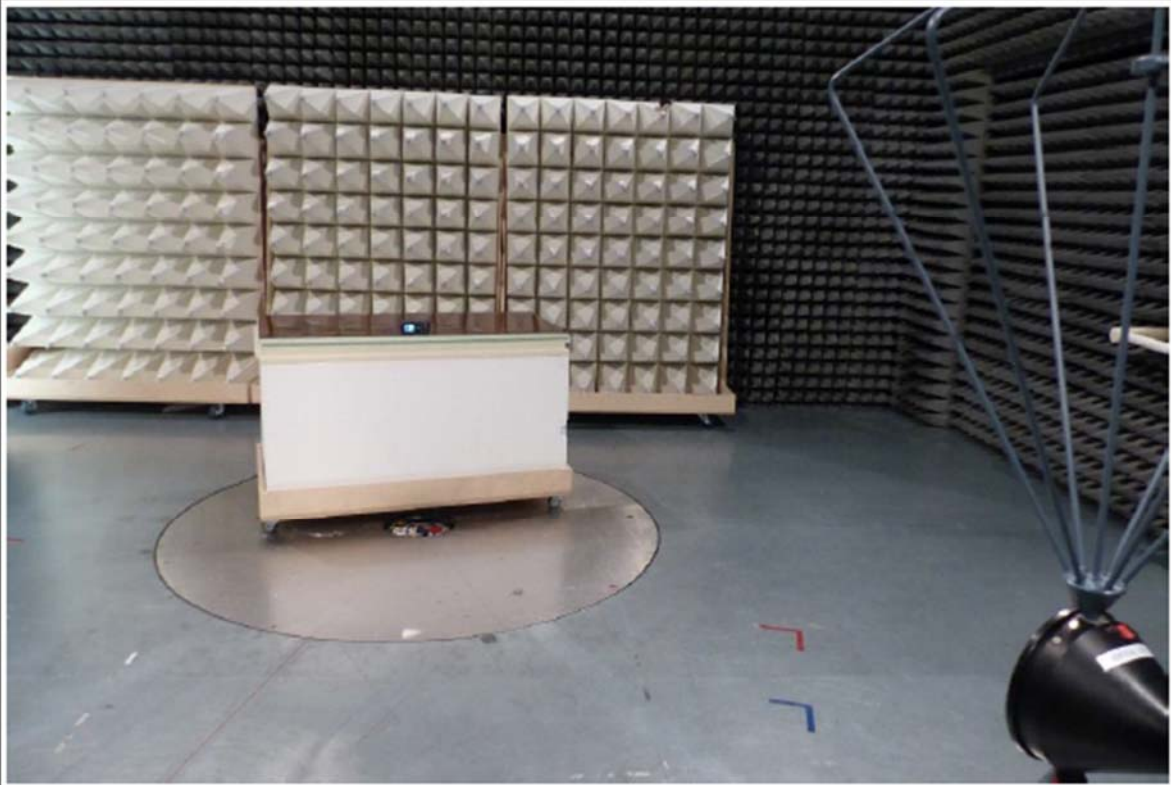
Test Setup 30-200MHz EUT configuration 1, 2
