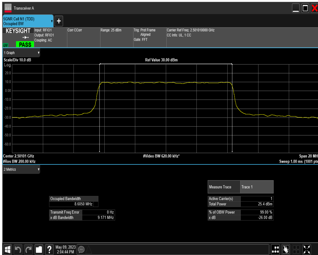
n41 SCS=30kHz DFT_QAM16 BW=10MHz Channel=500202 RB=24@0
