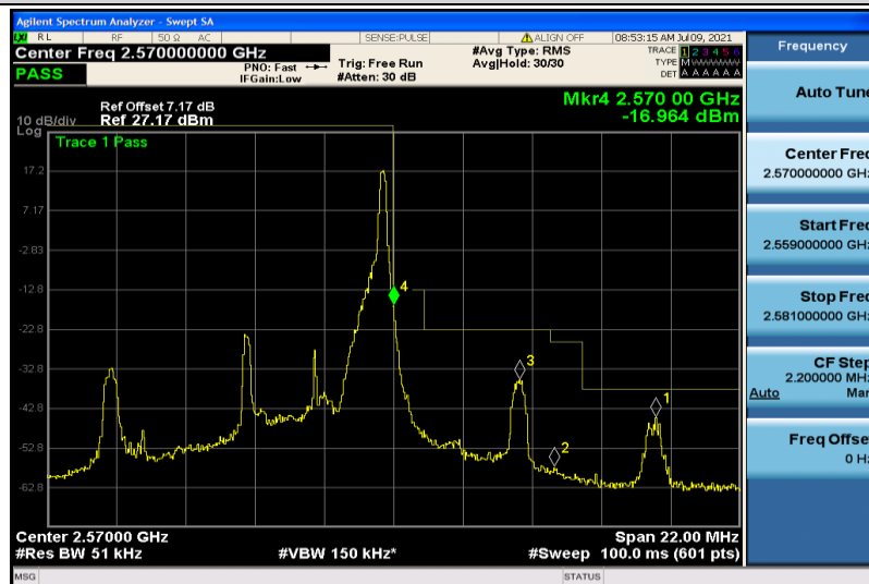
Band7-5MHz-16QAM-21425-1RB#24
