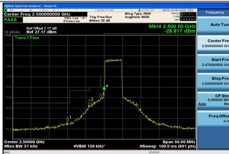
Band7-5MHz-QPSK-20775-25RB#0
