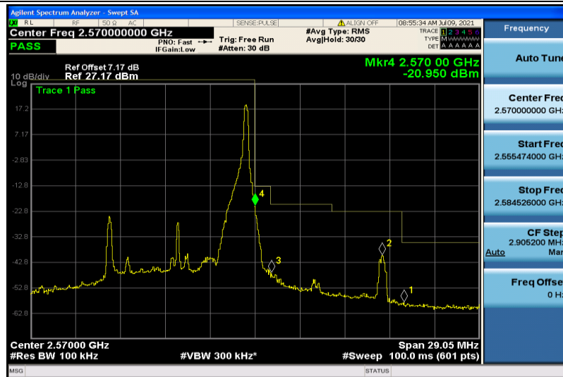
Band7-10MHz-16QAM-21400-1RB#49
