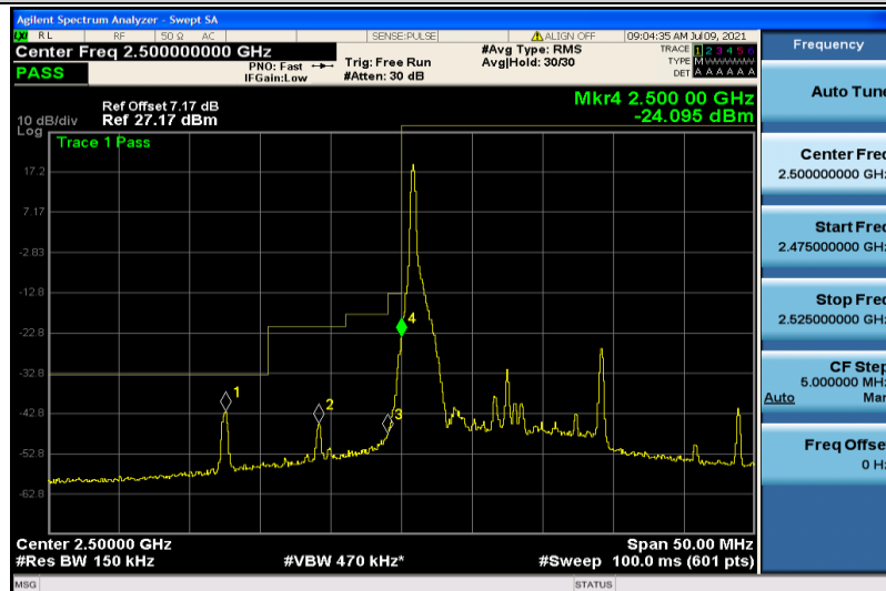
Band7-15MHz-QPSK-20825-1RB#0
