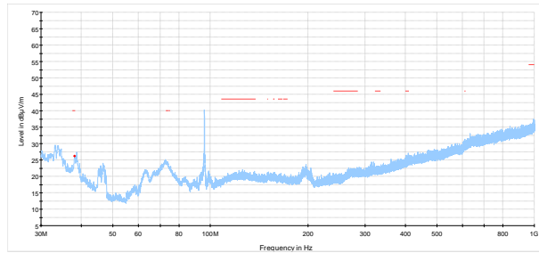
Figure 8.7-6: Radiated spurious emissions on Low channel
