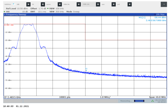
Figure 8.7-2: Conducted Band edge spurious emissions at 2483.5 MHz
