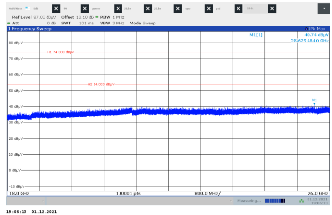
Figure 8.7-13: Radiated spurious emissions on Mid channel
