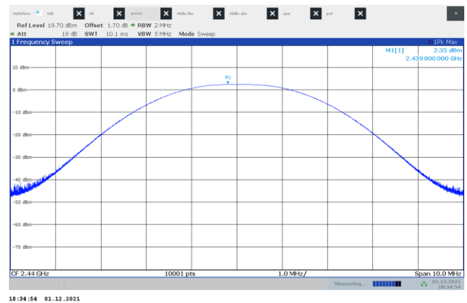
Figure 8.6-2: Output power on mid channel
