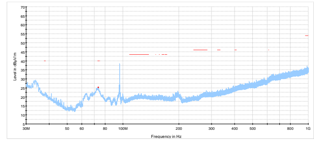
Figure 8.7-7: Radiated spurious emissions on Mid channel
