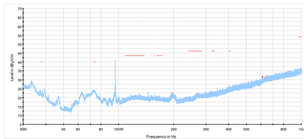
Figure 8.7-6: Radiated spurious emissions on Low channel
