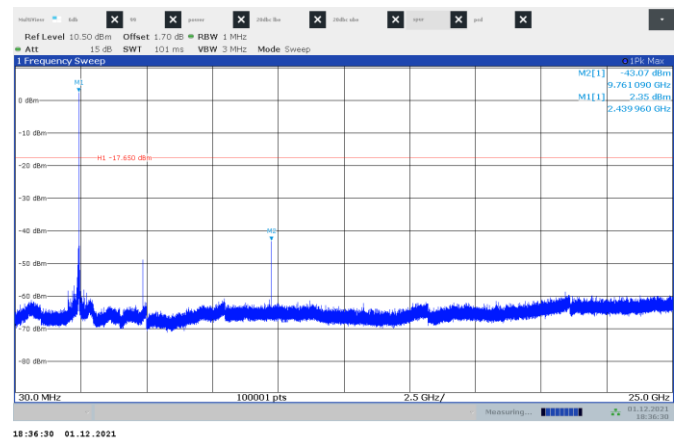
Figure 8.7-4: Conducted spurious emissions on Mid channel
