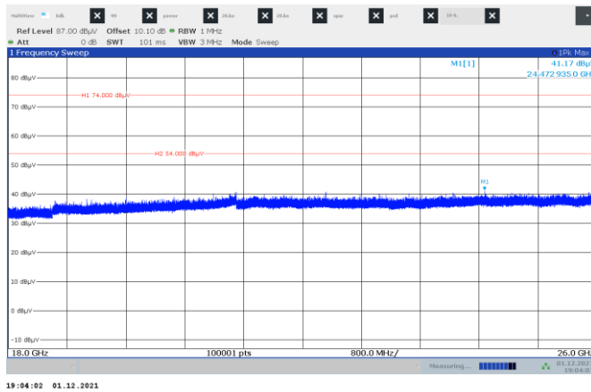
Figure 8.7-12: Radiated spurious emissions on Low channel
