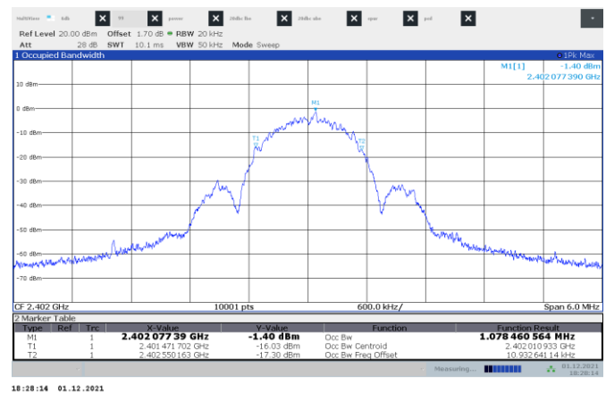
Figure 8.5-4: 99% occupied bandwidth Low channel
