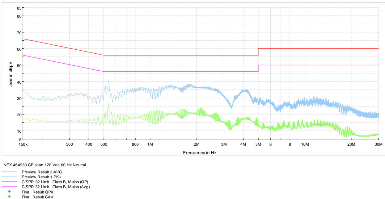
Plot 8.2-2: Conducted emissions on neutral line
