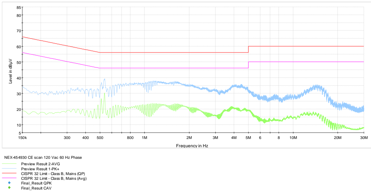
Plot 8.2-1: Conducted emissions on phase line
