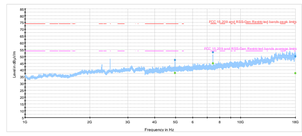
Figure 8.7-9: Radiated spurious emissions on Low channel
