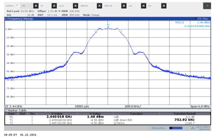
Figure 8.5-2: 6 dB bandwidth Mid channel
