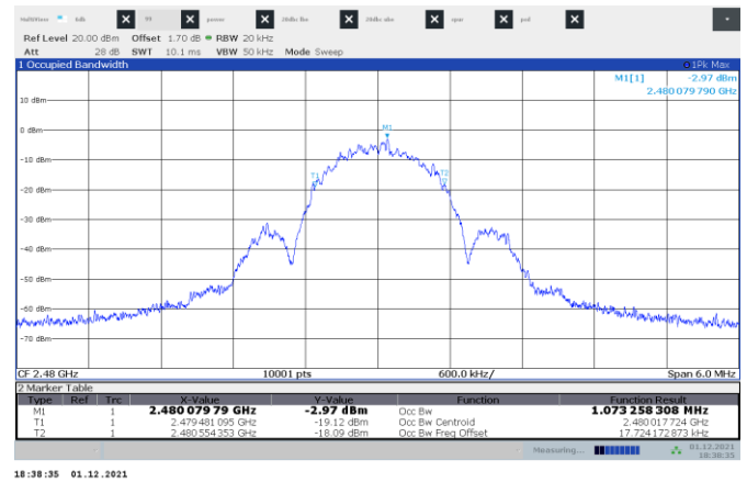
Figure 8.5-6: 99% occupied bandwidth High channel
