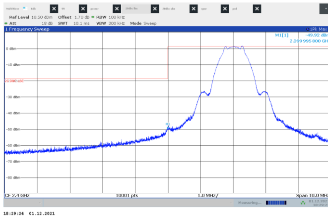
Figure 8.7-1: Conducted Band edge spurious emissions at 2400 MHz
