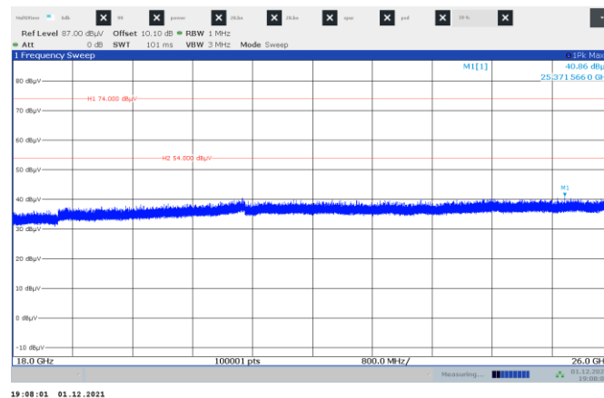
Figure 8.7-14: Radiated spurious emissions on High channel
