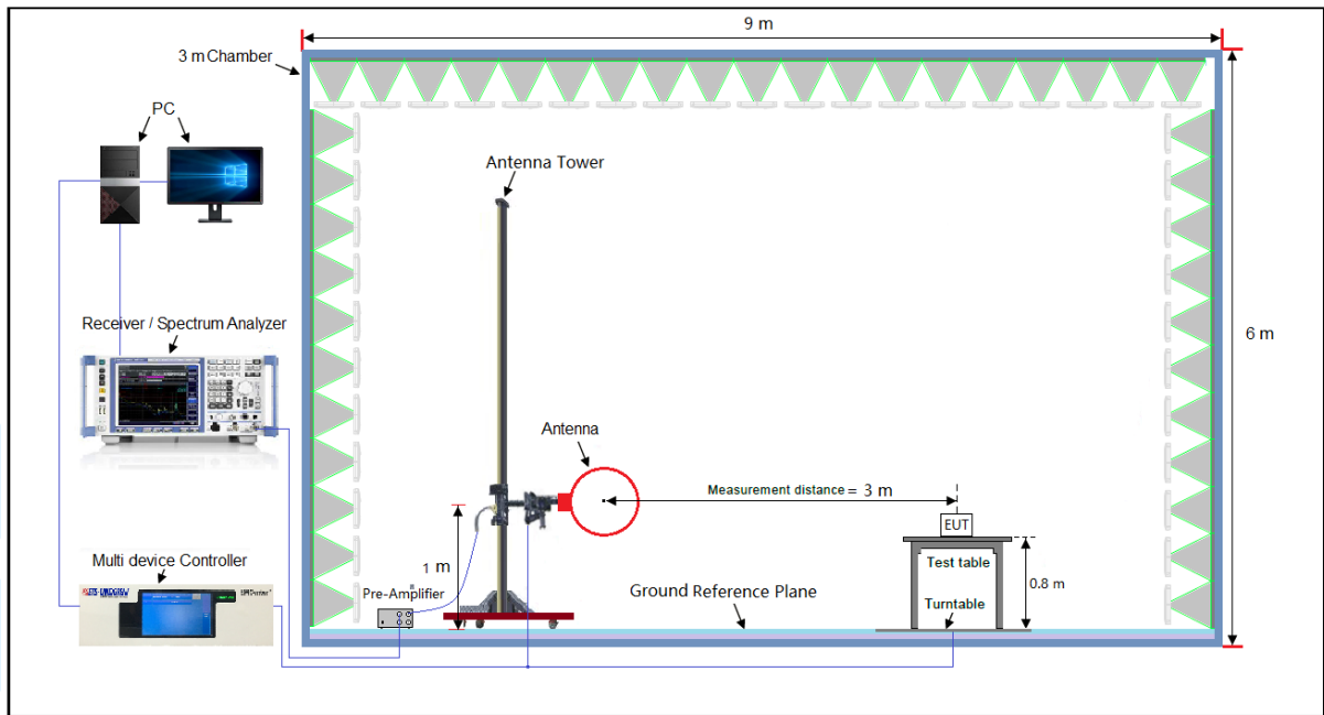
Figure 1. Below 30MHz
