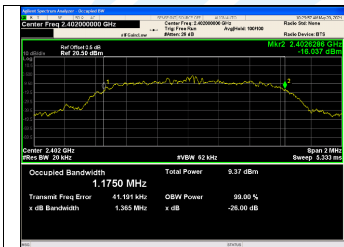
8DPSK_3-DH5_Channel 0
