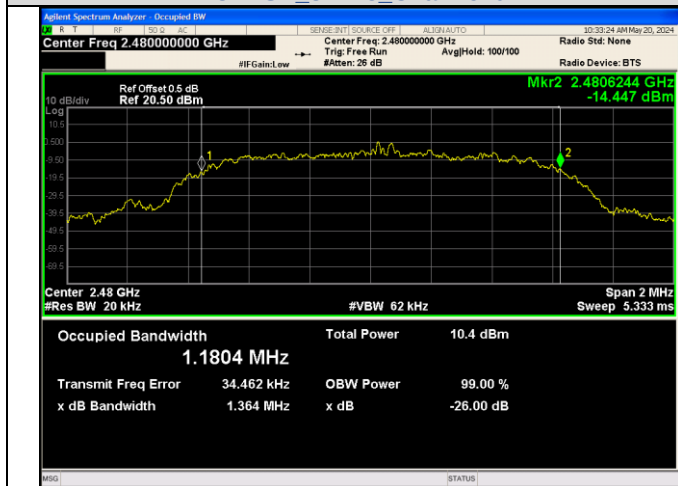
8DPSK_3-DH5_Channel 78
