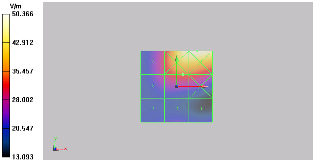
Figure 19 HAC RF E-Field GSM 1900 Channel 512
