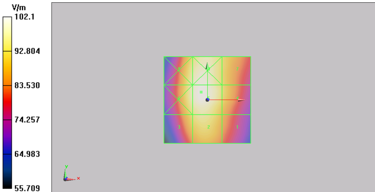
Figure 10 HAC RF E-Field GSM 850 Channel 128
