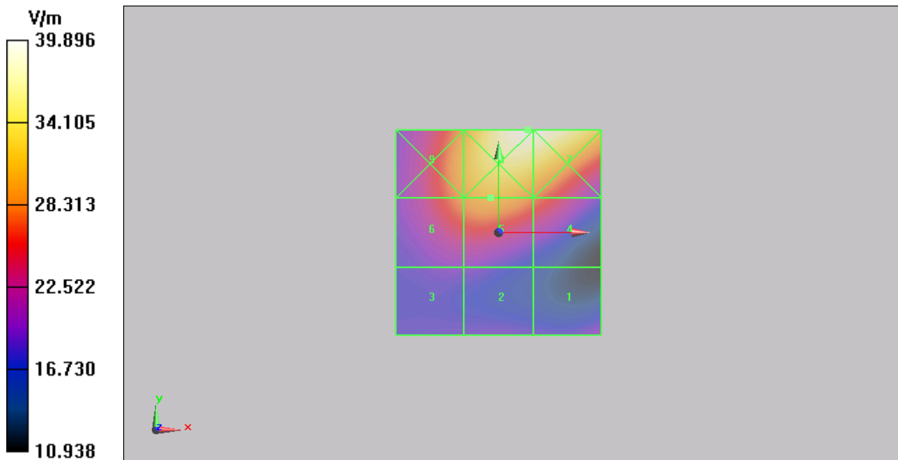
Figure 17 HAC RF E-Field GSM 1900 Channel 810
