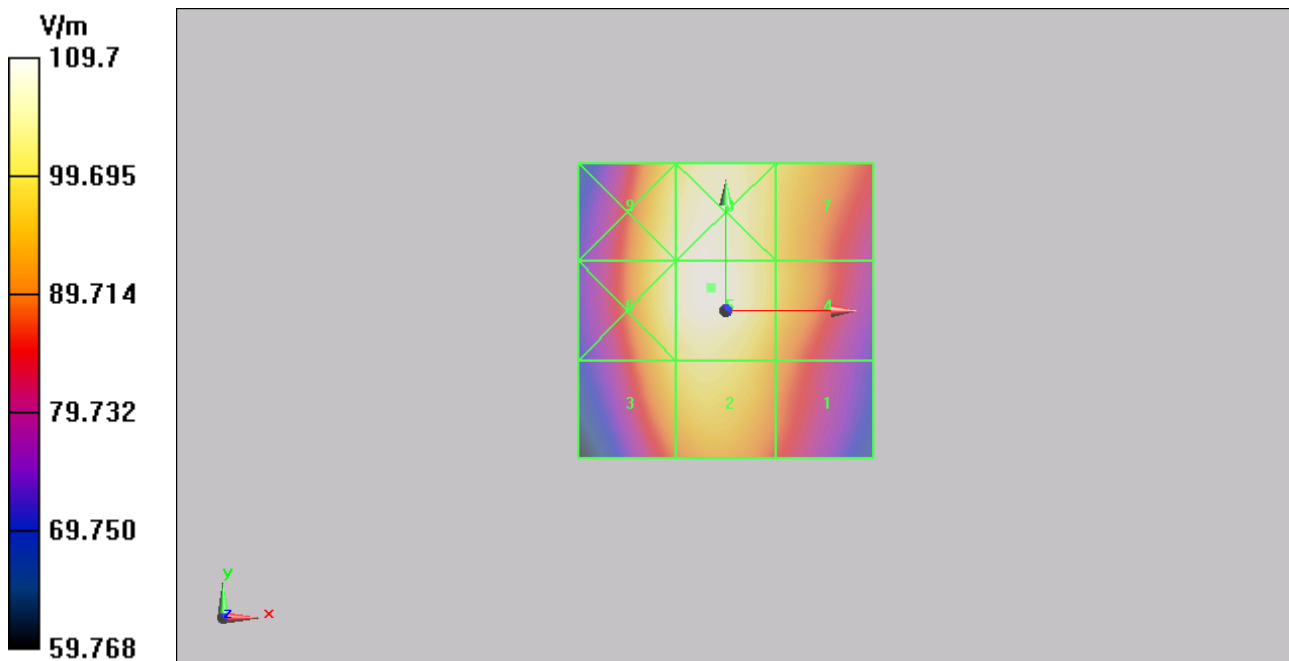
Figure 9 HAC RF E-Field GSM 850 Channel 190
