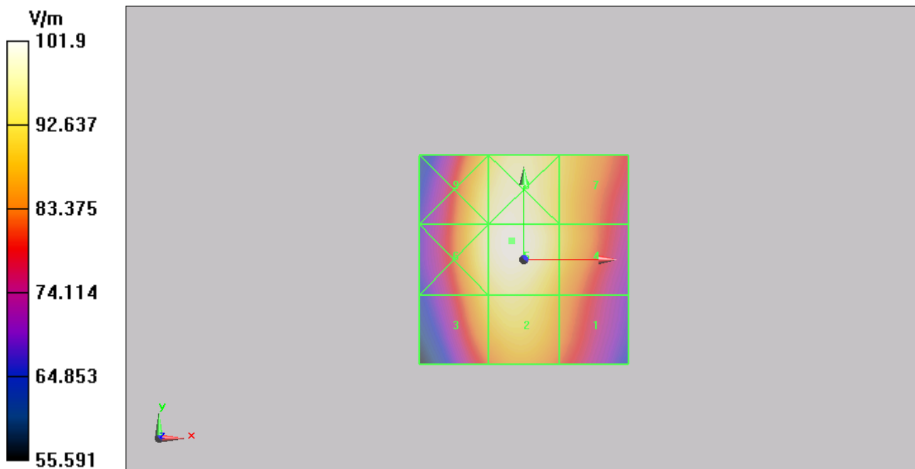
Figure 13 HAC RF E-Field GSM 850 Channel 128
