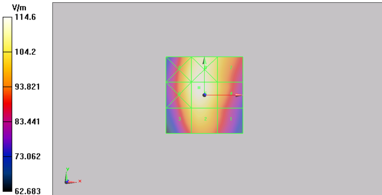
Figure 11 HAC RF E-Field GSM 850 Channel 251
