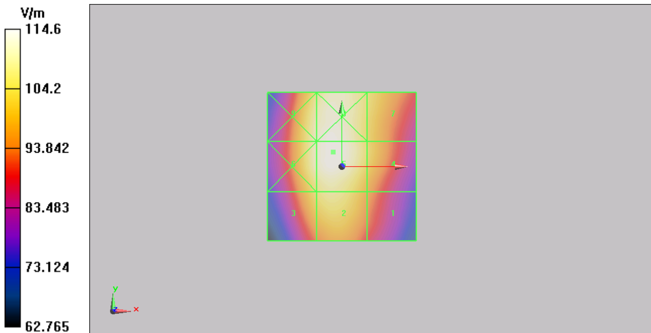
Figure 8 HAC RF E-Field GSM 850 Channel 251
