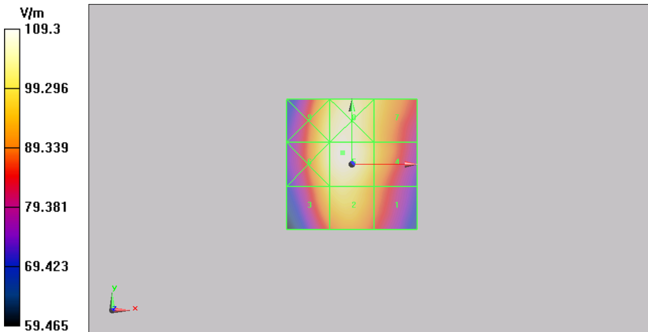
Figure 12 HAC RF E-Field GSM 850 Channel 190
