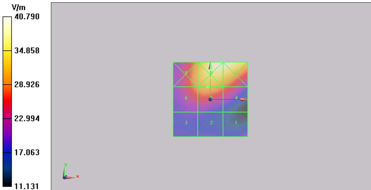
Figure 14 HAC RF E-Field GSM 1900 Channel 810
