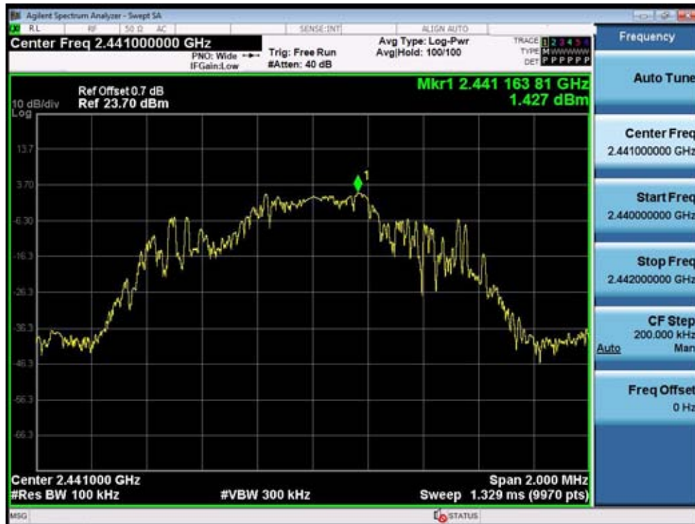
(Plot 4.9.3 B1: Channel 39: 2441MHz @ 8DPSK)
