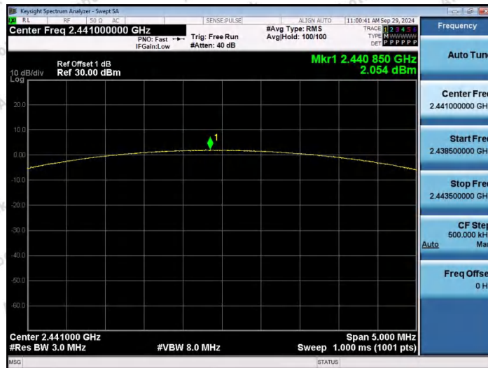
DH5-Ant1-2441-PASS
