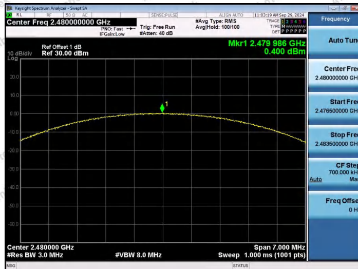
2DH5-Ant1-2480-PASS
