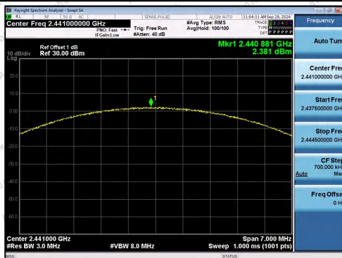
3DH5-Ant1-2441-PASS
