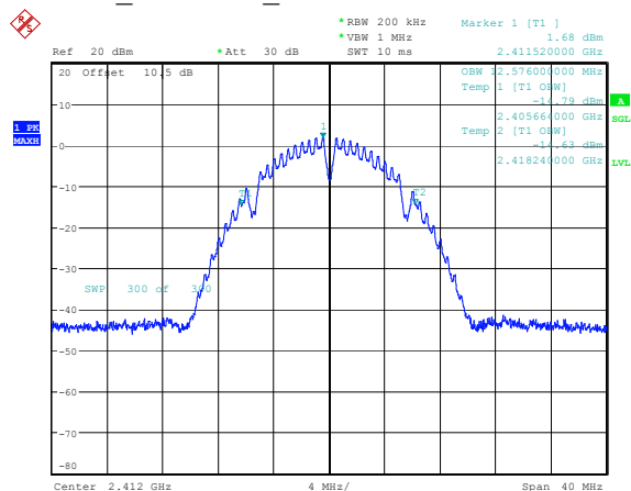
b 2412MHz Chain 0 12.576MHz
