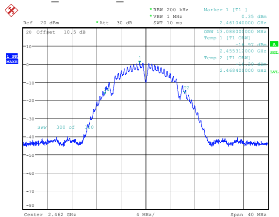
b 2462MHz Chain 1 13.088MHz
