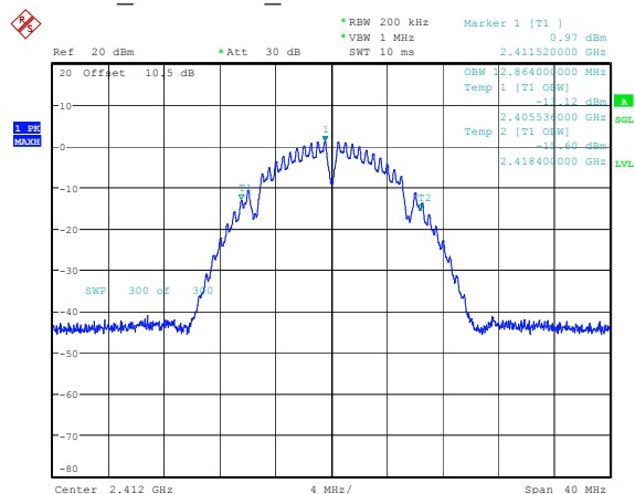
b 2412MHz Chain 1 12.864MHz
