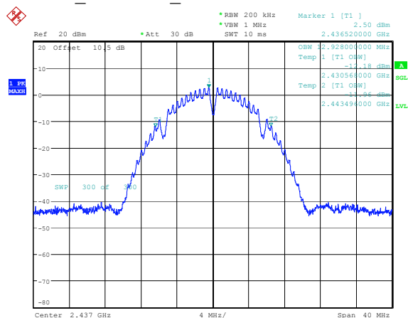
b 2437MHz Chain 0 12.928MHz
