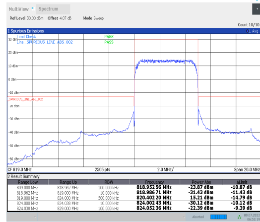
1-N26-814-824--15-5-H-3-DFT-PI2BPSK-Outer_F ull-25@0-Ant0-PASS-see graph
