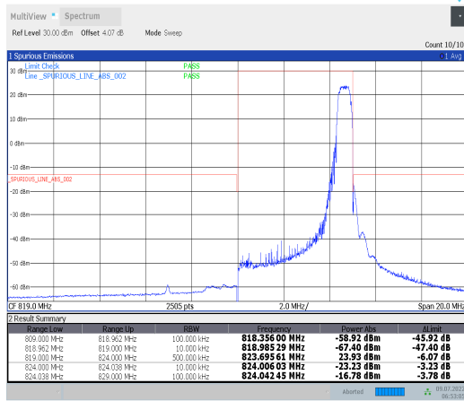
1-N26-814-824--15-5-H-2-DFT-PI2BPSK-Edge_1RB_R ight-1@24-Ant0-PASS-see graph
