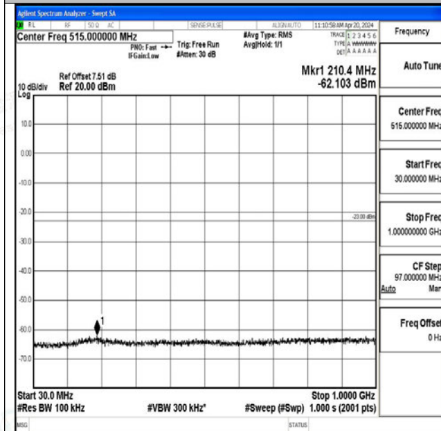
Band25_1.4MHz_QPSK_26683_1RB#0_30~1000_30~10
