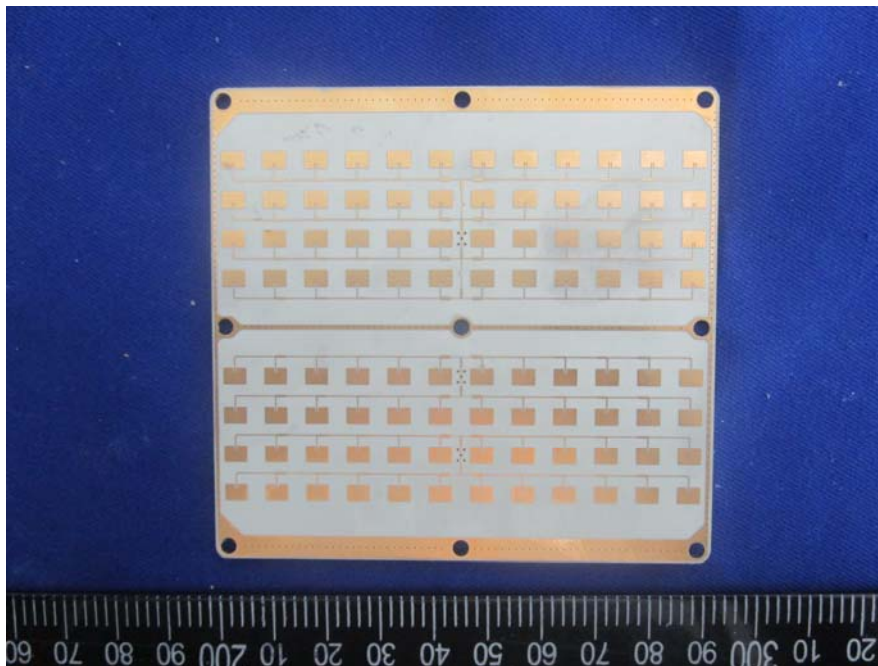
EUT – Ant Top View
