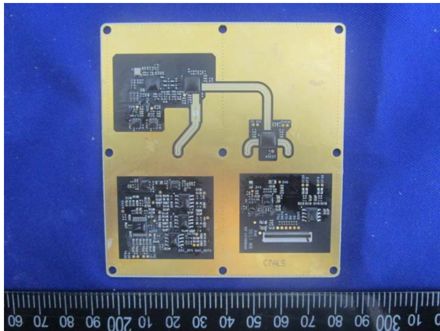
EUT – Ant Bottom View
