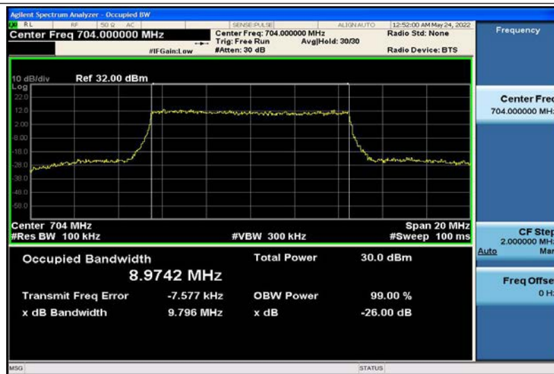
Band12-10MHz-16QAM-23060-50RB#0-8.9742
