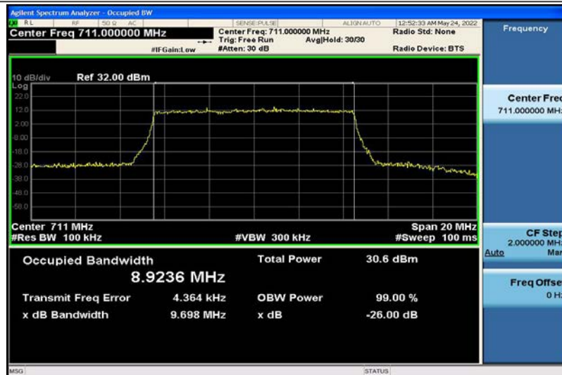
Band12-10MHz-QPSK-23130-50RB#0-8.9236
