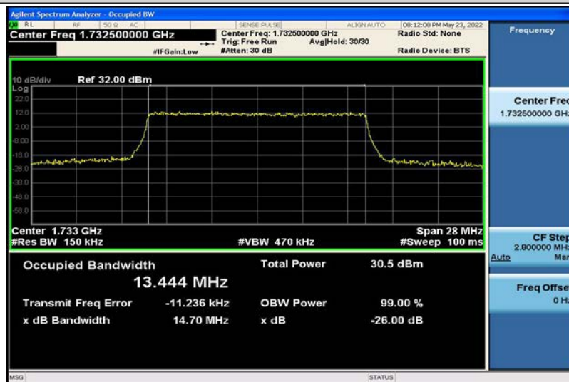
Band4-15MHz-16QAM-20175-75RB#0-13.444
