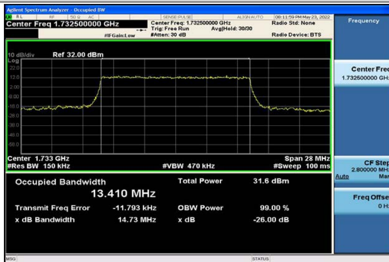
Band4-15MHz-QPSK-20175-75RB#0-13.410
