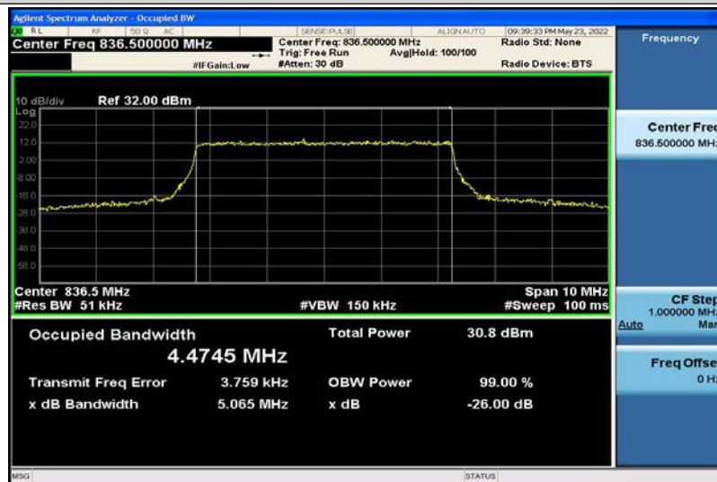
Band5-5MHz-QPSK-20525-25RB#0-4.4745
