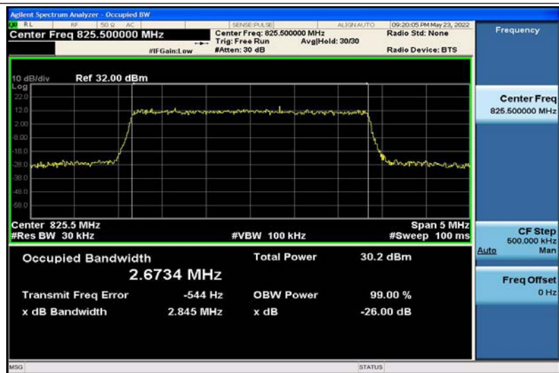
Band5-3MHz-QPSK-20415-15RB#0-2.6734
