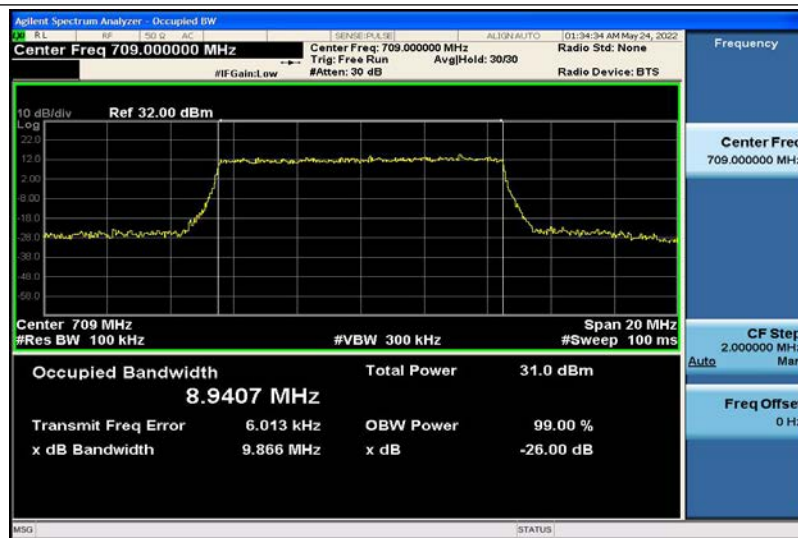
Band17-10MHz-QPSK-23780-50RB#0-8.9407
