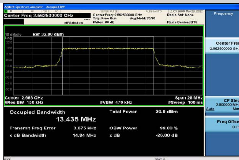
Band7-15MHz-QPSK-21375-75RB#0-13.435
