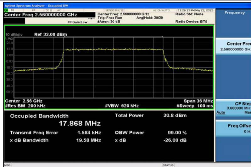
Band7-20MHz-QPSK-21350-100RB#0-17.868
