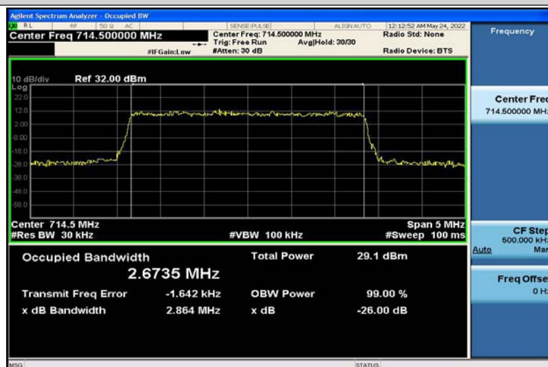
Band12-3MHz-16QAM-23165-15RB#0-2.6735
