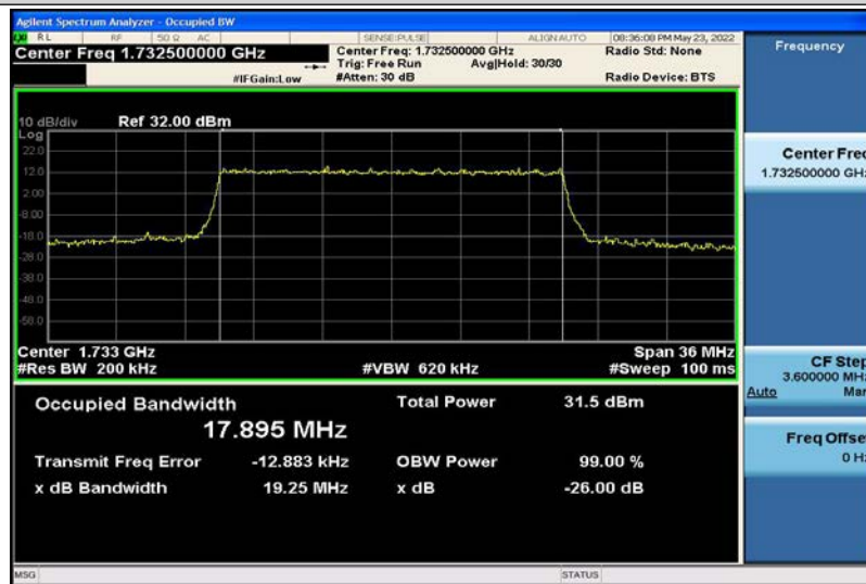
Band4-20MHz-QPSK-20175-100RB#0-17.895
