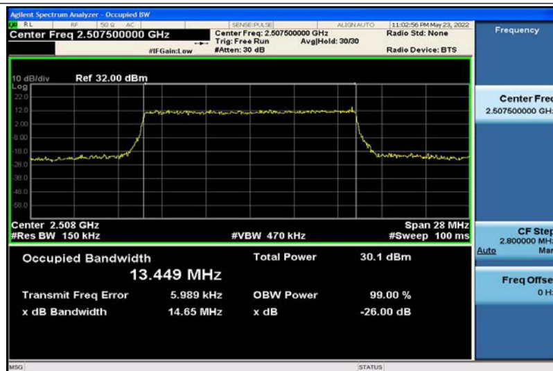
Band7-15MHz-16QAM-20825-75RB#0-13.449
