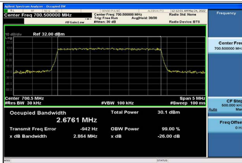
Band12-3MHz-QPSK-23025-15RB#0-2.6761
