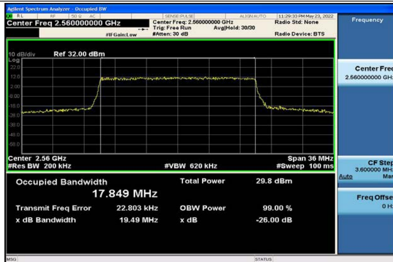
Band7-20MHz-16QAM-21350-100RB#0-17.849
