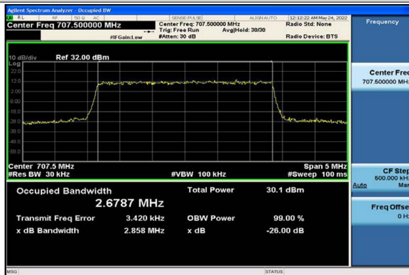
Band12-3MHz-QPSK-23095-15RB#0-2.6787
