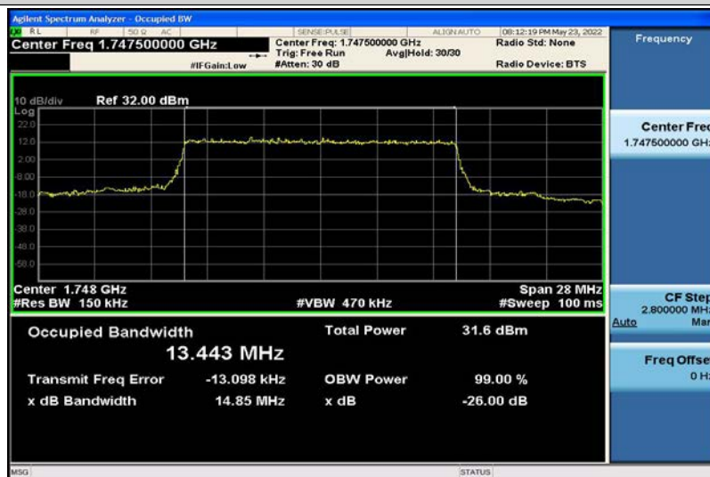
Band4-15MHz-QPSK-20325-75RB#0-13.443
