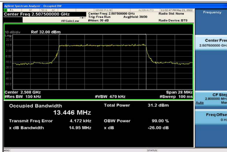
Band7-15MHz-QPSK-20825-75RB#0-13.446
