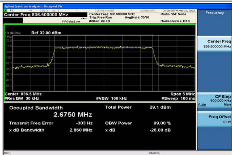
Band5-3MHz-16QAM-20525-15RB#0-2.6750
