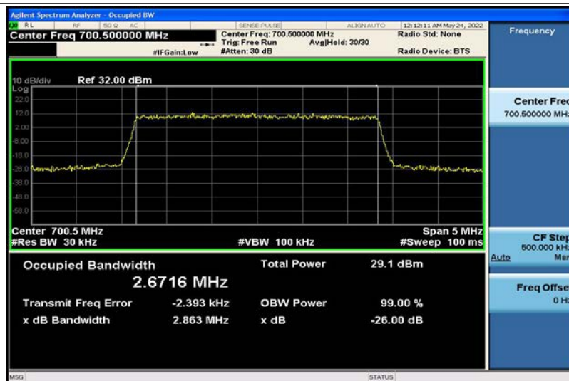
Band12-3MHz-16QAM-23025-15RB#0-2.6716
