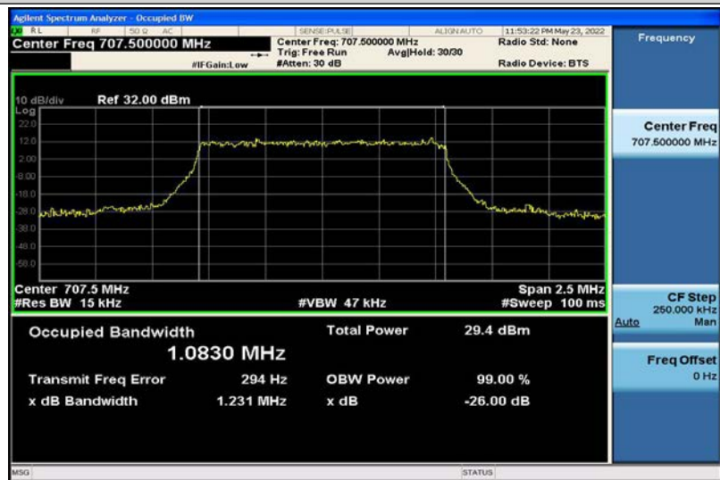
Band12-1.4MHz-QPSK-23095-6RB#0-1.0830
