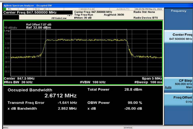
Band5-3MHz-16QAM-20635-15RB#0-2.6712
