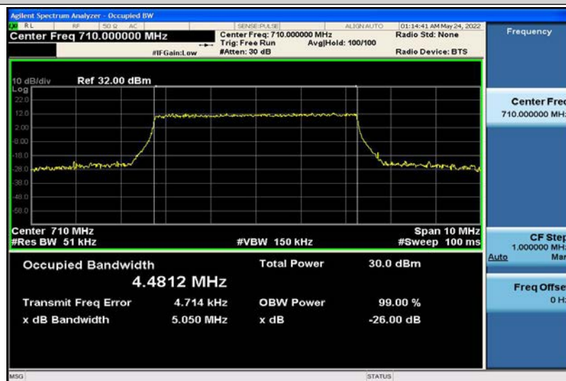
Band17-5MHz-16QAM-23790-25RB#0-4.4812
