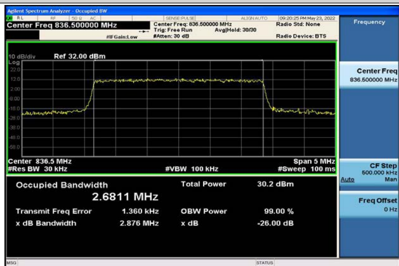
Band5-3MHz-QPSK-20525-15RB#0-2.6811
