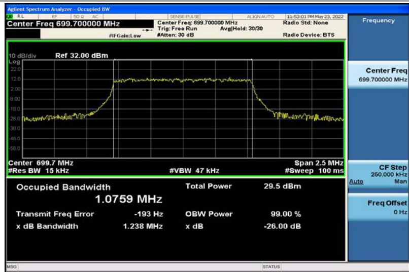
Band12-1.4MHz-QPSK-23017-6RB#0-1.0759
