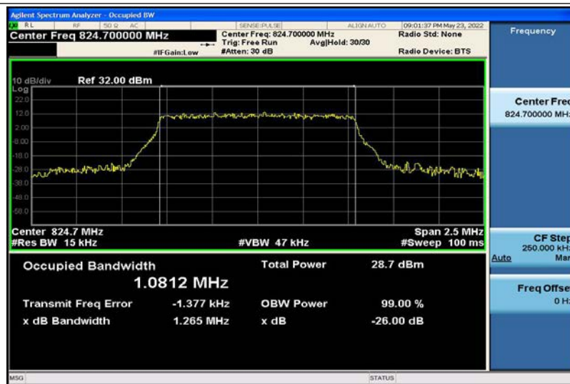
Band5-1.4MHz-16QAM-20407-6RB#0-1.0812
