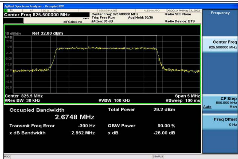
Band5-3MHz-16QAM-20415-15RB#0-2.6748
