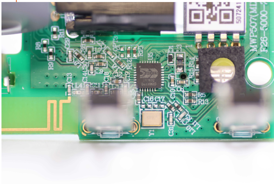
SRD&amp;BLE Antenna
