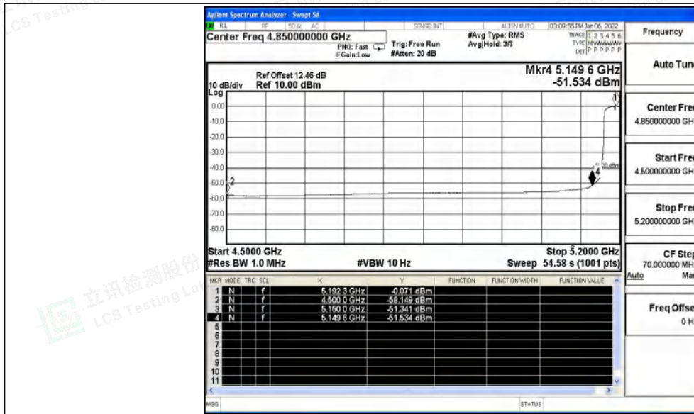
11N40SISO_Ant1_Low_5190_Peak
