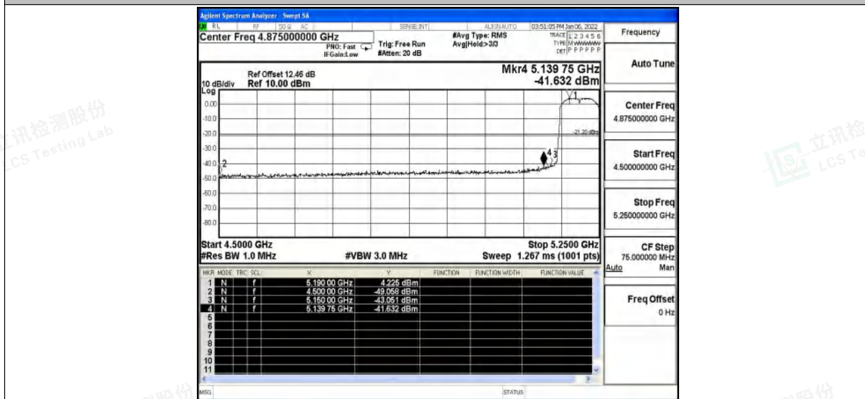
11AC80SISO_Ant1_High_5210_AV
