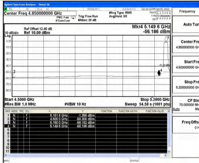
11A_Ant0_Low_5180_Peak
