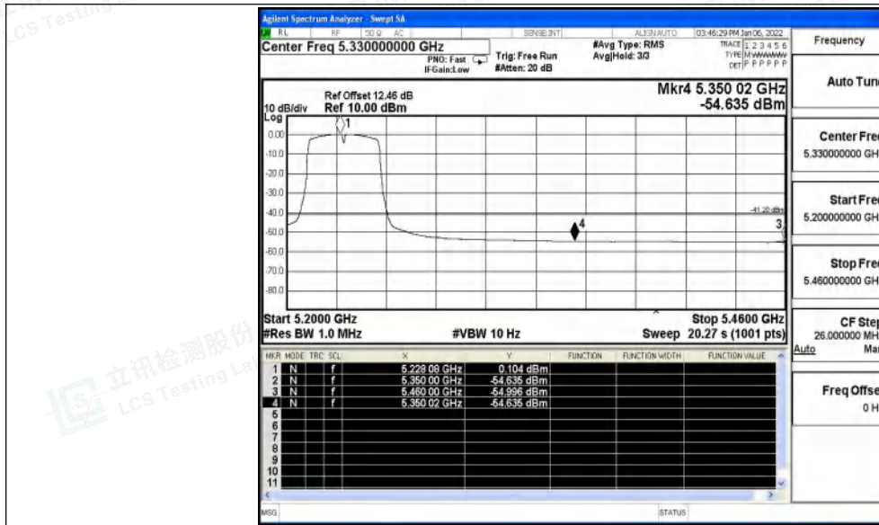
11AC40SISO_Ant1_High_5230_Peak
