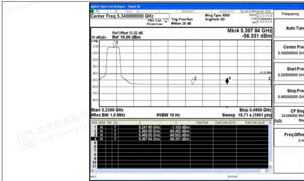
11A_Ant0_High_5240_Peak
