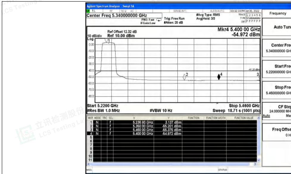
11AC20SISO_Ant1_High_5240_Peak
