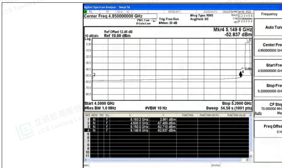
11AC20SISO_Ant1_Low_5180_Peak
