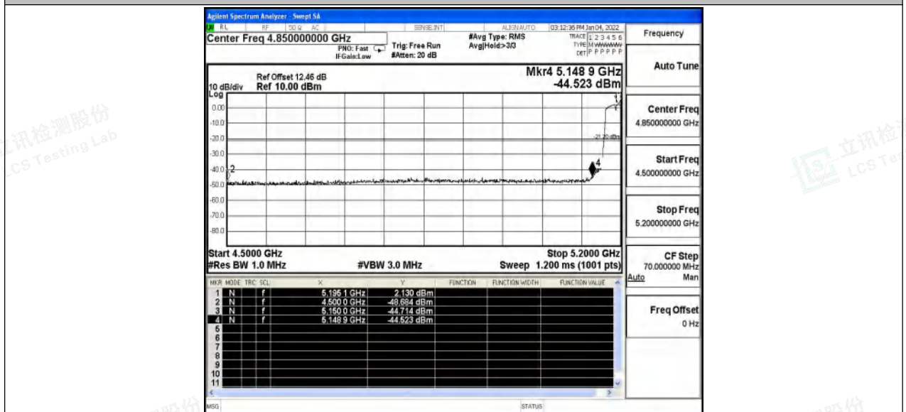
11AC40SISO_Ant0_High_5230_AV
