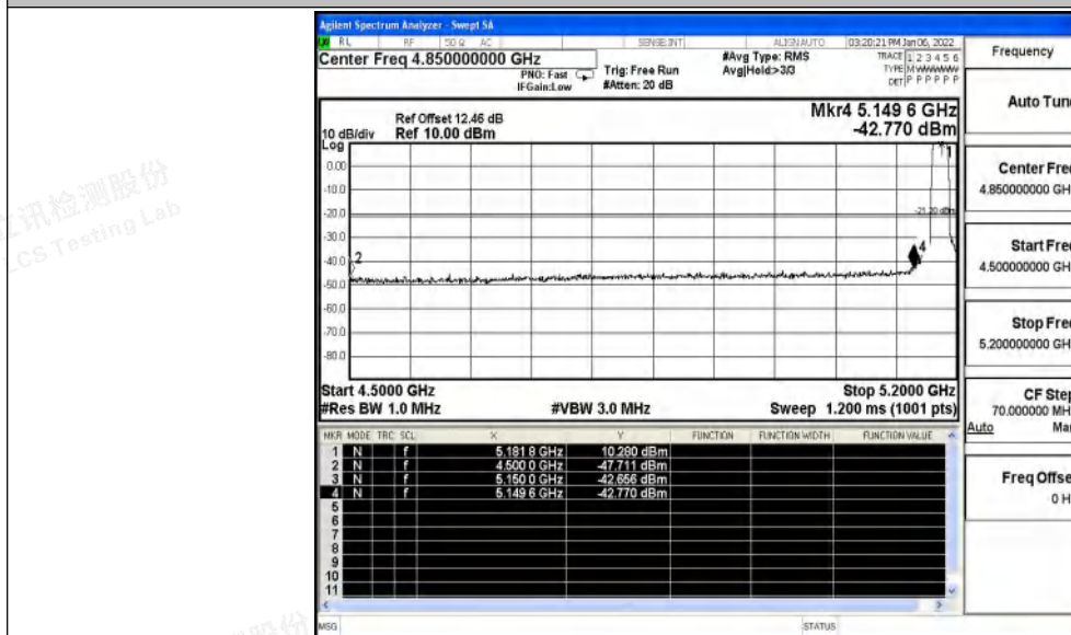
11AC20SISO_Ant1_High_5240_AV
