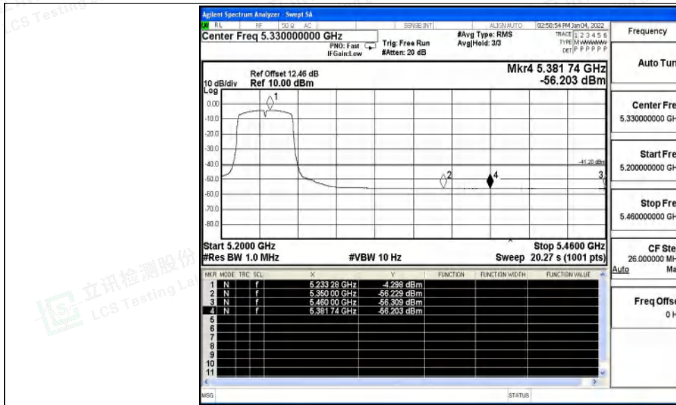
11N40SISO_Ant0_High_5230_Peak
