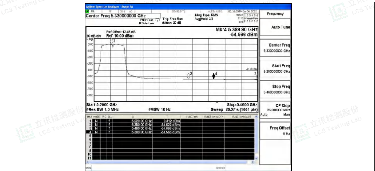
11N40SISO_Ant1_High_5230_Peak
