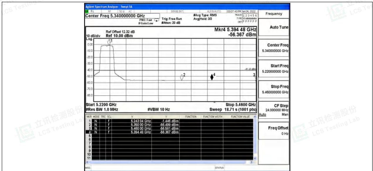
11AC20SISO_Ant0_High_5240_Peak
