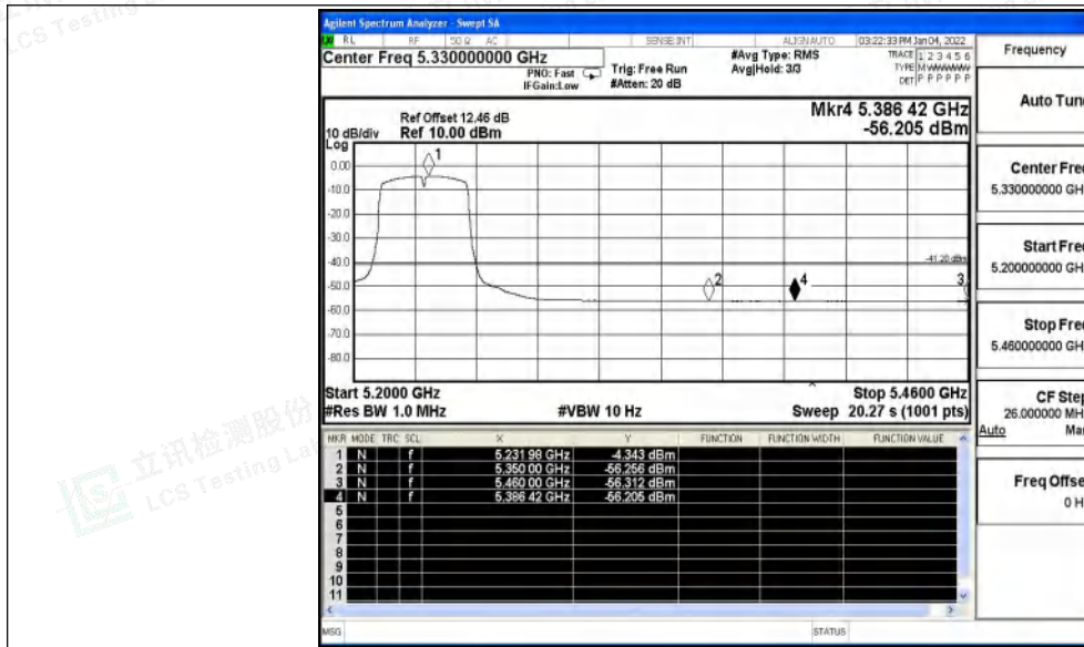
11AC40SISO_Ant0_High_5230_Peak
