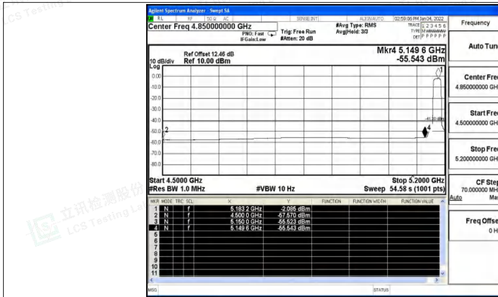
11AC20SISO_Ant0_Low_5180_Peak
