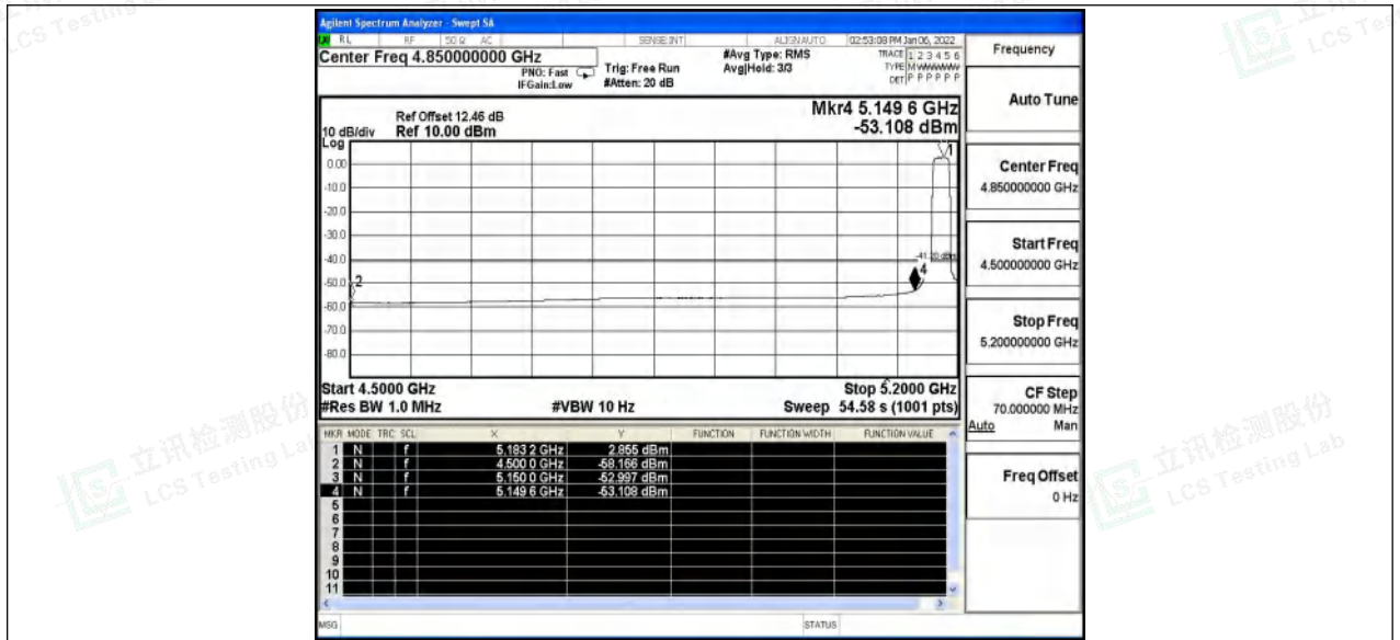
11N20SISO_Ant1_Low_5180_Peak
