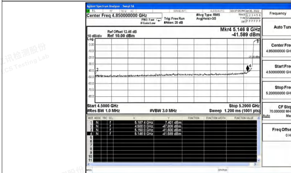
11AC40SISO_Ant1_High_5230_AV
