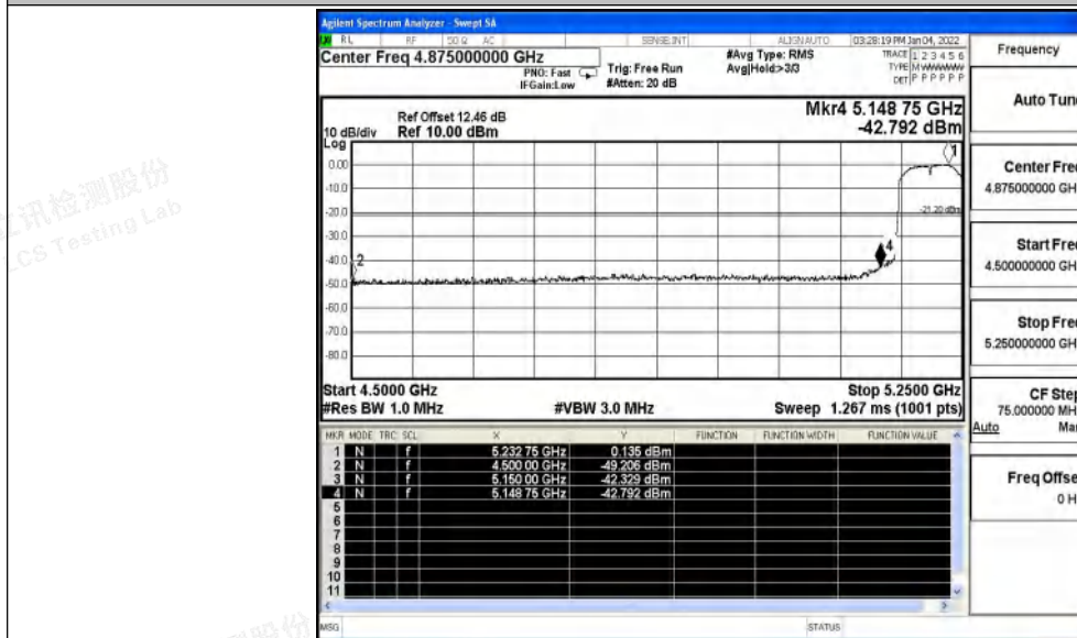
11AC80SISO_Ant0_High_5210_AV
