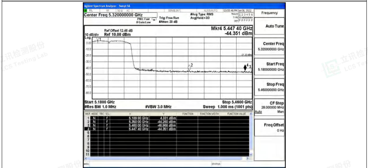
11AC80SISO_Ant1_High_5210_Peak
