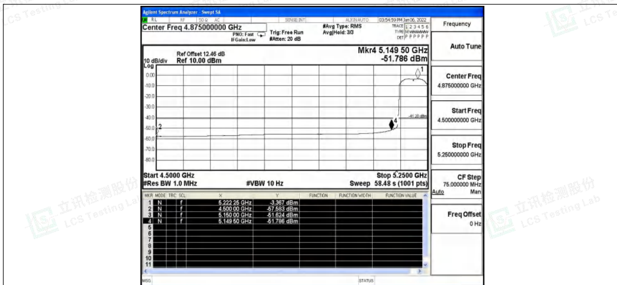
11AC80SISO_Ant1_Low_5210_Peak
