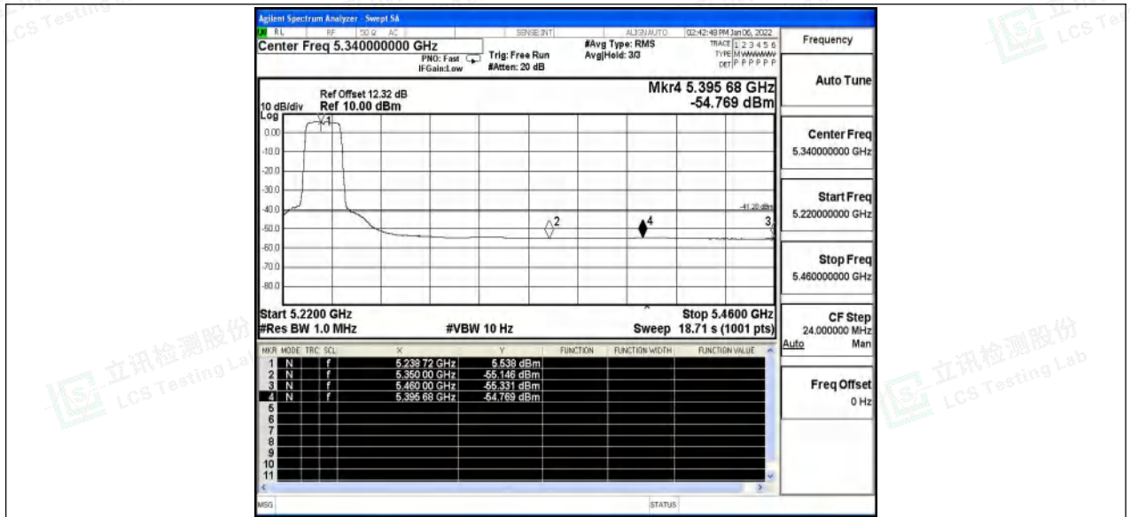
11A_Ant1_High_5240_Peak
