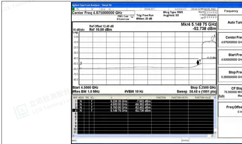
11AC80SISO_Ant0_Low_5210_Peak
