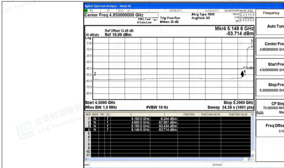
11N40SISO_Ant0_Low_5190_Peak
