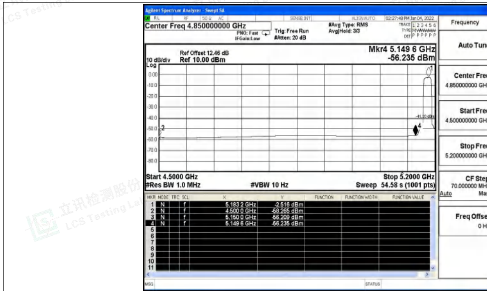
11N20SISO_Ant0_Low_5180_Peak
