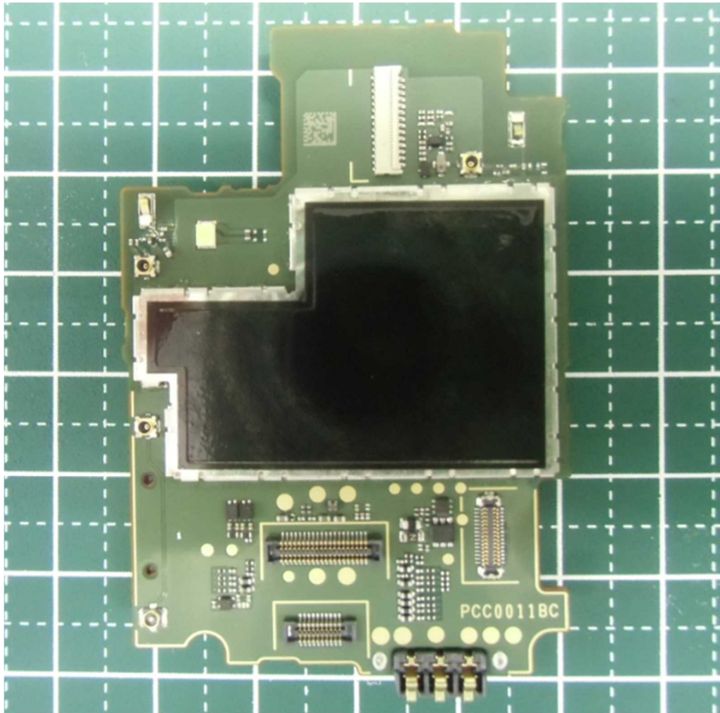
Main PCB front
