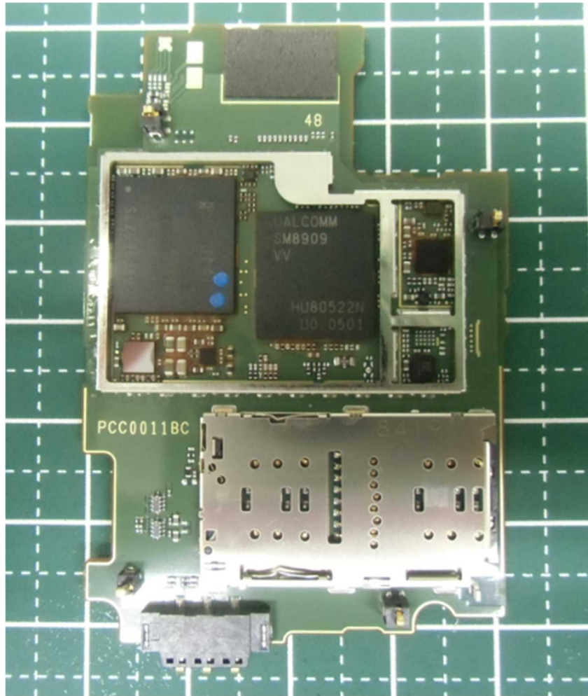
Main PCB without shield rear
