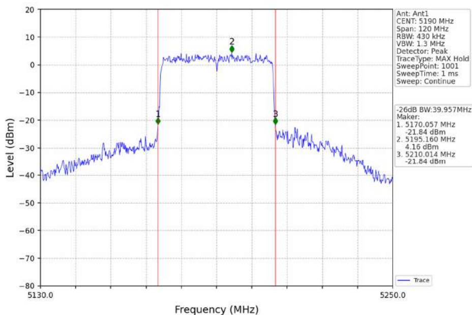
802.11ax(HEW40) LCH_5190MHz RU484 Left Ant1 NTVN
