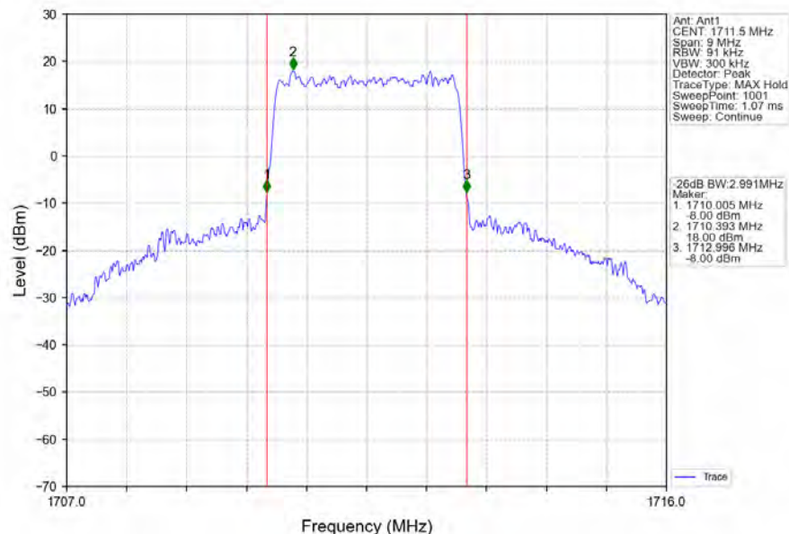
Band66_3MHz_64QAM_LCH_1711.5MHz_RB_15_0_NTNV
