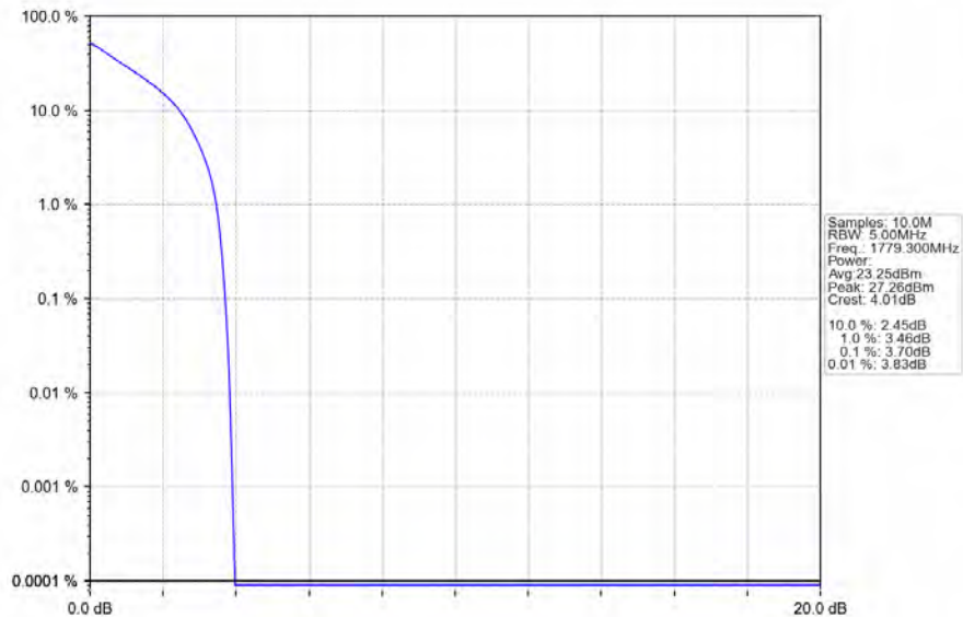
Band66_1.4MHz_QPSK_HCH_1779.3MHz_RB_6_0_NTNV
