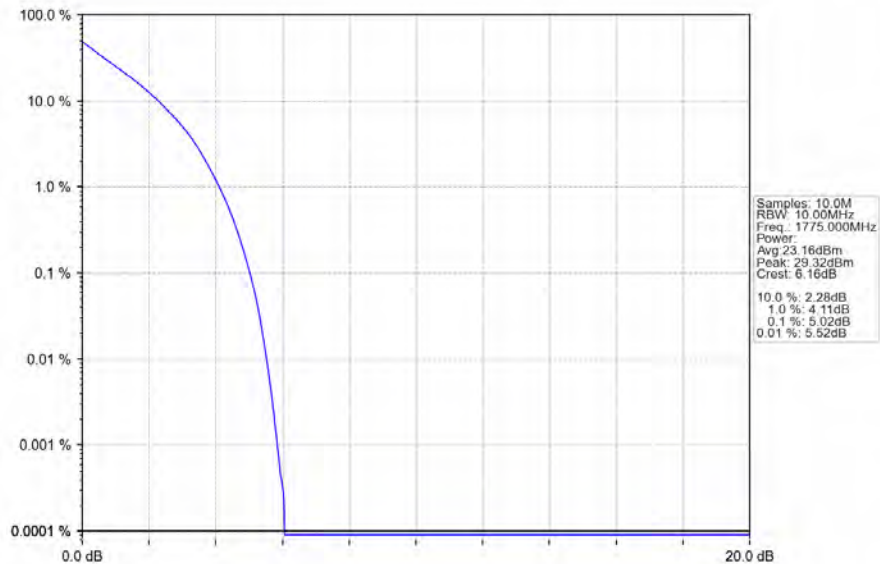
Band66_10MHz_QPSK_HCH_1775MHz_RB_50_0_NTNV
