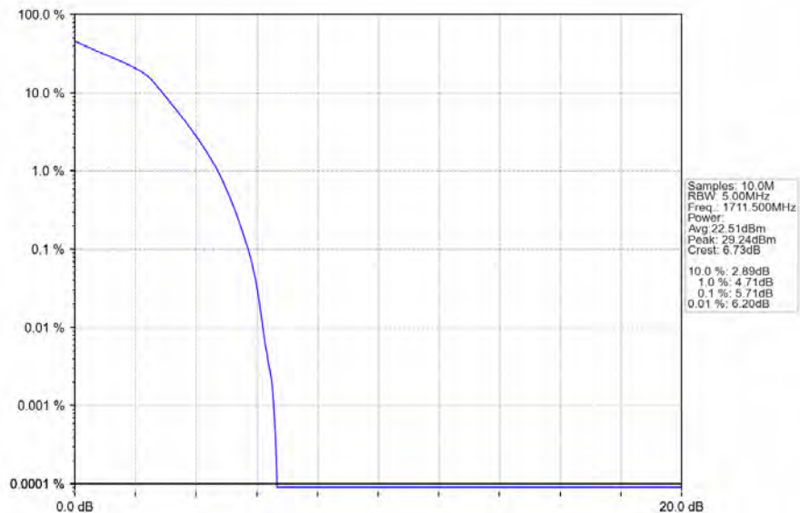
Band66_3MHz_16QAM_LCH_1711.5MHz_RB_15_0_NTNV
