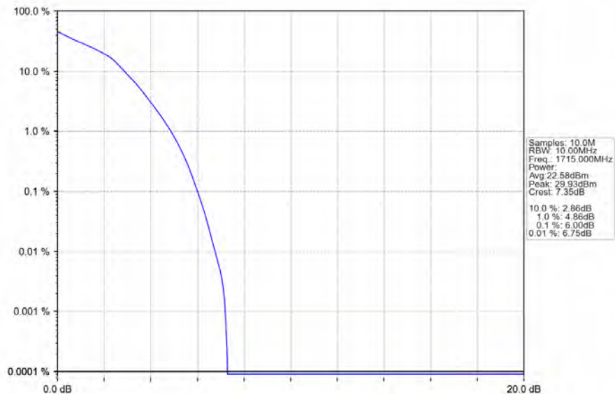
Band66_10MHz_16QAM_LCH_1715MHz_RB_50_0_NTNV
