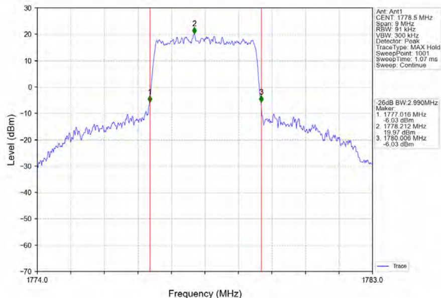
Band66_3MHz_QPSK_HCH_1778.5MHz_RB_15_0_NTNV
