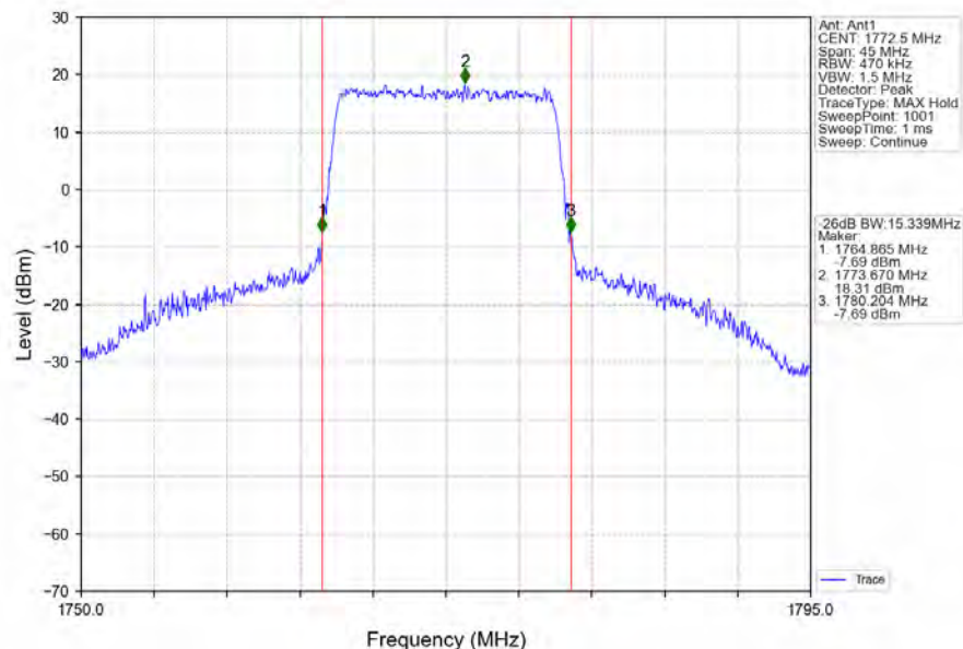
Band66_15MHz_16QAM_HCH_1772.5MHz_RB_75_0_NTNV
