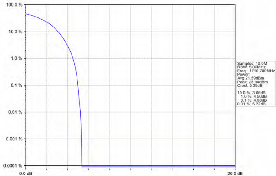
Band66_1.4MHz_64QAM_LCH_1710.7MHz_RB_6_0_NTNV
