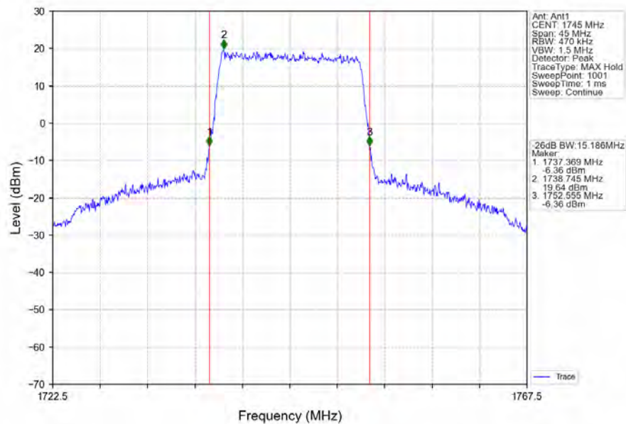
Band66_15MHz_QPSK_MCH_1745MHz_RB_75_0_NTNV
