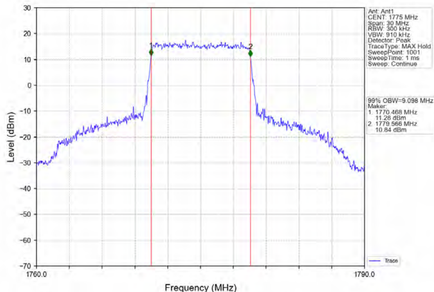
Band66_10MHz_64QAM_HCH_1775MHz_RB_50_0_NTNV
