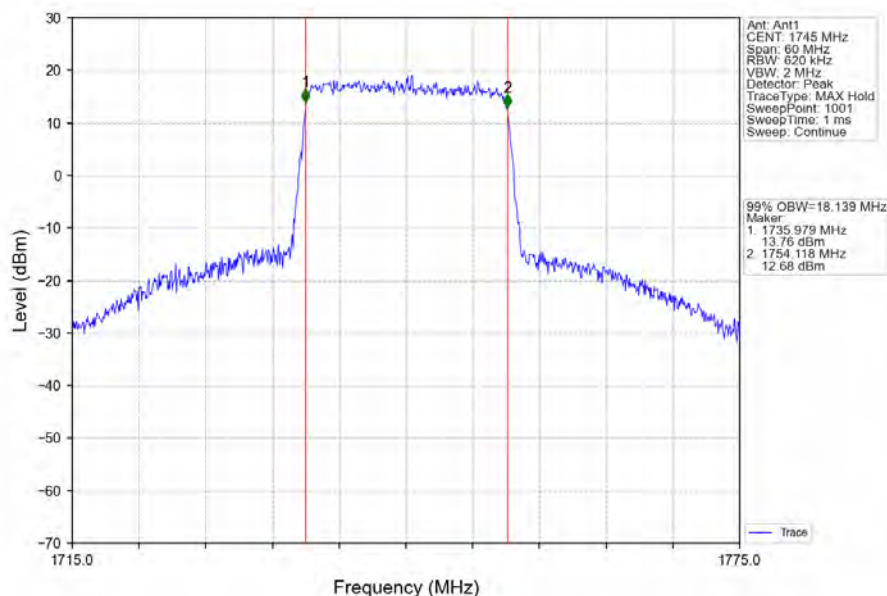
Band66_20MHz_16QAM_MCH_1745MHz_RB_100_0_NTNV
