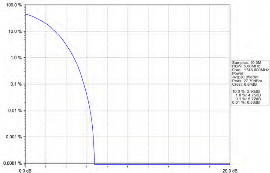
Band66_5MHz_64QAM_MCH_1745MHz_RB_25_0_NTNV
