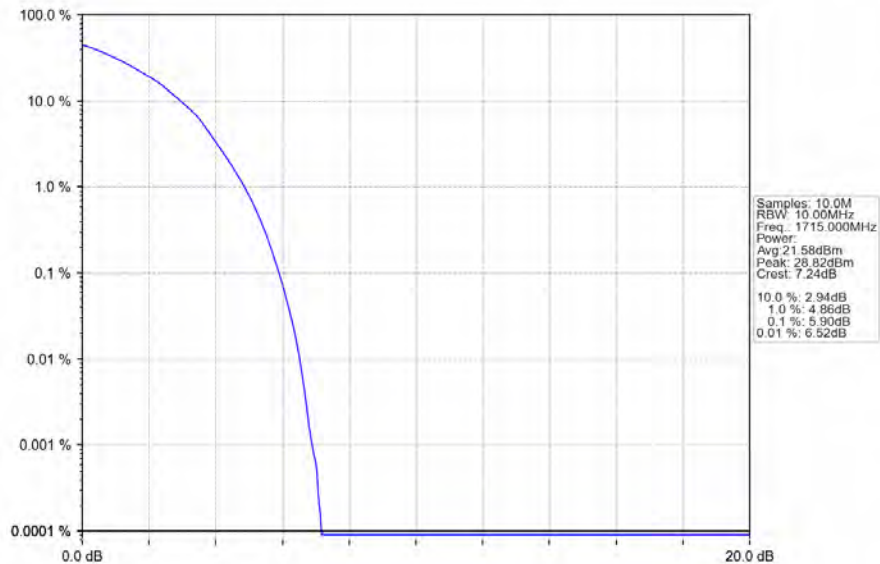
Band66_10MHz_64QAM_LCH_1715MHz_RB_50_0_NTNV
