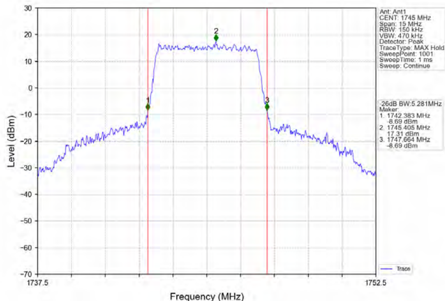
Band66_5MHz_64QAM_MCH_1745MHz_RB_25_0_NTNV
