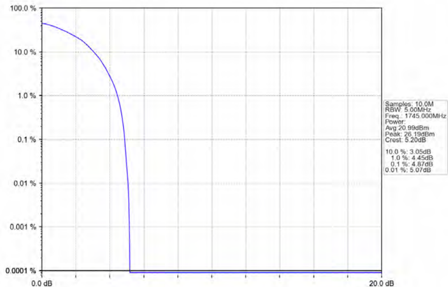
Band66_1.4MHz_64QAM_MCH_1745MHz_RB_6_0_NTNV
