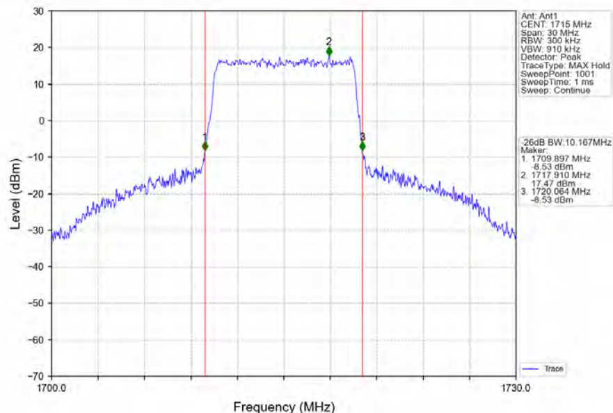
Band66_10MHz_64QAM_LCH_1715MHz_RB_50_0_NTNV
