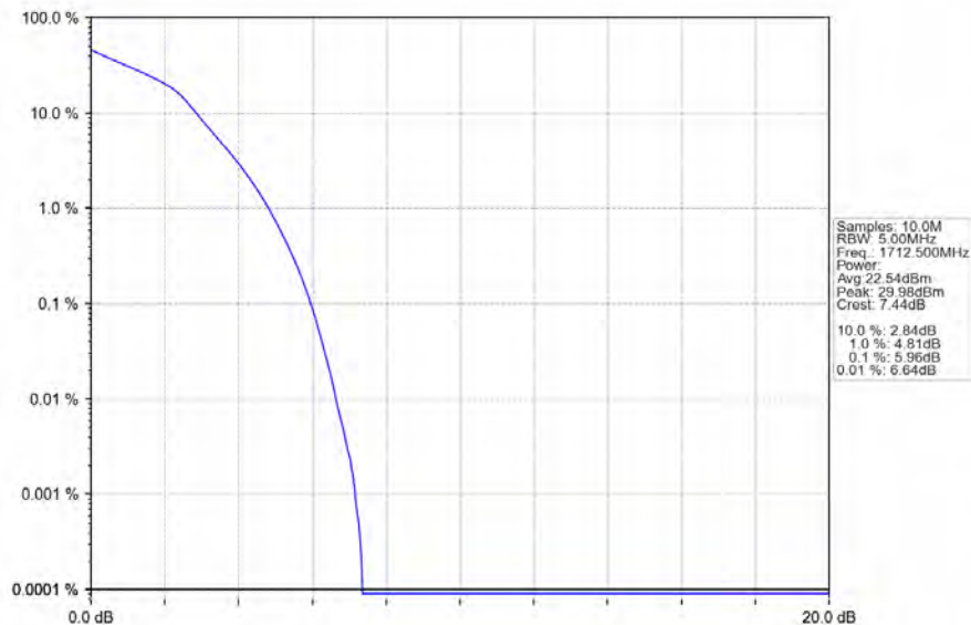
Band66_5MHz_16QAM_LCH_1712.5MHz_RB_25_0_NTNV
