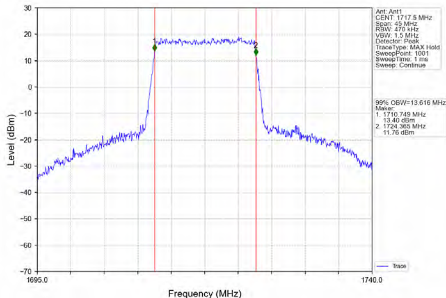
Band66_15MHz_16QAM_LCH_1717.5MHz_RB_75_0_NTNV
