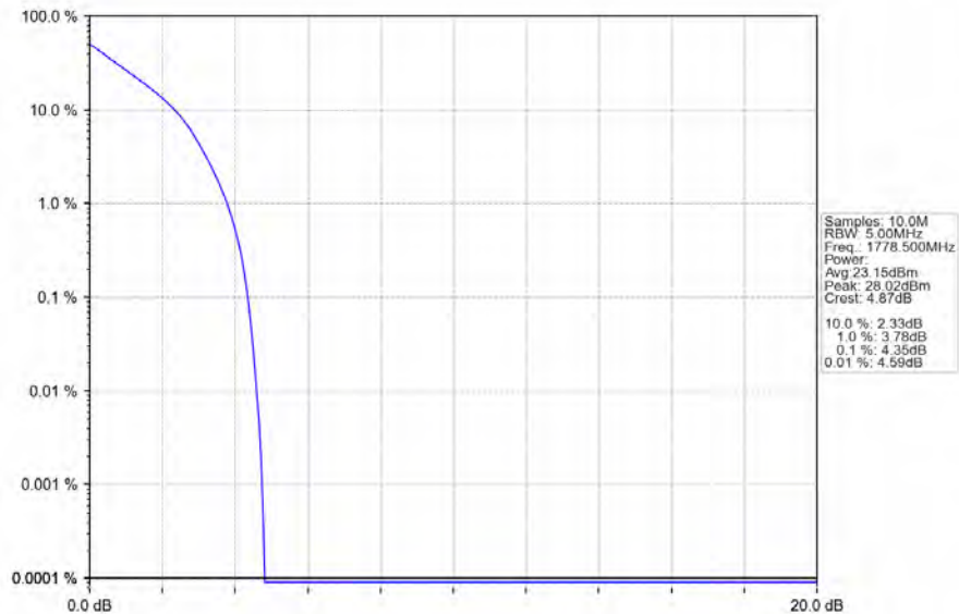
Band66_3MHz_QPSK_HCH_1778.5MHz_RB_15_0_NTNV
