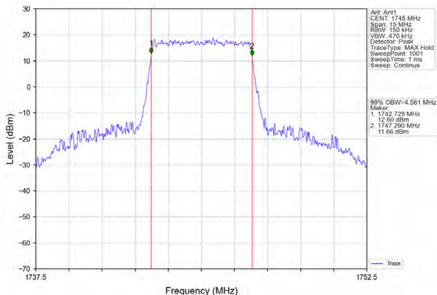
Band66_5MHz_QPSK_MCH_1745MHz_RB_25_0_NTNV
