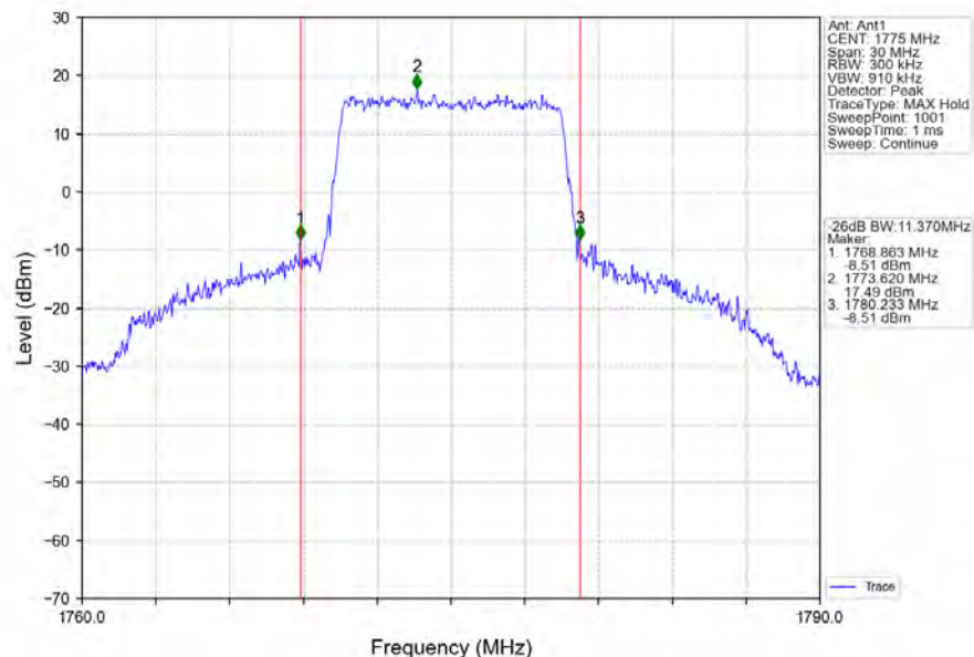
Band66_10MHz_64QAM_HCH_1775MHz_RB_50_0_NTNV
