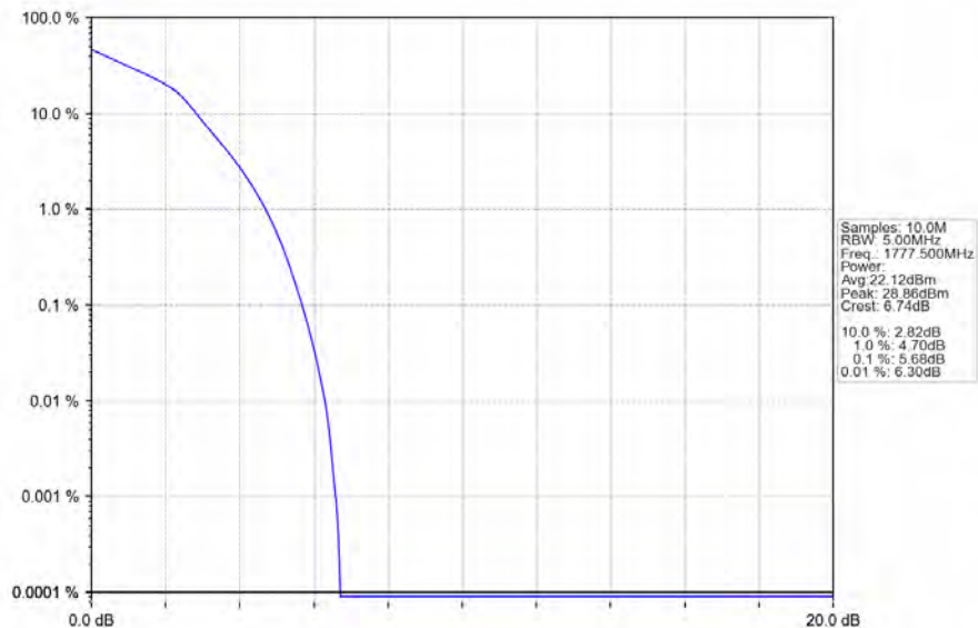
Band66_5MHz_16QAM_HCH_1777.5MHz_RB_25_0_NTNV
