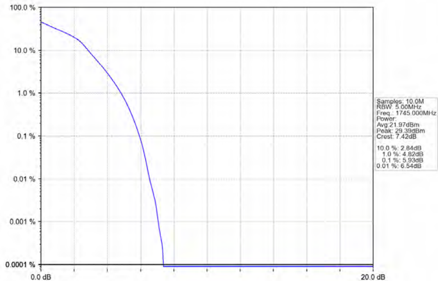
Band66_5MHz_16QAM_MCH_1745MHz_RB_25_0_NTNV
