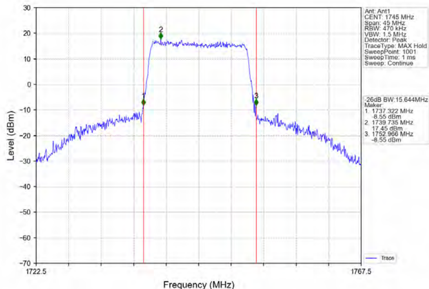
Band66_15MHz_64QAM_MCH_1745MHz_RB_75_0_NTNV
