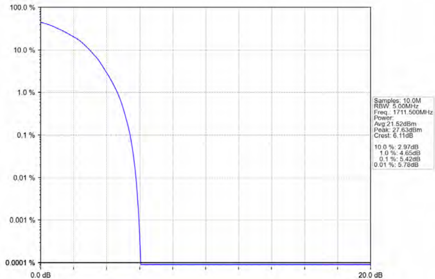
Band66_3MHz_64QAM_LCH_1711.5MHz_RB_15_0_NTNV
