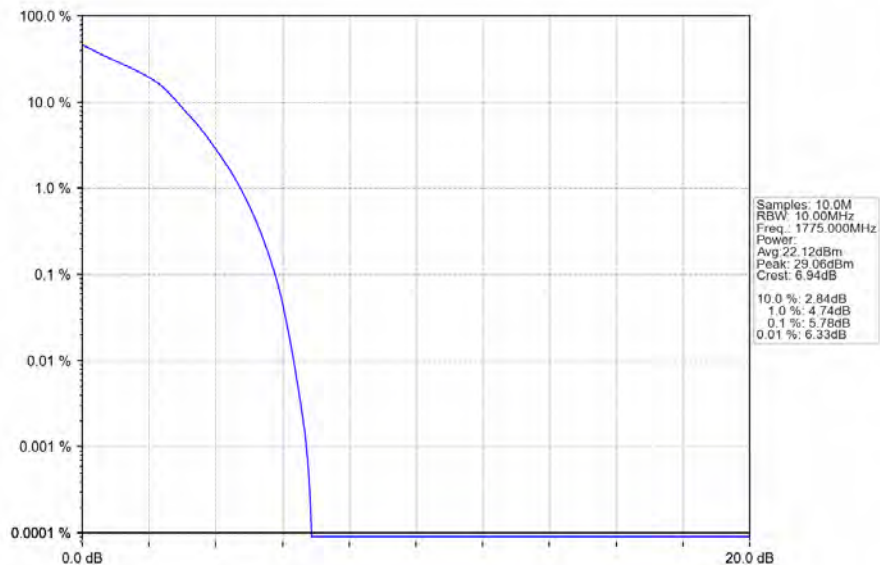
Band66_10MHz_16QAM_HCH_1775MHz_RB_50_0_NTNV
