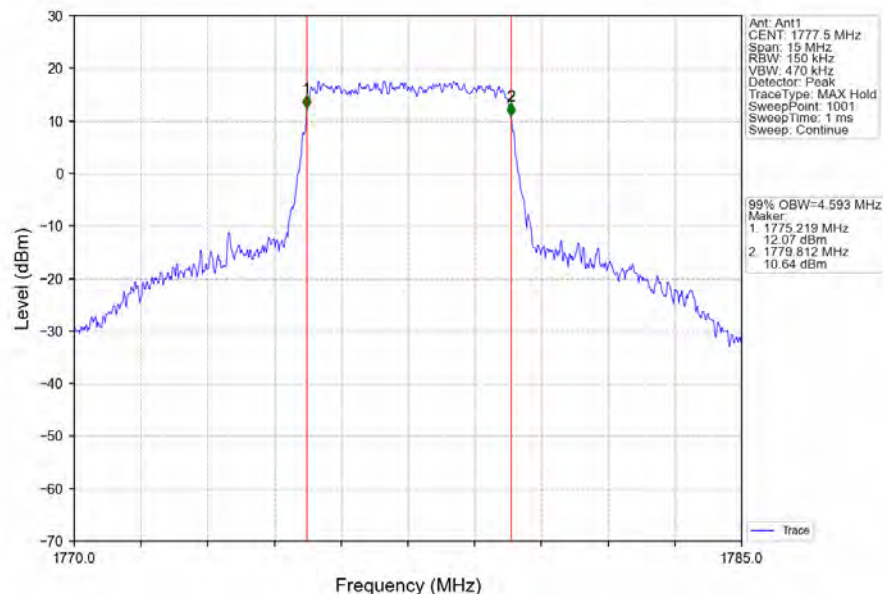
Band66_5MHz_16QAM_HCH_1777.5MHz_RB_25_0_NTNV
