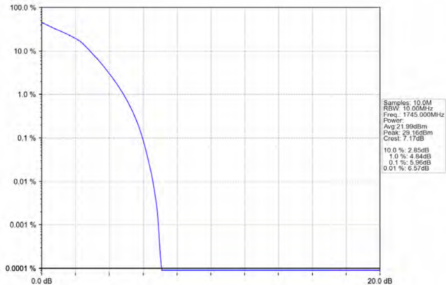
Band66_10MHz_16QAM_MCH_1745MHz_RB_50_0_NTNV
