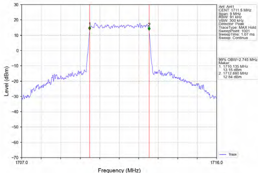
Band66_3MHz_64QAM_LCH_1711.5MHz_RB_15_0_NTNV
