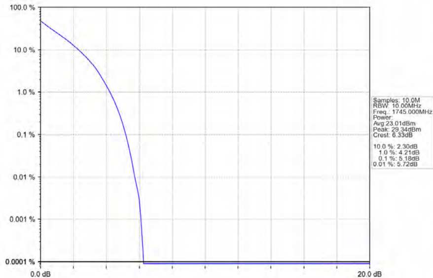
Band66_10MHz_QPSK_MCH_1745MHz_RB_50_0_NTNV
