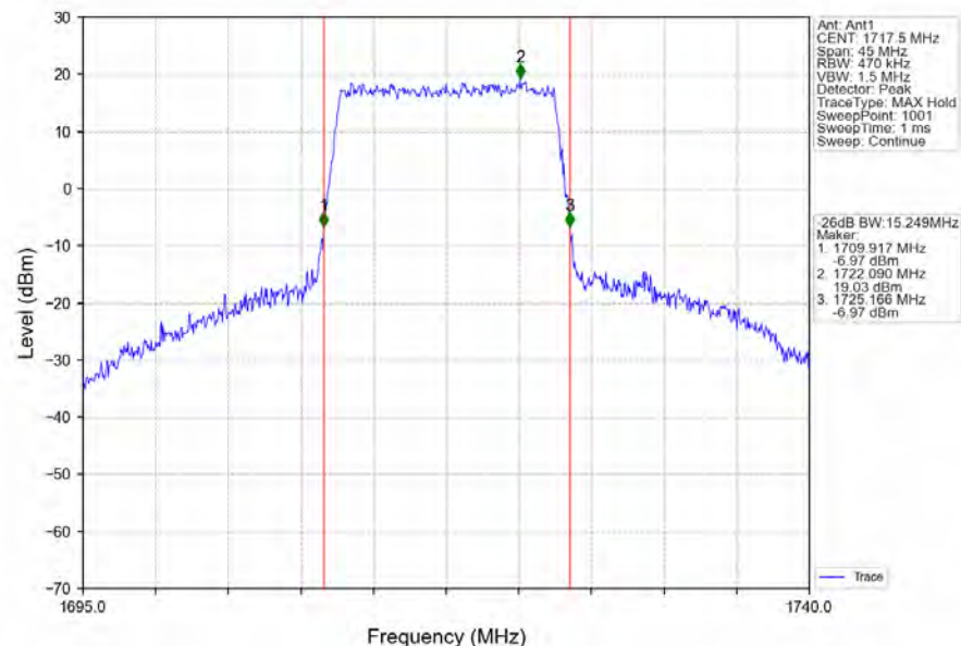
Band66_15MHz_16QAM_LCH_1717.5MHz_RB_75_0_NTNV
