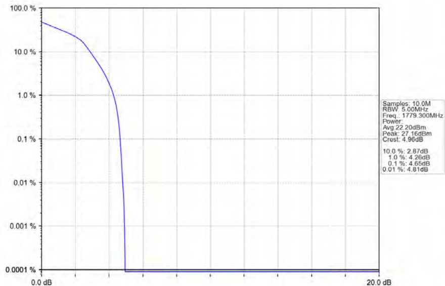
Band66_1.4MHz_16QAM_HCH_1779.3MHz_RB_6_0_NTNV
