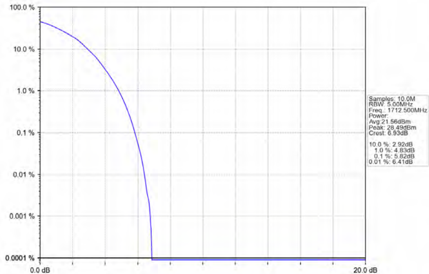
Band66_5MHz_64QAM_LCH_1712.5MHz_RB_25_0_NTNV
