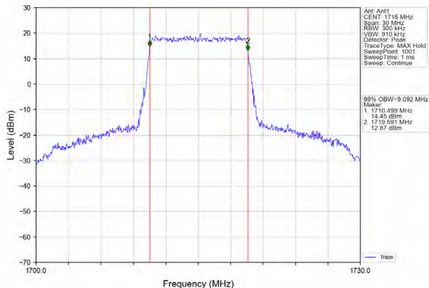
Band66_10MHz_QPSK_LCH_1715MHz_RB_50_0_NTNV
