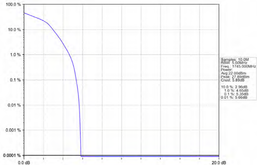
Band66_1.4MHz_16QAM_MCH_1745MHz_RB_6_0_NTNV
