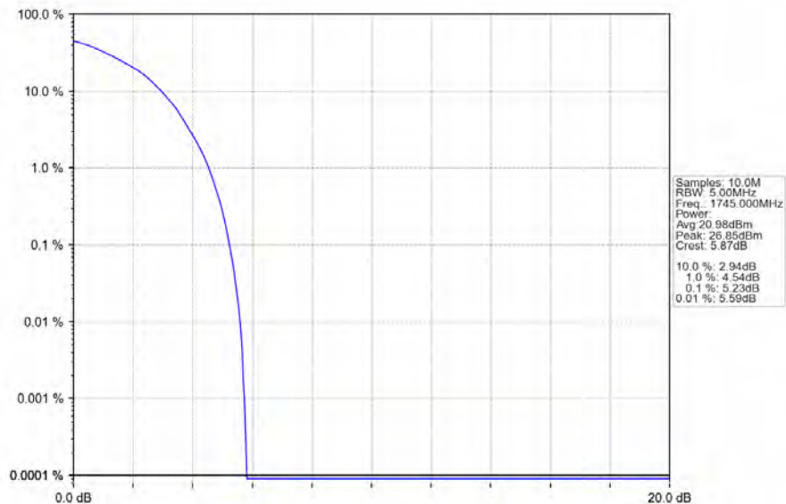
Band66_3MHz_64QAM_MCH_1745MHz_RB_15_0_NTNV
