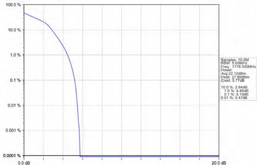
Band66_3MHz_16QAM_HCH_1778.5MHz_RB_15_0_NTNV
