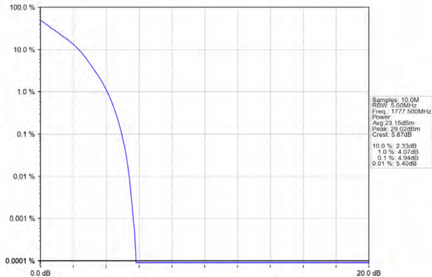
Band66_5MHz_QPSK_HCH_1777.5MHz_RB_25_0_NTNV
