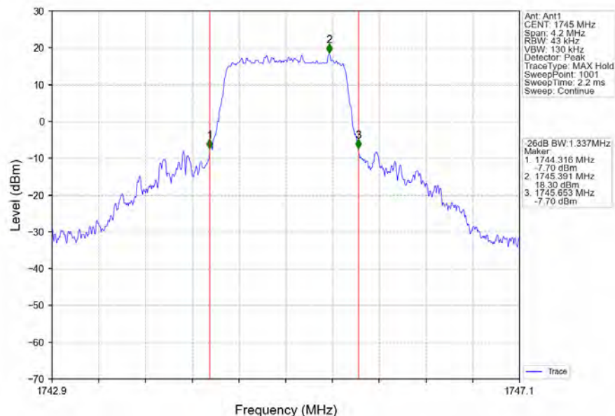
Band66_1.4MHz_64QAM_MCH_1745MHz_RB_6_0_NTNV
