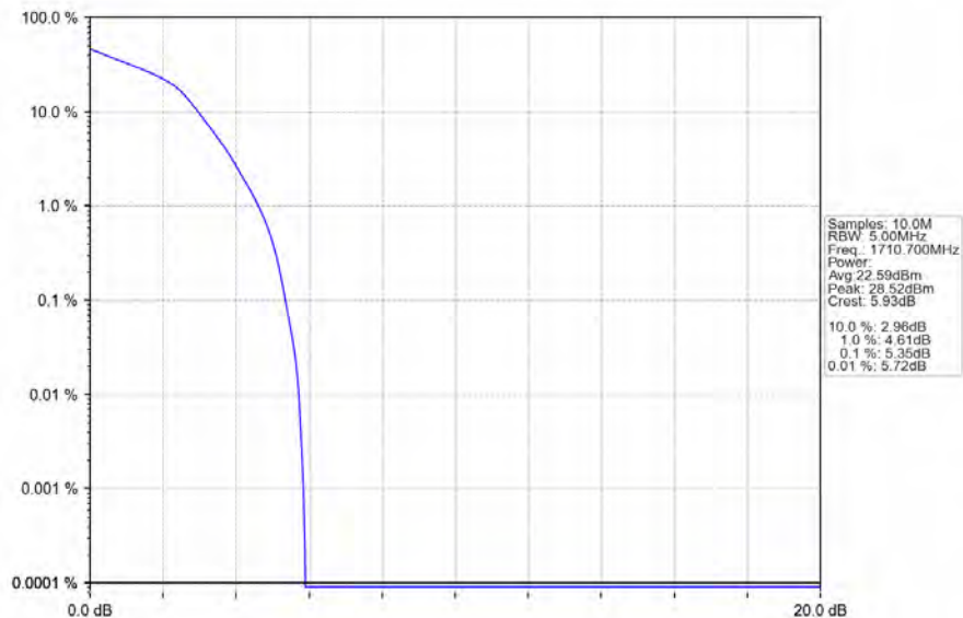
Band66_1.4MHz_16QAM_LCH_1710.7MHz_RB_6_0_NTNV
