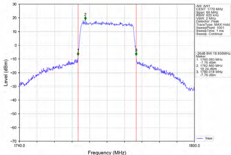
Band66_20MHz_64QAM_HCH_1770MHz_RB_100_0_NTNV
