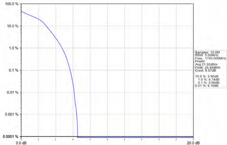
Band66_3MHz_16QAM_MCH_1745MHz_RB_15_0_NTNV
