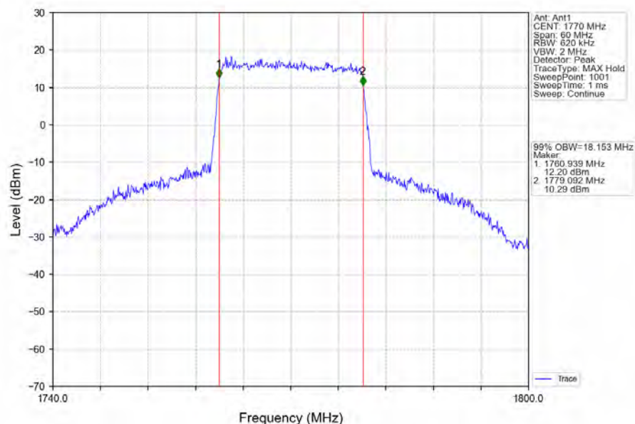
Band66_20MHz_64QAM_HCH_1770MHz_RB_100_0_NTNV
