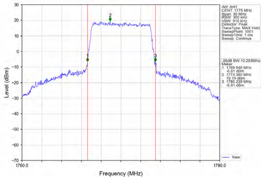
Band66_10MHz_QPSK_HCH_1775MHz_RB_50_0_NTNV
