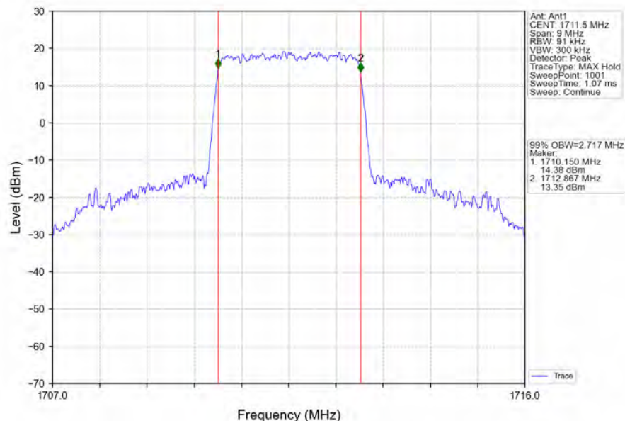
Band66_3MHz_QPSK_LCH_1711.5MHz_RB_15_0_NTNV
