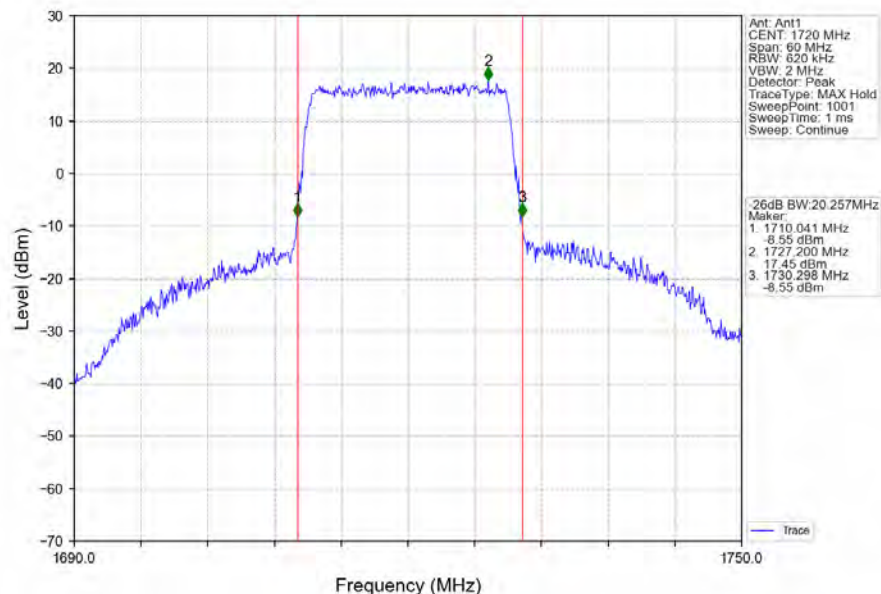
Band66_20MHz_64QAM_LCH_1720MHz_RB_100_0_NTNV
