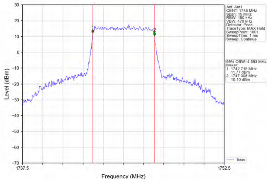
Band66_5MHz_64QAM_MCH_1745MHz_RB_25_0_NTNV
