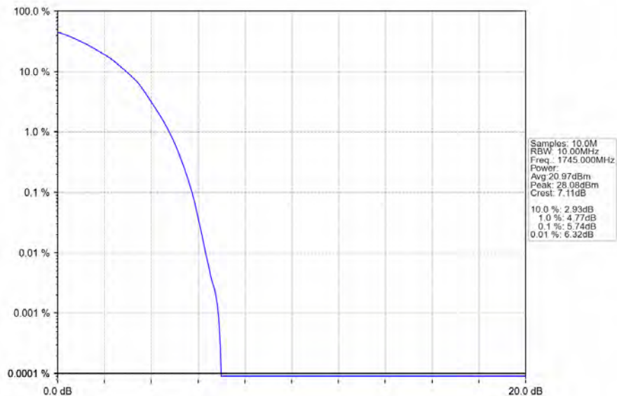
Band66_10MHz_64QAM_MCH_1745MHz_RB_50_0_NTNV
