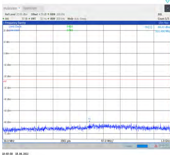
1-N2--15-20-H-1-DFT-PI2BPSK-Inner_1RB_Left-1@ 1-30-1000-Ant1--60.41--23-PASS
