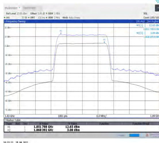
1-N2--15-20-L-2-CP-256QAM-Outer_Full-106@0-Ant 1-9.57-100%-0.00-9.57-PASS≤13
