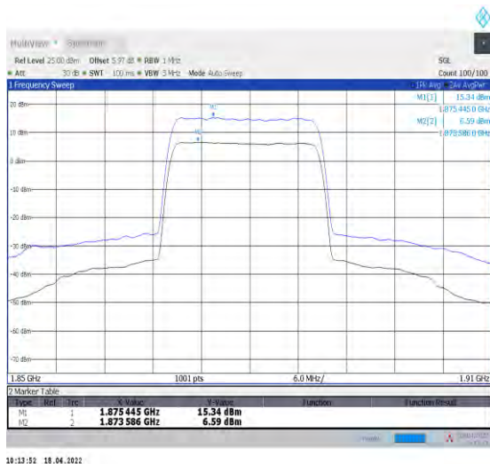
1-N2--15-20-M-1-DFT-256QAM-Outer_Full-100@0-Ant1 Ant1-8.75-100%-0.00-8.75-PASS≤13
