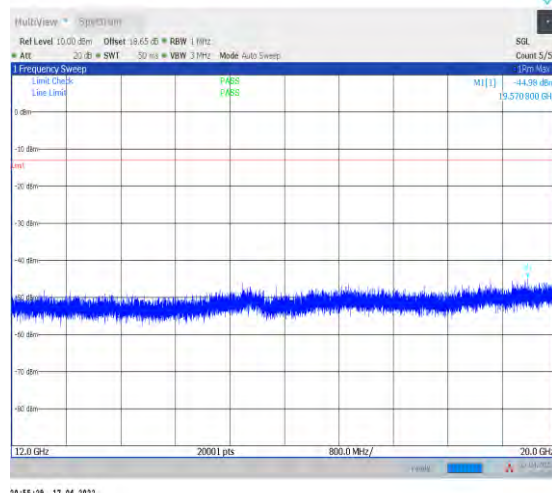
1-N2--15-20-L-1-DFT-PI2BPSK-Inner_1RB_Left-1@ 1-12000-20000-Ant1--44.98--13-PASS
