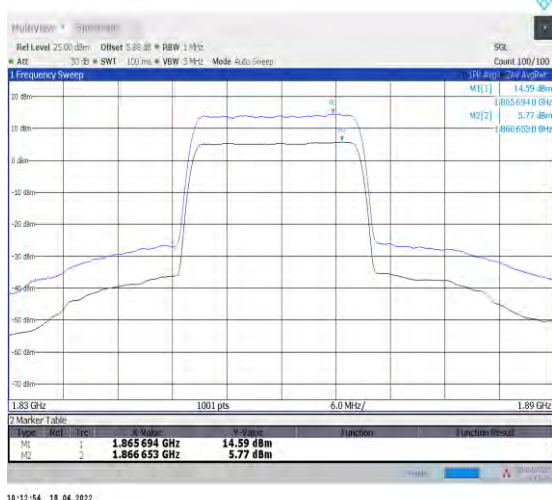
1-N2--15-20-L-1-DFT-256QAM-Outer_Full-100@0-A nt1-8.82-100%-0.00-8.82-PASS≤13
