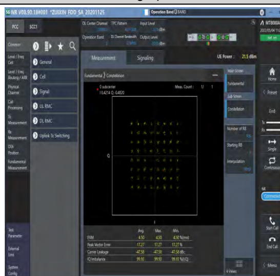
1-N2-PC3-15-20-M-8-CP-64QAM-Outer_Full-106@ 0-Ant1-see graph-PASS
