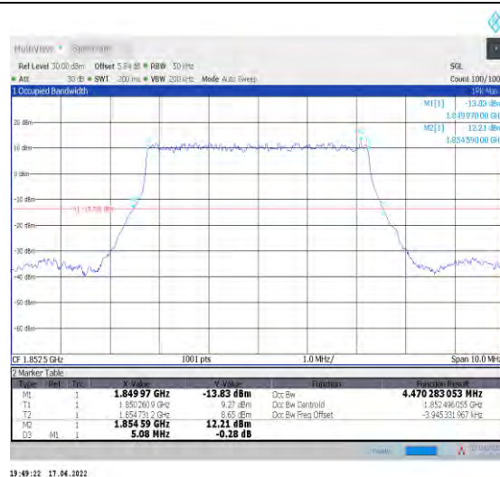
1-N2--15-5-L-2-DFT-PI2BPSK-Outer_Full-25@0-Ant 1-4.47-5.080-≤5-PASS
