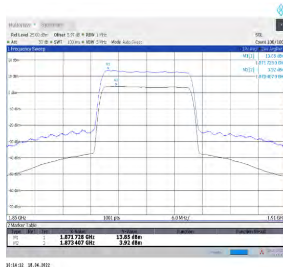
1-N2--15-20-M-2-CP-256QAM-Outer_Full-106@0-Ant t1-9.93-100%-0.00-9.93-PASS≤13
