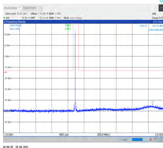
1-N2--15-20-H-1-DFT-PI2BPSK-Inner_1RB_Left-1@ 1-1000-3000-Ant1--44.57--13-PASS
