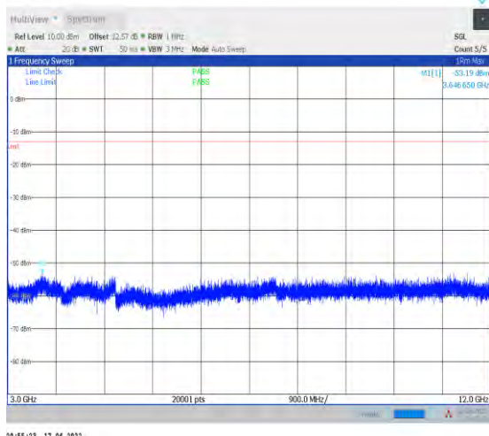
1-N2--15-20-L-1-DFT-PI2BPSK-Inner_1RB_Left-1@ 1-3000-12000-Ant1--53.19--13-PASS
