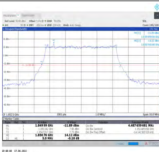
1-N2--15-5-L-1-DFT-QPSK-Outer_Full-25@0-Ant1-4 4.488-5.000-≤5-PASS
