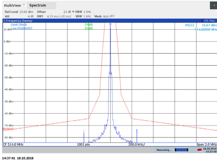
Plot 3: Unmodulated carrier reference (with pilot-tone), 514.0 MHz
