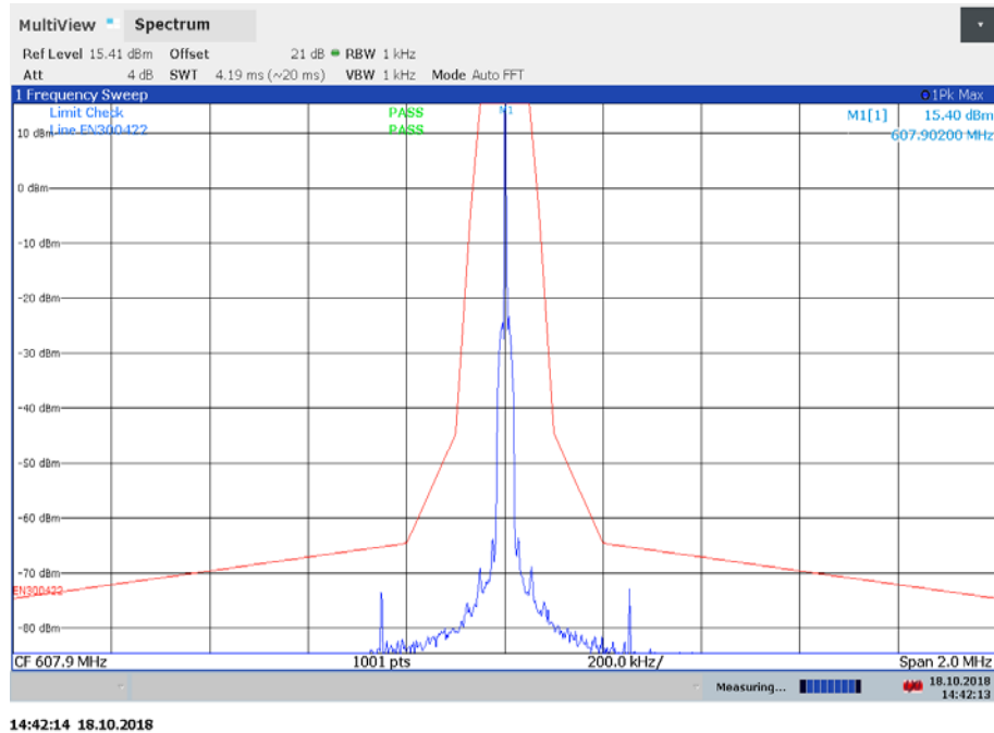
Plot 5: Unmodulated carrier reference (with pilot-tone), 607.9 MHz
