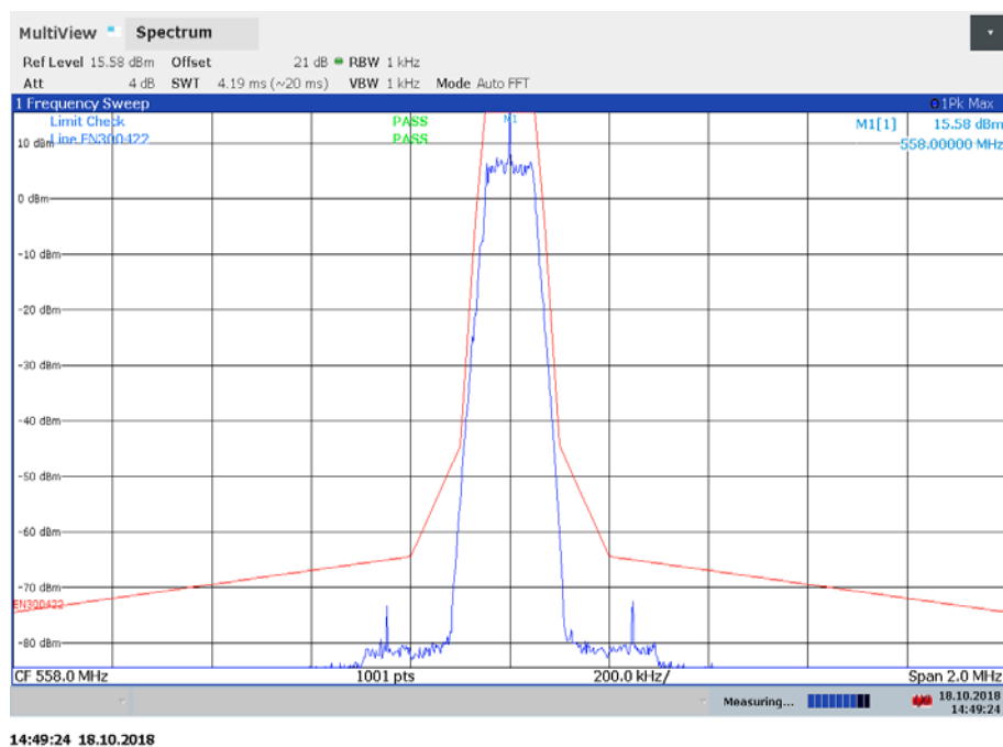
Plot 6: Modulated carrier with the weighted noise source, 558 MHz
