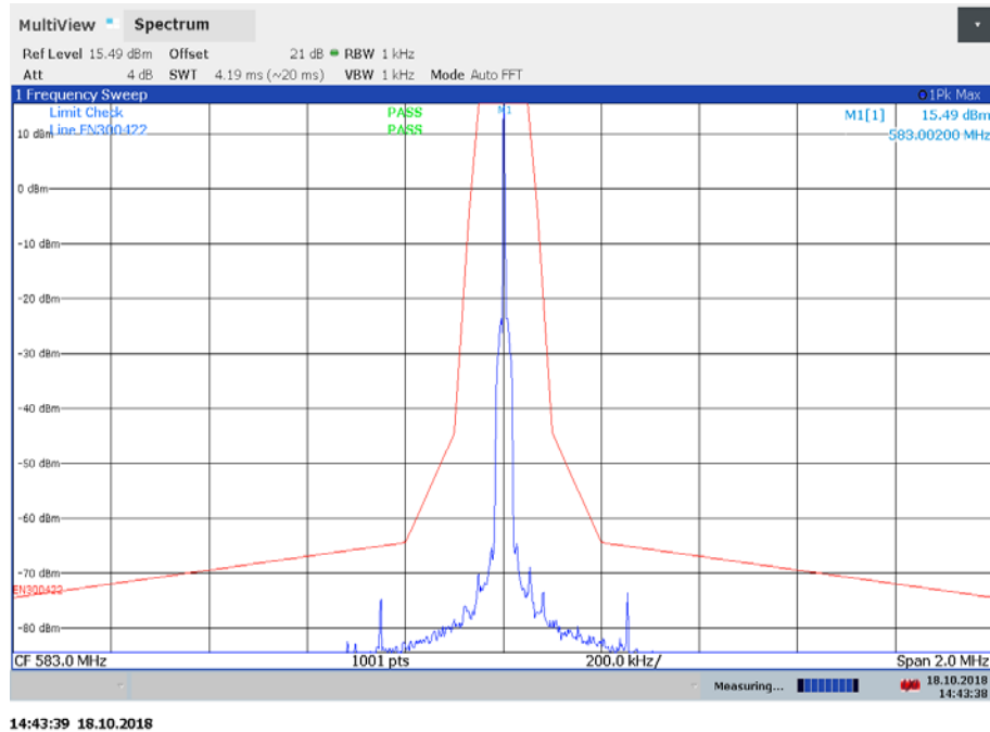
Plot 3: Unmodulated carrier reference (with pilot-tone), 583.0 MHz
