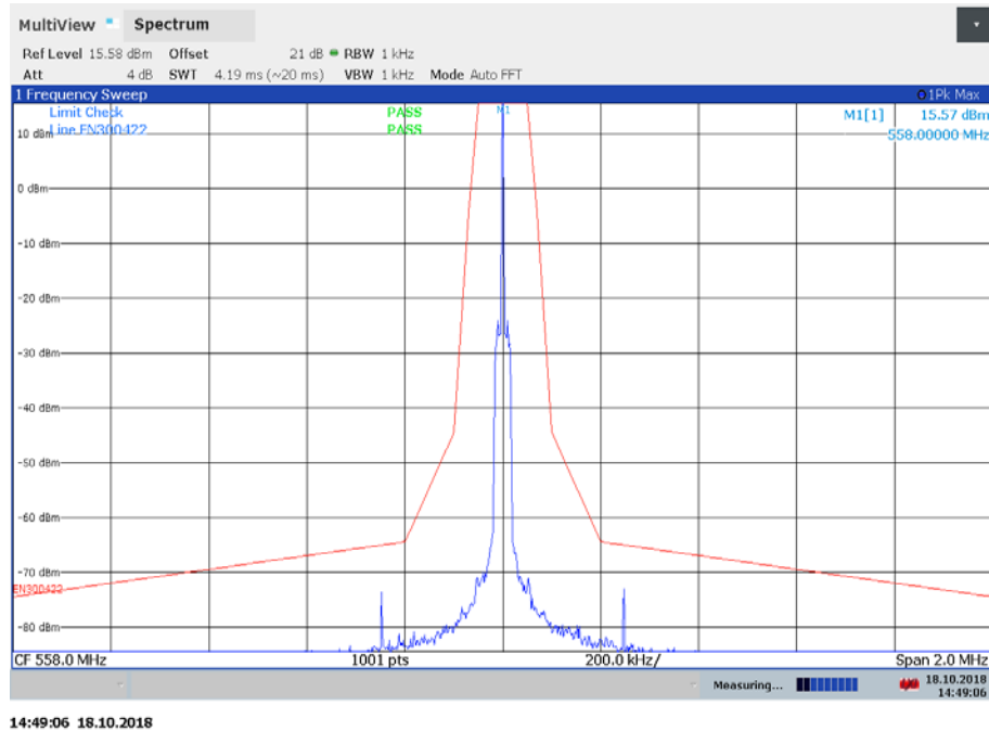
Plot 5: Unmodulated carrier reference (with pilot-tone), 558.0 MHz
