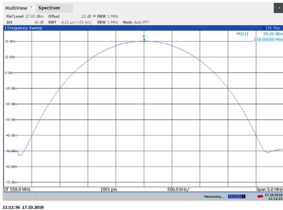
Plot 6: 558 MHz, peak (unmodulated carrier)
