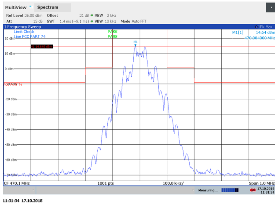
Plot 1: 470.1 MHz, spectrum mask
