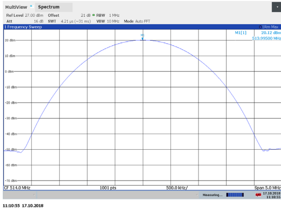
Plot 3: 514 MHz, average (modulated carrier)
