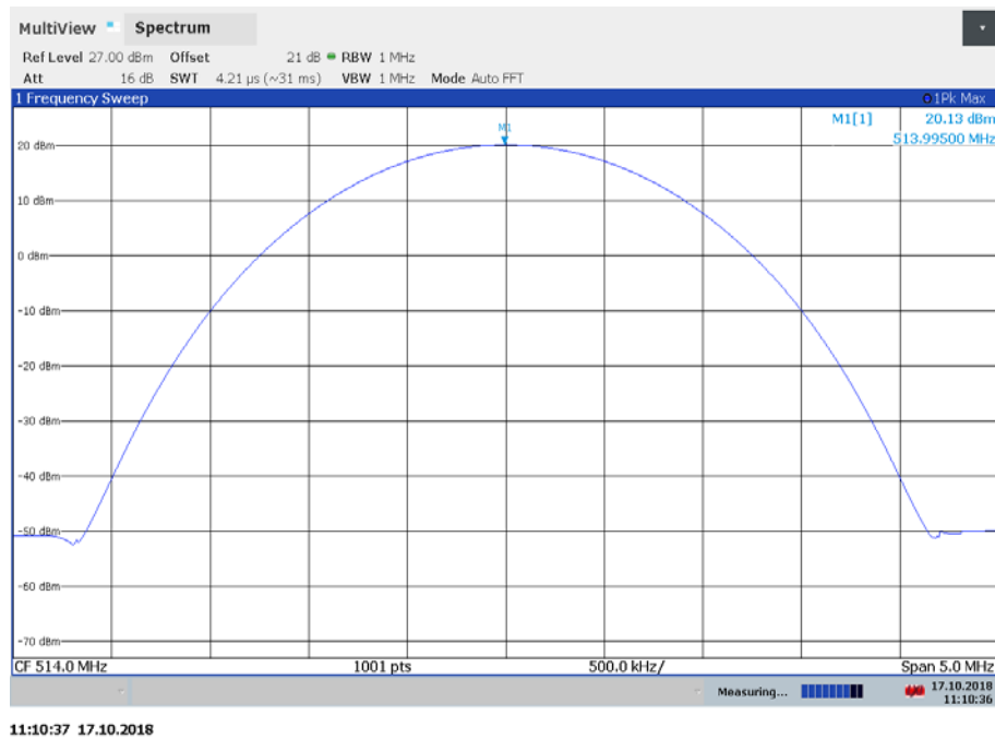
Plot 4: 514 MHz, peak (unmodulated carrier)
