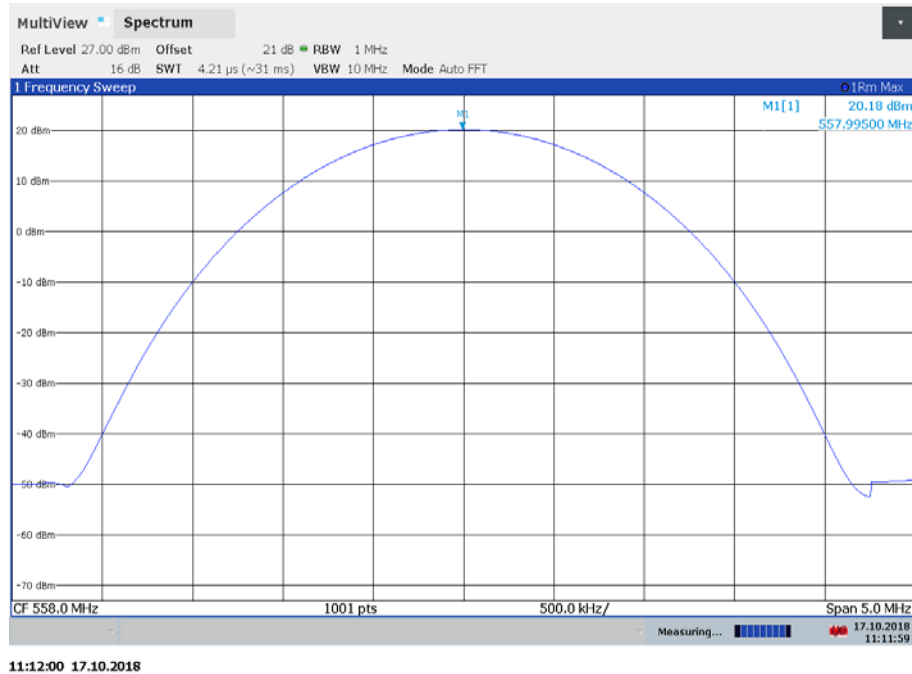
Plot 5: 558 MHz, average (modulated carrier)
