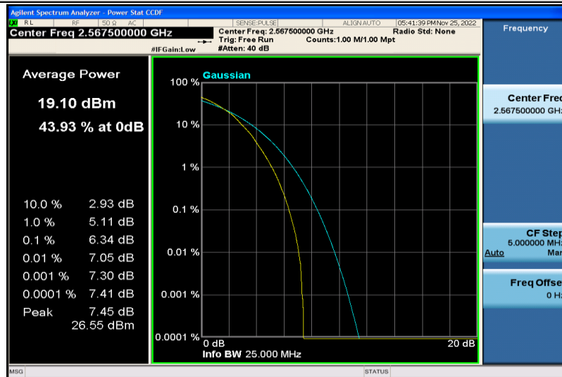
Band7-5MHz-64QAM-21425-25RB#0
