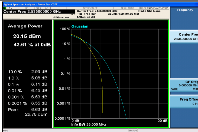
Band7-10MHz-64QAM-21100-1RB#0
