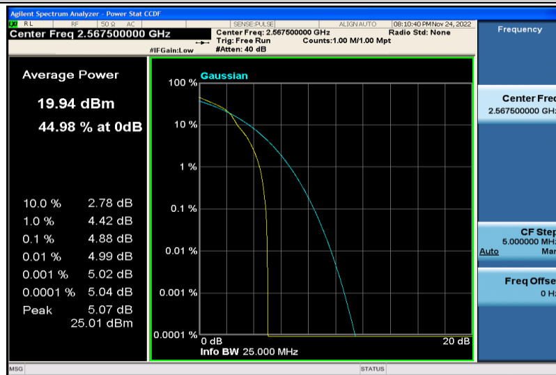
Band7-5MHz-16QAM-21425-1RB#0
