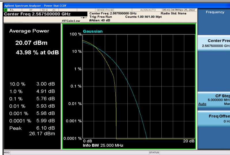
Band7-5MHz-64QAM-21425-1RB#0
