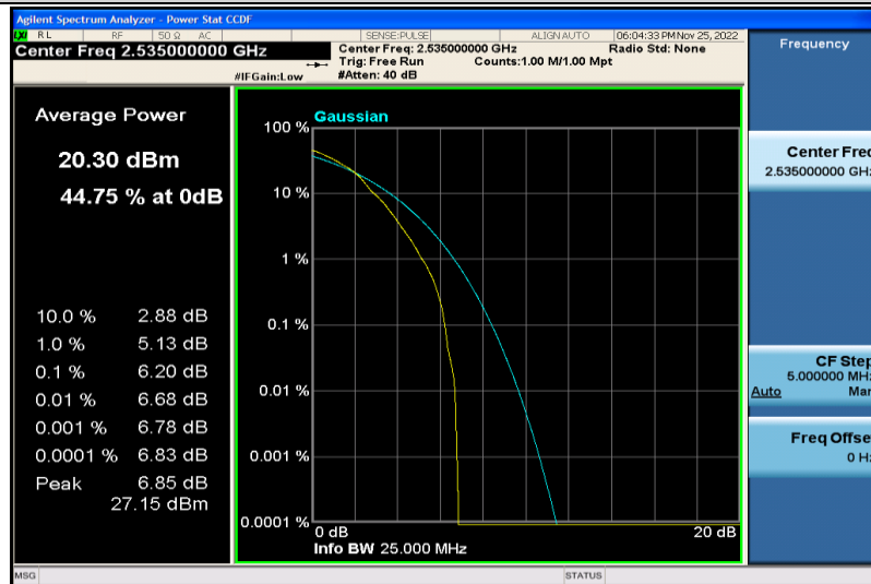
Band7-15MHz-64QAM-21100-1RB#0
