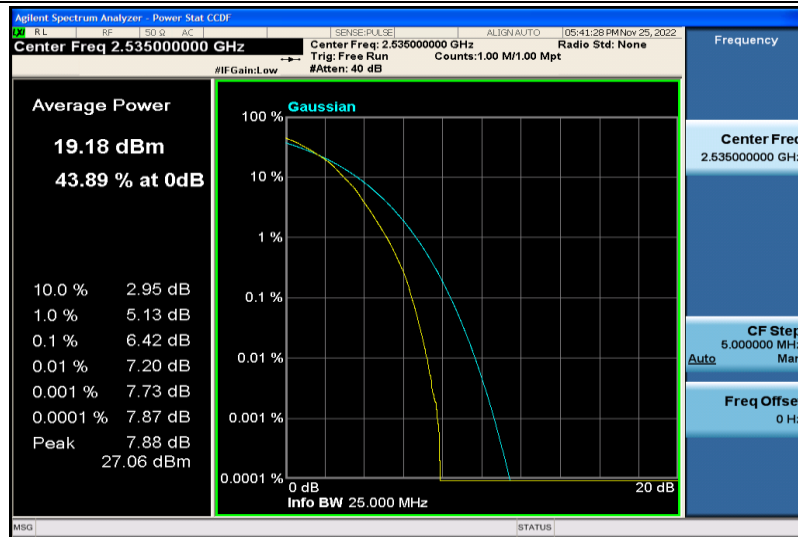
Band7-5MHz-64QAM-21100-25RB#0
