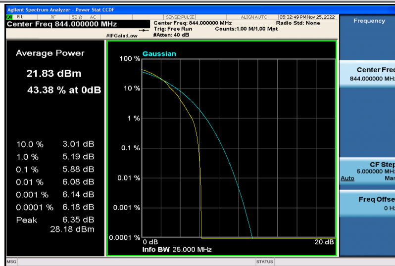
Band5-10MHz-64QAM-20600-1RB#0
