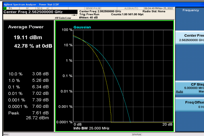
Band7-15MHz-64QAM-21375-75RB#0
