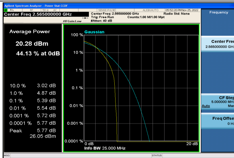
Band7-10MHz-64QAM-21400-1RB#0
