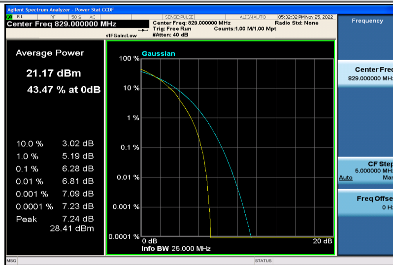
Band5-10MHz-64QAM-20450-50RB#0
