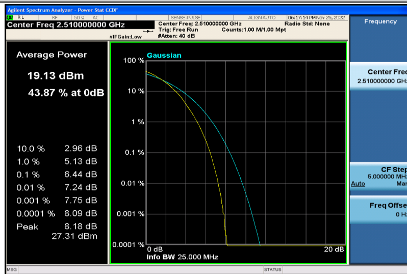
Band7-20MHz-64QAM-20850-100RB#0
