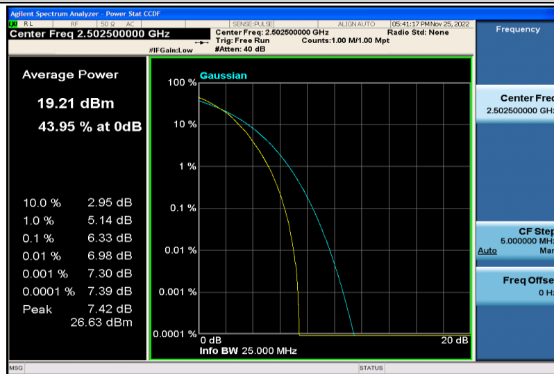
Band7-5MHz-64QAM-20775-25RB#0
