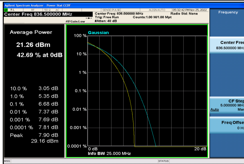
Band5-10MHz-64QAM-20525-50RB#0
