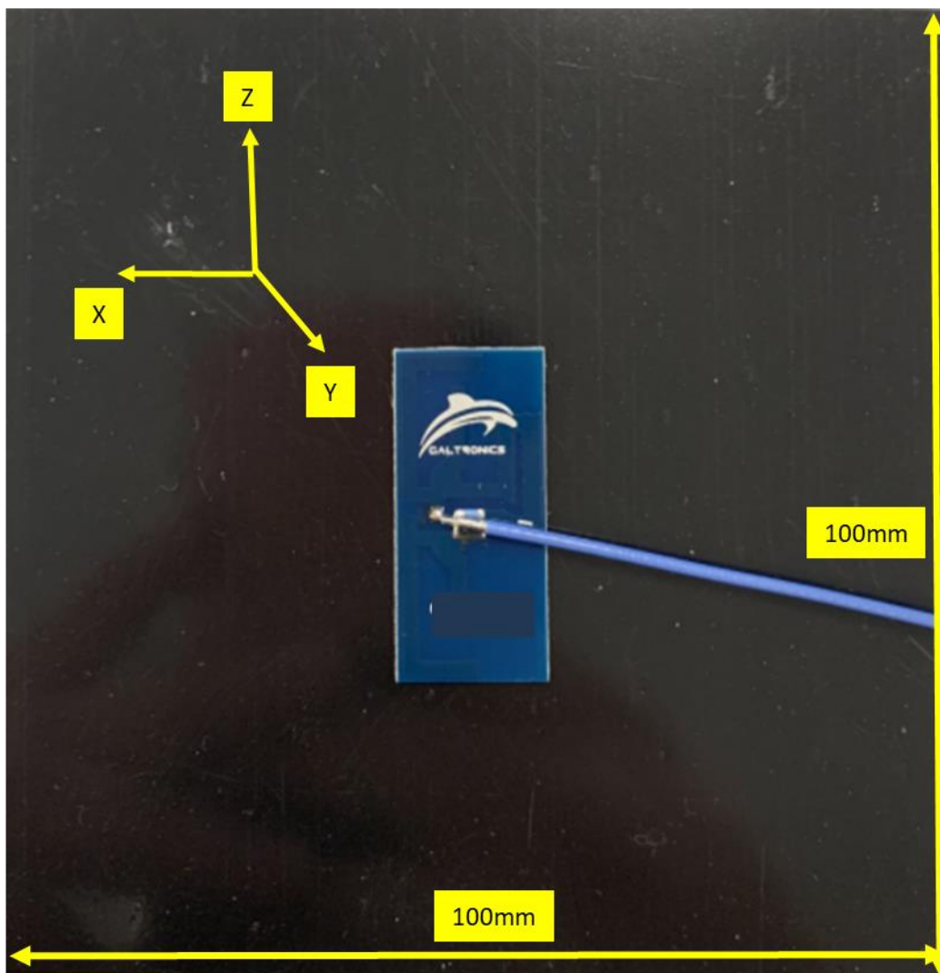
Figure 3 Measurement Orientation
