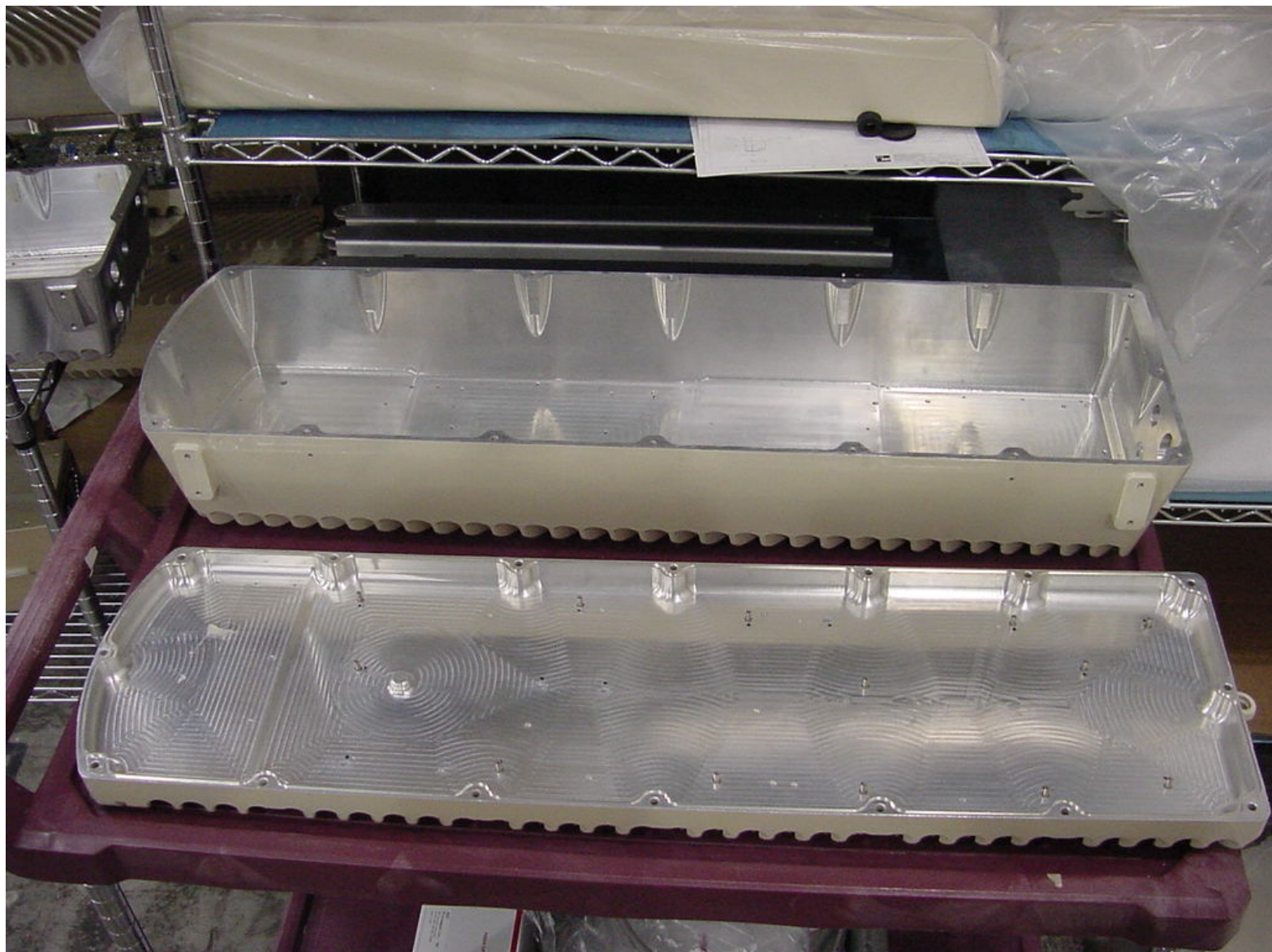
Digivance Street Coverage Solution Remote Unit Open Top View 2
