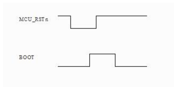
Figure 2 . 3 Timing diagram for entering burn-in mode
