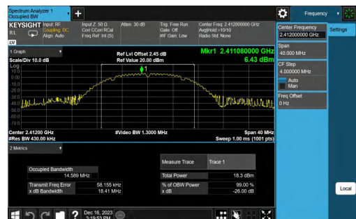
11B-CDD-Ant2-2412
