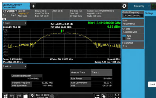
11B-CDD-Ant1-2412
