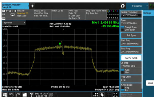
11N40SISO-Ant1-2437-PASS
