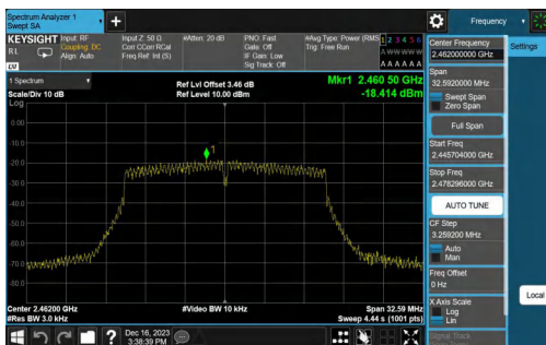
11G-CDD-Ant1-2462-PASS
