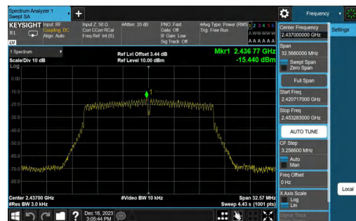
11G-Ant2-2437-PASS
