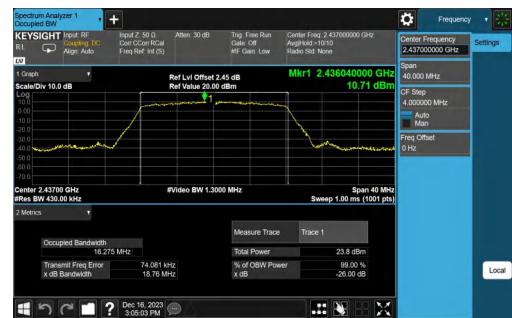
11G-Ant2-2437
