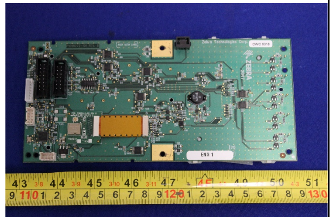
LCD board – Bottom view
