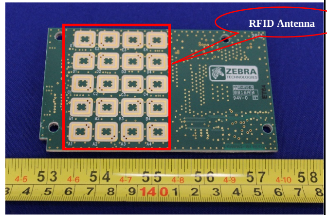
UHF RFID Board – Bottom view
