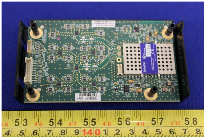
UHF RFID Board – Top view
