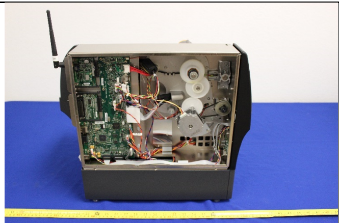
EUT - Cover off-2
