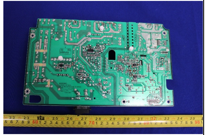
Power Board - Bottom view
