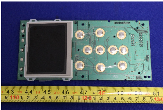
LCD board – Top view
