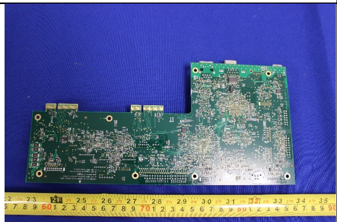
Main Board - bottom view
