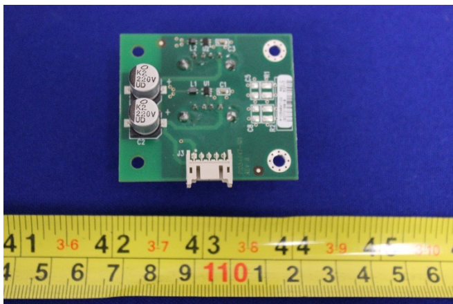
USB board - Top view
