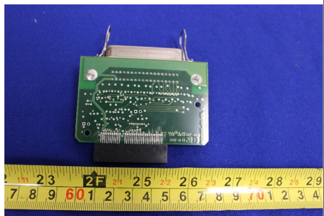
Parallel Board - Bottom view
