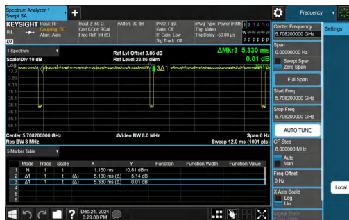
NTNV-11AX20SISO-Ant1-5700-106Tone-RU54
