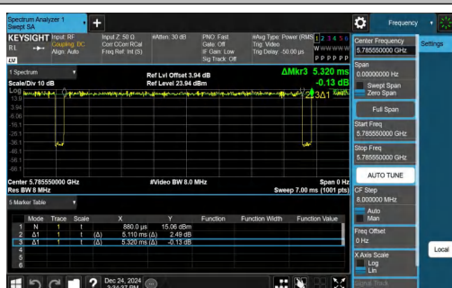
NTNV-11AX20SISO-Ant1-5785-106Tone-RU53
