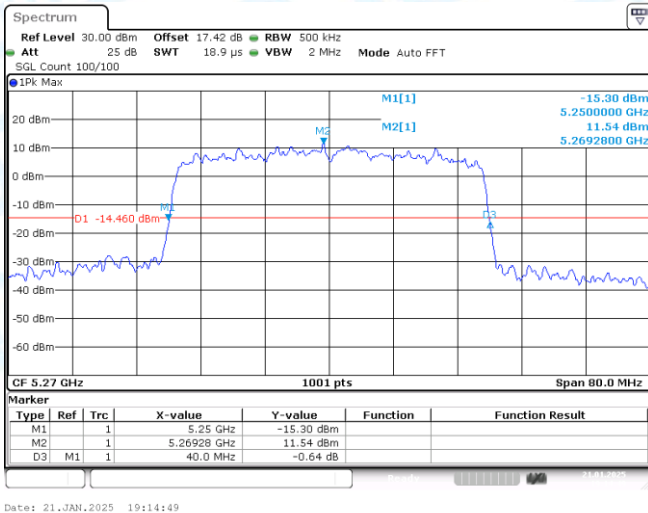
11AX40-CDD-Ant1-5270
