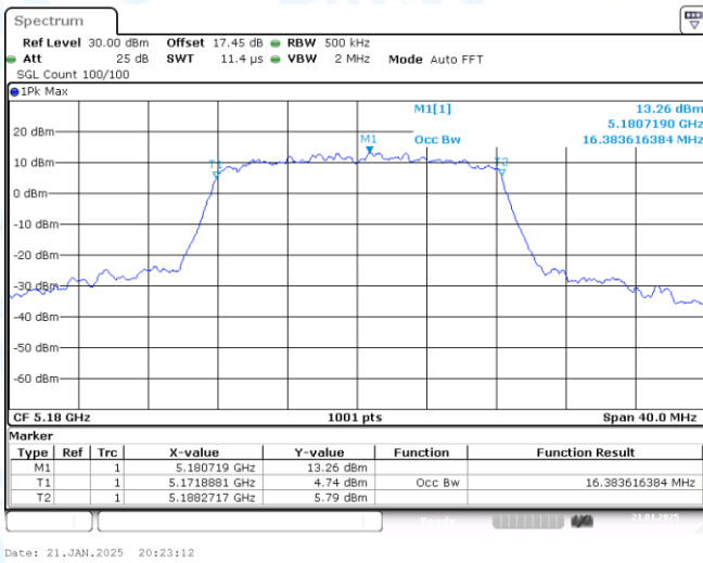
11A-CDD-Ant1-5180
