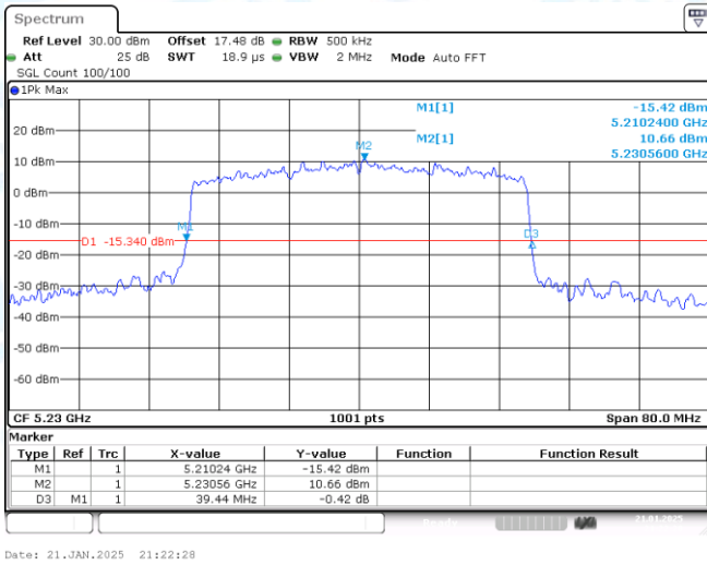
11AX40-CDD-Ant1-5230
