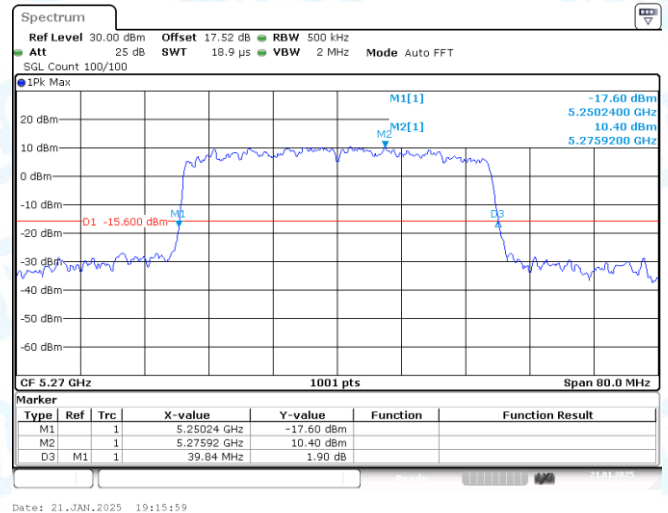
11AX40-CDD-Ant2-5270
