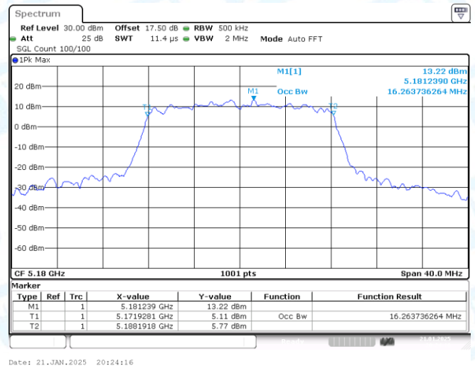
11A-CDD-Ant2-5180
