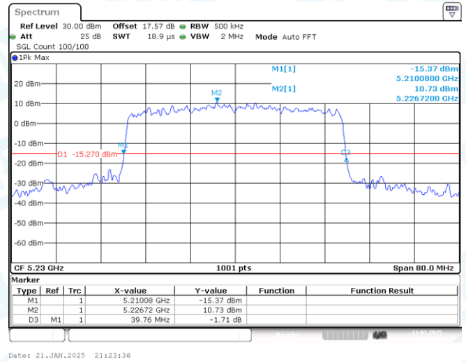
11AX40-CDD-Ant2-5230
