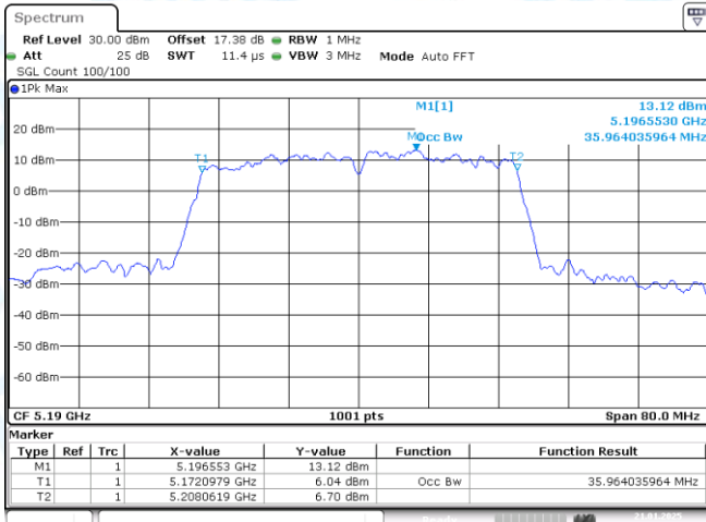
11N40-CDD-Ant1-5190
