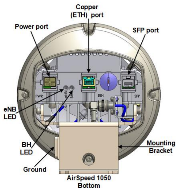
Figure 4: AirSpeed 1050 Bottom
