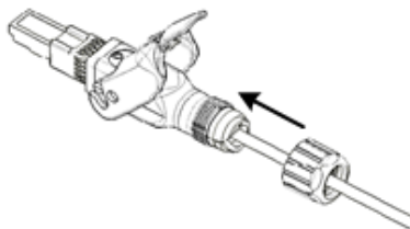
Figure 53: Insert Cone
