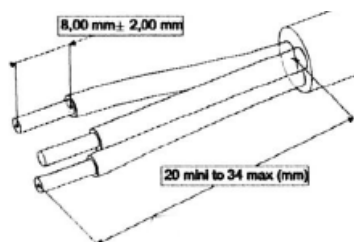
Figure 12: Stripping Dimensions (AC Cable)
