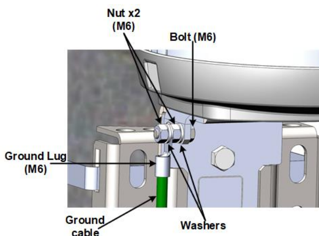
Figure 11: Ground Connection
