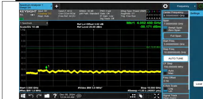
Band26(814-824)-5MHz-QPSK-26715-1RB#0-3000~10000-PASS
