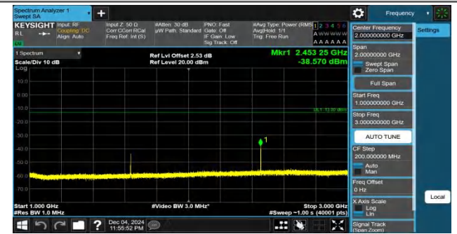
Band26(814-824)-3MHz-QPSK-26740-1RB#0-1000~3000-PASS
