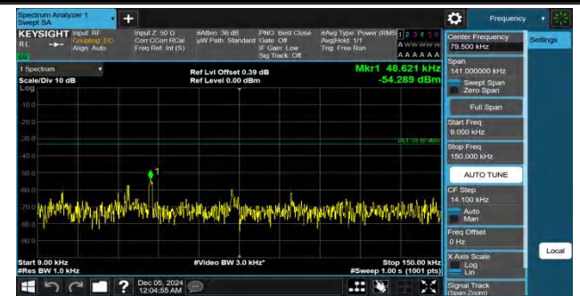
Band26(814-824)-5MHz-QPSK-26715-1RB#24-0.009~0.15-PASS
