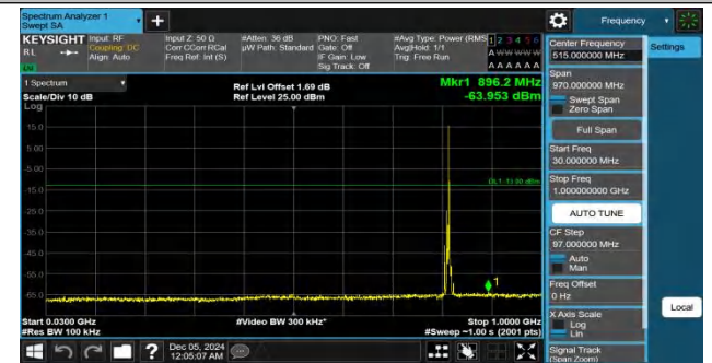
Band26(814-824)-5MHz-QPSK-26715-1RB#24-30~1000-PASS
