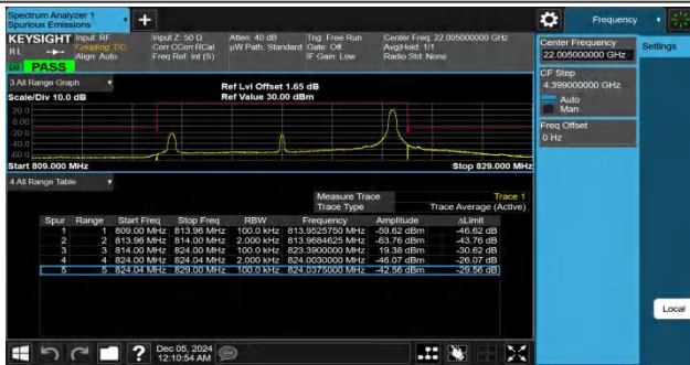
Band26(814-824)-10MHz-QPSK-26740-1RB#49-PASS
