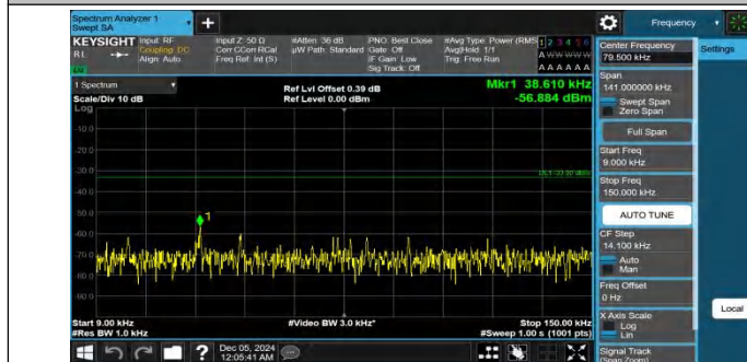
Band26(814-824)-5MHz-QPSK-26740-1RB#0-0.009~0.15-PASS
