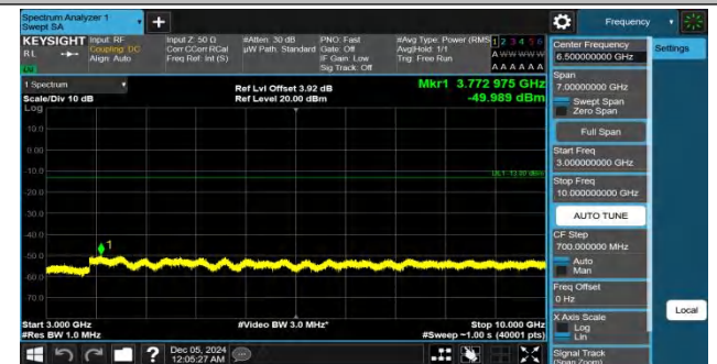
Band26(814-824)-5MHz-QPSK-26715-1RB#24-3000~10000-PASS
